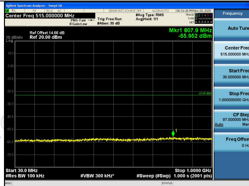
Band2-5MHz-16QAM-18900-1RB#0-30~1000-PA
