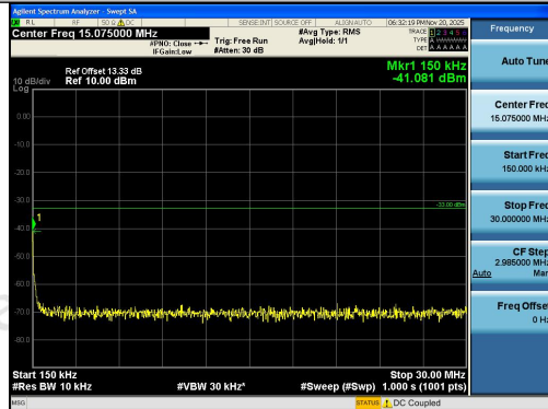
Band2-5MHz-QPSK-18900-1RB#24-0.15~30-PAS
