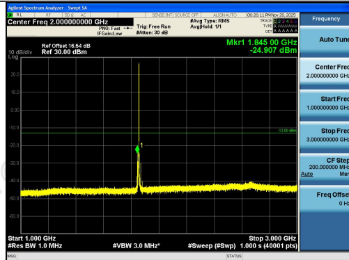
Band2-5MHz-QPSK-18625-1RB#24-1000~3000-P
