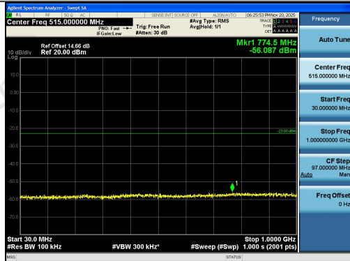
Band2-5MHz-QPSK-18625-1RB#24-30~1000-PA
