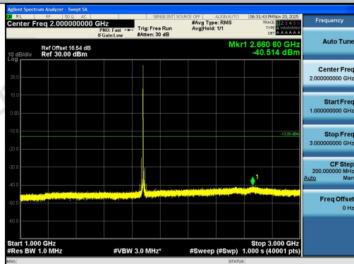
Band2-5MHz-16QAM-18900-1RB#0-1000~3000-P
