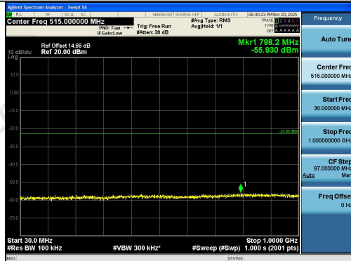
Band2-5MHz-QPSK-18900-1RB#0-30~1000-PAS
