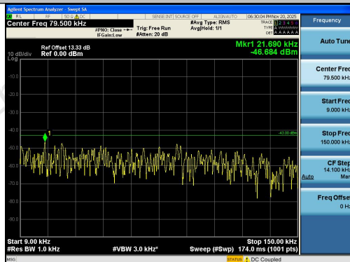
Band2-5MHz-QPSK-18900-1RB#0-0.009~0.15-PA
