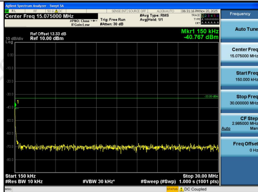
Band2-5MHz-16QAM-18900-1RB#0-0.15~30-PAS
