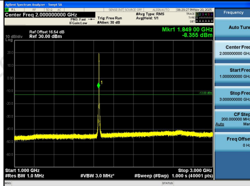
Band2-5MHz-16QAM-18625-25RB#0-1000~3000-
