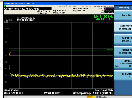
Band2-5MHz-QPSK-18900-1RB#0-0.15~30-PASS
