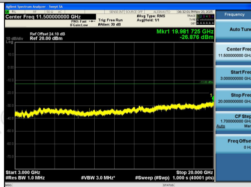
Band2-5MHz-16QAM-18900-1RB#0-3000~20000-PASS
