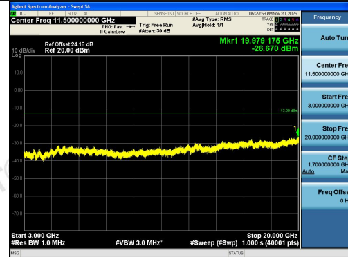
Band2-5MHz-16QAM-18625-25RB#0-3000~2000
