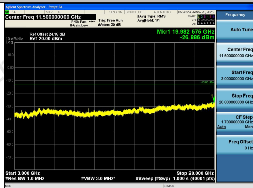
Band2-5MHz-QPSK-18625-1RB#24-3000~20000-PASS
