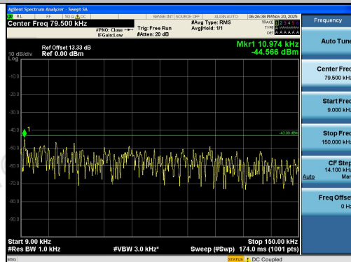
Band2-5MHz-16QAM-18625-1RB#24-0.009~0.15-PASS
