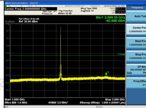
Band2-5MHz-QPSK-18900-1RB#0-1000~3000-PA
