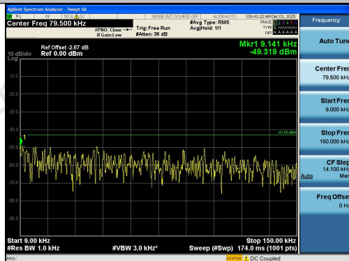
Band2-10MHz-16QAM-18650-1RB#0-0.009~0.15-PASS
