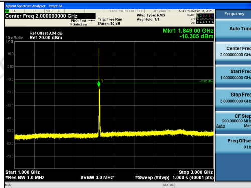
Band2-10MHz-QPSK-18650-1RB#0-1000~3000-P
