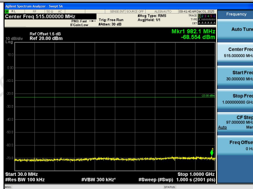
Band2-10MHz-16QAM-18650-1RB#0-30~1000-PA
