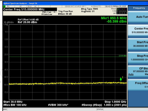
Band2-5MHz-16QAM-19175-25RB#0-30~1000-PA
