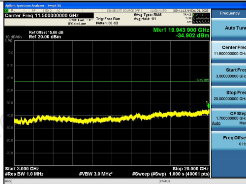
Band2-10MHz-QPSK-18650-1RB#0-3000~20000-PASS
