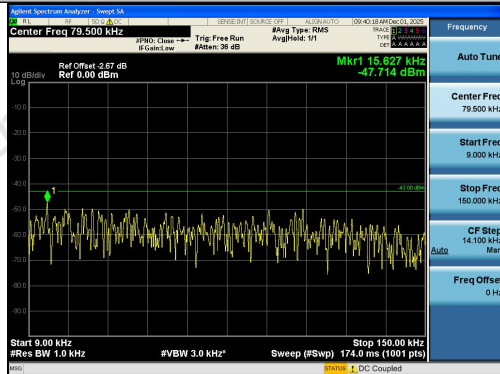
Band2-10MHz-QPSK-18650-1RB#0-0.009~0.15-P
