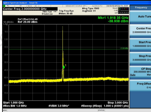
Band2-10MHz-QPSK-19150-1RB#0-1000~3000-P
