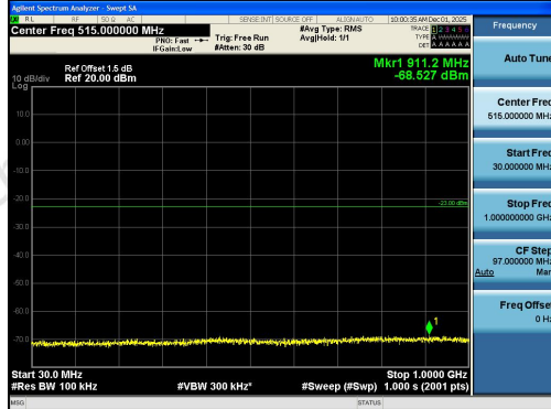
Band2-10MHz-16QAM-19150-1RB#0-30~1000-PA
