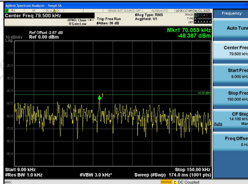
Band2-10MHz-16QAM-19150-1RB#0-0.009~0.15-PASS
