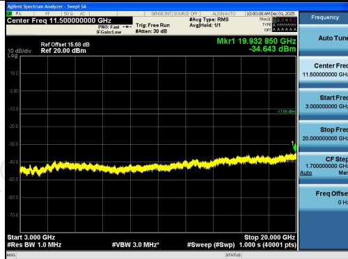
Band2-10MHz-QPSK-19150-1RB#0-3000~20000-PASS
