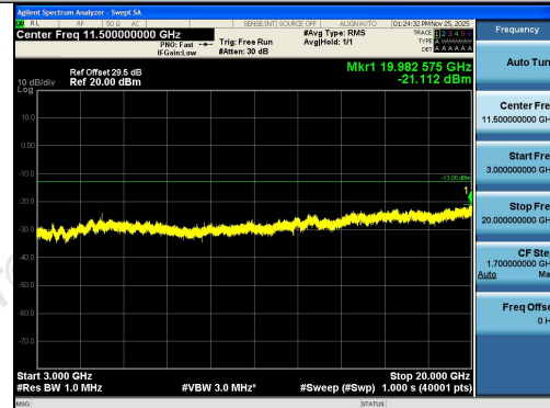
Band2-20MHz-16QAM-18700-1RB#0-3000~2000
