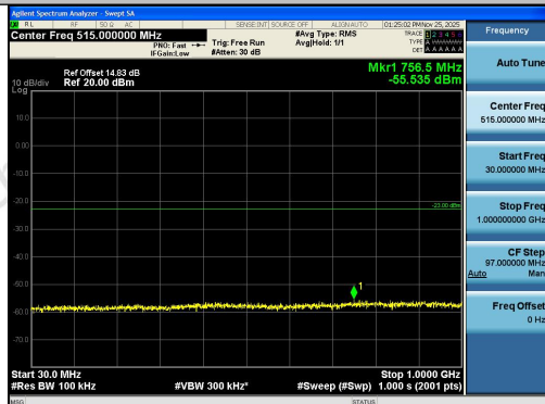
Band2-20MHz-QPSK-18700-1RB#99-30~1000-PA
