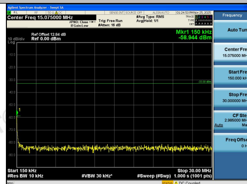
Band2-20MHz-QPSK-18700-1RB#99-0.15~30-PA
