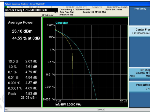
Band4-3MHz-QPSK-20175-1RB#0-PASS
