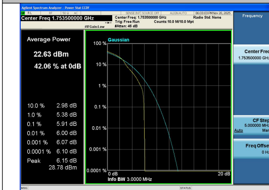
Band4-3MHz-16QAM-20385-1RB#0-PASS
