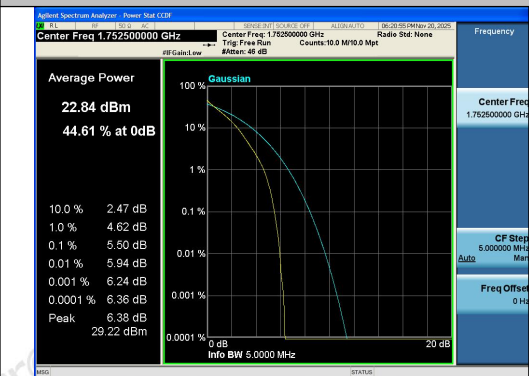
Band4-5MHz-QPSK-20375-25RB#0-PASS
