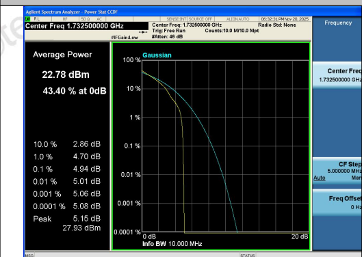
Band4-10MHz-QPSK-20175-1RB#0-PASS
