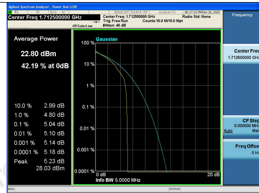
Band4-5MHz-QPSK-19975-1RB#0-PASS
