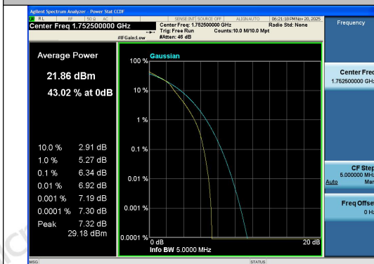
Band4-5MHz-16QAM-20375-25RB#0-PASS
