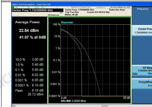
Band4-1.4MHz-16QAM-20393-1RB#0-PASS
