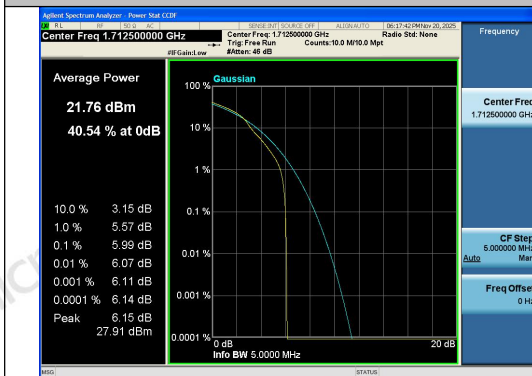
Band4-5MHz-16QAM-19975-1RB#0-PASS
