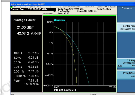
Band4-3MHz-16QAM-20175-15RB#0-PASS
