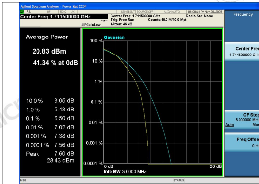
Band4-3MHz-16QAM-19965-15RB#0-PASS
