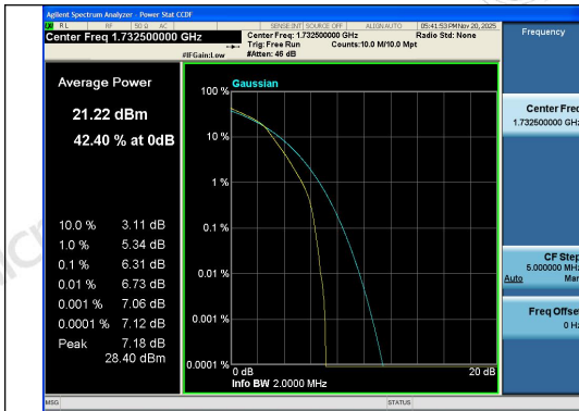
Band4-1.4MHz-16QAM-20175-6RB#0-PASS
