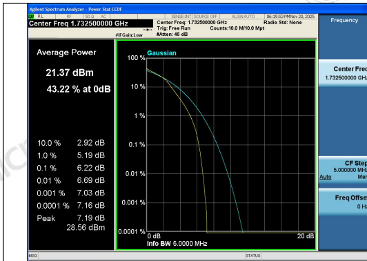
Band4-5MHz-16QAM-20175-25RB#0-PASS
