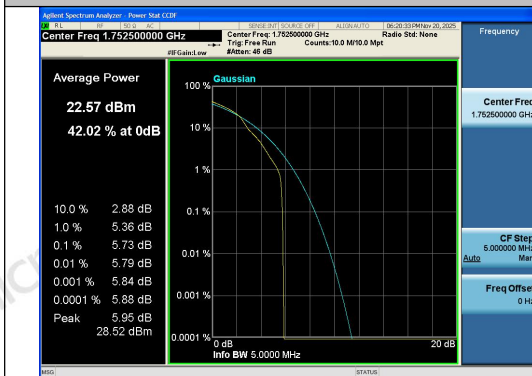
Band4-5MHz-16QAM-20375-1RB#0-PASS
