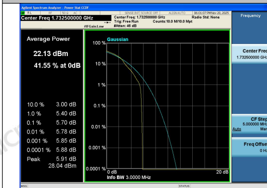
Band4-3MHz-16QAM-20175-1RB#0-PASS
