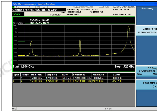
Band4-15MHz-QPSK-20025-1RB#74-PASS
