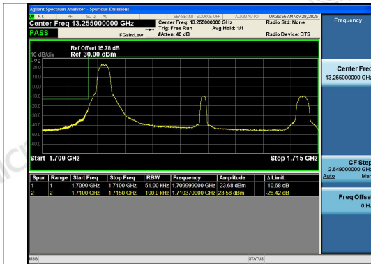
Band4-5MHz-QPSK-19975-1RB#0-PASS
