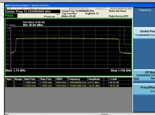
Band4-15MHz-QPSK-20325-75RB#0-PASS
