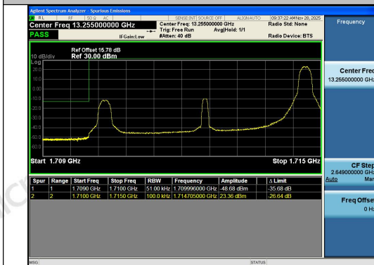
Band4-5MHz-QPSK-19975-1RB#24-PASS
