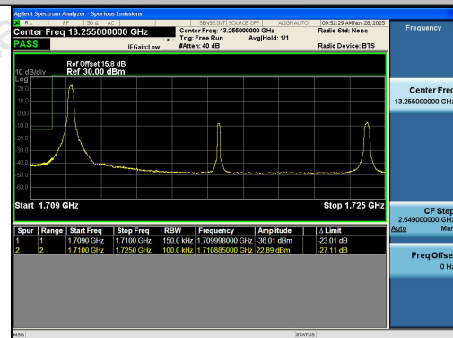
Band4-15MHz-16QAM-20025-1RB#0-PASS
