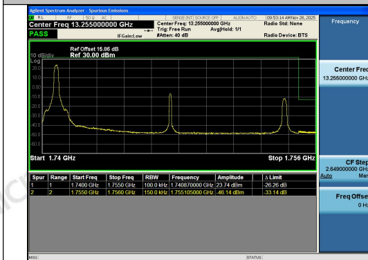
Band4-15MHz-QPSK-20325-1RB#0-PASS
