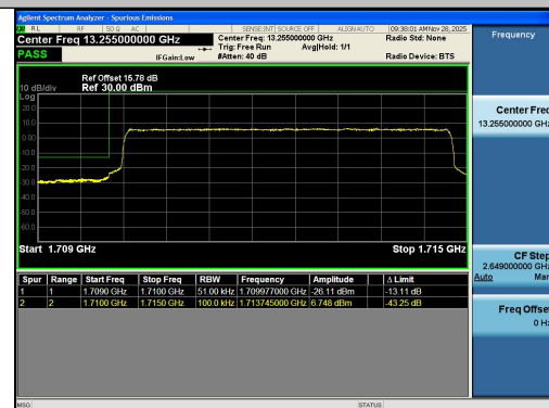
Band4-5MHz-16QAM-19975-25RB#0-PASS
