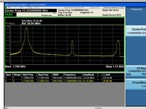
Band4-10MHz-16QAM-20000-1RB#0-PASS
