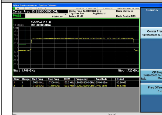
Band4-15MHz-QPSK-20025-75RB#0-PASS
