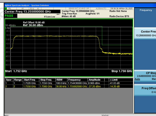
Band4-3MHz-16QAM-20385-15RB#0-PASS
