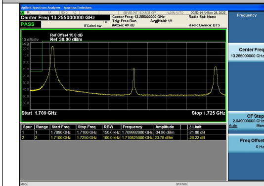
Band4-15MHz-QPSK-20025-1RB#0-PASS
