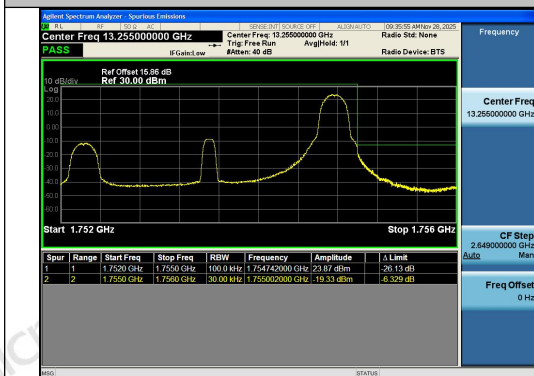
Band4-3MHz-QPSK-20385-1RB#14-PASS
