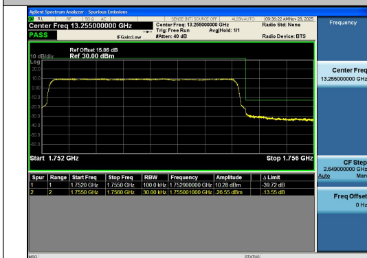
Band4-3MHz-QPSK-20385-15RB#0-PASS
