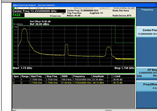
Band4-5MHz-QPSK-20375-1RB#0-PASS
