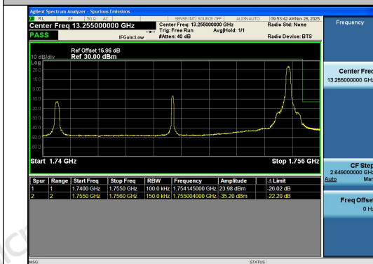
Band4-15MHz-QPSK-20325-1RB#74-PASS
