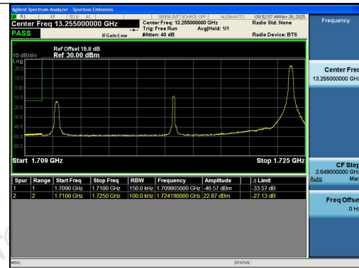
Band4-15MHz-16QAM-20025-1RB#74-PASS
