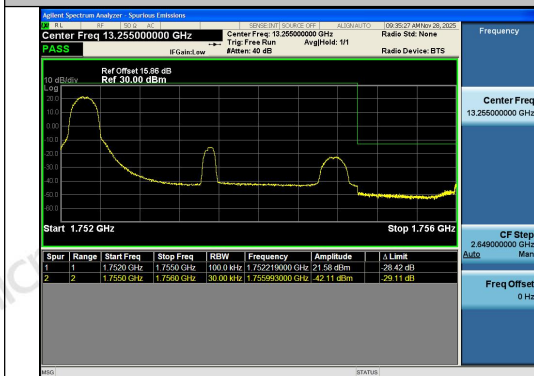
Band4-3MHz-QPSK-20385-1RB#0-PASS
