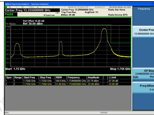
Band4-5MHz-16QAM-20375-1RB#24-PASS
