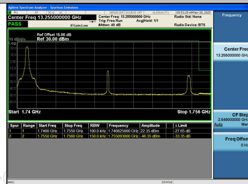
Band4-15MHz-16QAM-20325-1RB#0-PASS
