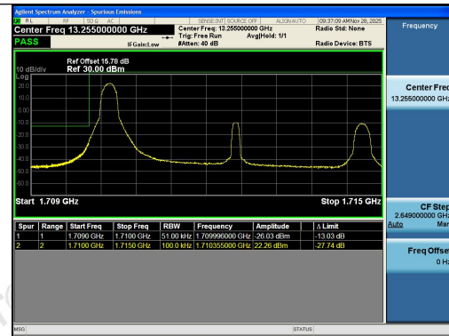
Band4-5MHz-16QAM-19975-1RB#0-PASS
