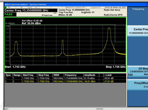
Band4-10MHz-16QAM-20350-1RB#49-PASS
