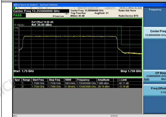
Band4-5MHz-QPSK-20375-25RB#0-PASS
