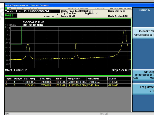
Band4-10MHz-16QAM-20000-1RB#49-PASS
