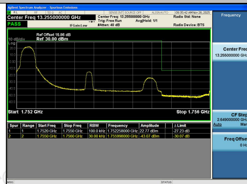
Band4-3MHz-16QAM-20385-1RB#0-PASS
