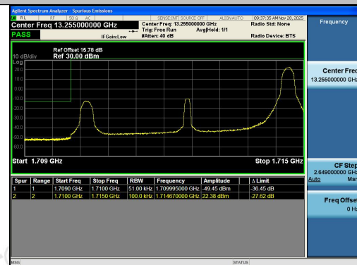
Band4-5MHz-16QAM-19975-1RB#24-PASS
