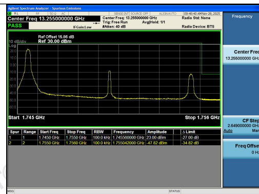
Band4-10MHz-16QAM-20350-1RB#0-PASS
