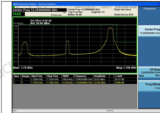
Band4-5MHz-QPSK-20375-1RB#24-PASS
