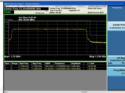
Band4-5MHz-16QAM-20375-25RB#0-PASS
