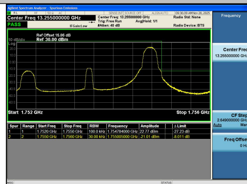
Band4-3MHz-16QAM-20385-1RB#14-PASS
