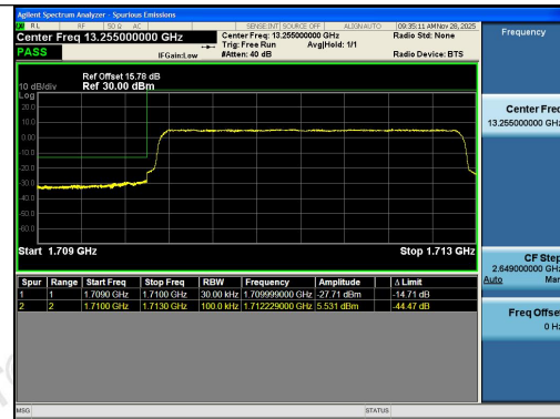
Band4-3MHz-16QAM-19965-15RB#0-PASS
