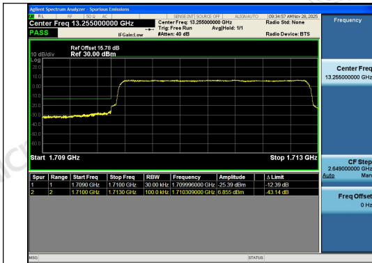
Band4-3MHz-QPSK-19965-15RB#0-PASS
