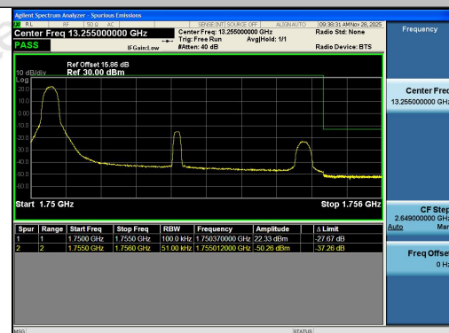
Band4-5MHz-16QAM-20375-1RB#0-PASS
