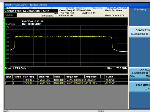
Band4-10MHz-QPSK-20350-50RB#0-PASS
