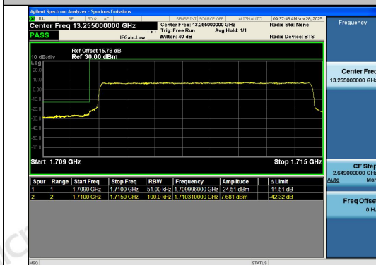
Band4-5MHz-QPSK-19975-25RB#0-PASS
