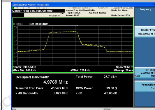
Band5-10MHz-16QAM-20525-27RB#0-PASS
