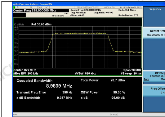
Band5-10MHz-QPSK-20450-50RB#0-PASS
