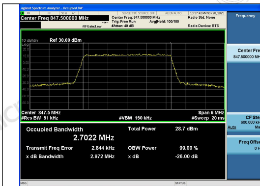
Band5-3MHz-QPSK-20635-15RB#0-PASS
