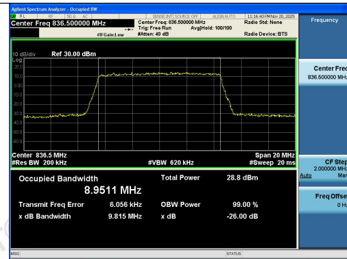
Band5-10MHz-QPSK-20525-50RB#0-PASS
