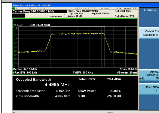
Band5-5MHz-QPSK-20625-25RB#0-PASS
