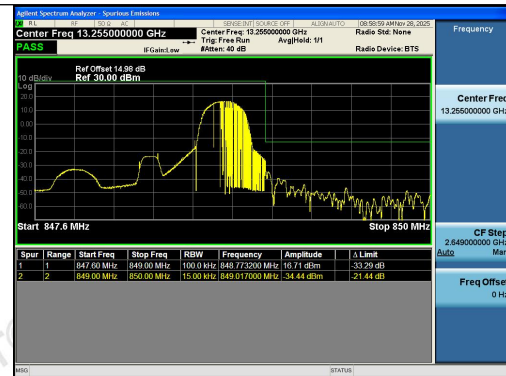
Band5-1.4MHz-16QAM-20643-1RB#5-PASS
