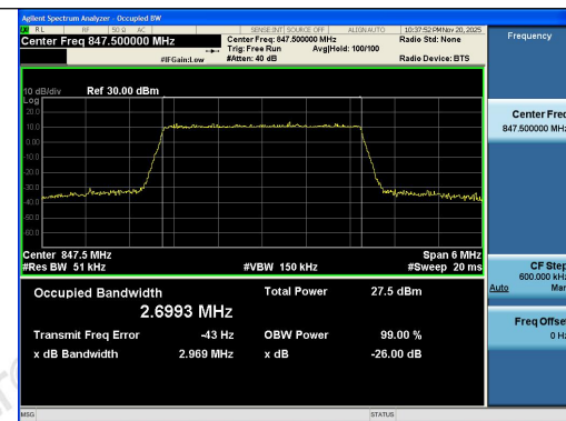
Band5-3MHz-16QAM-20635-15RB#0-PASS
