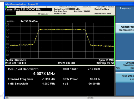
Band5-5MHz-16QAM-20425-25RB#0-PASS
