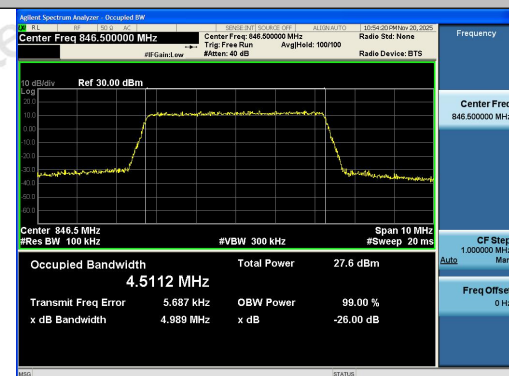
Band5-5MHz-16QAM-20625-25RB#0-PASS
