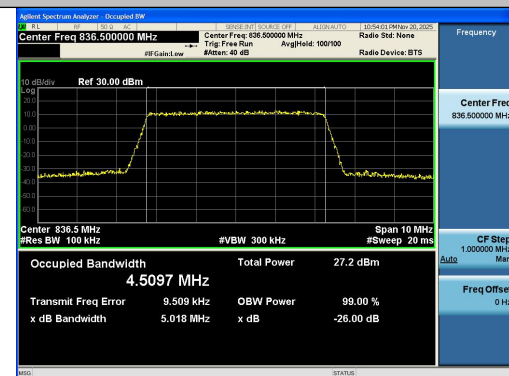
Band5-5MHz-16QAM-20525-25RB#0-PASS
