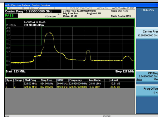
Band5-3MHz-16QAM-20415-1RB#0-PASS
