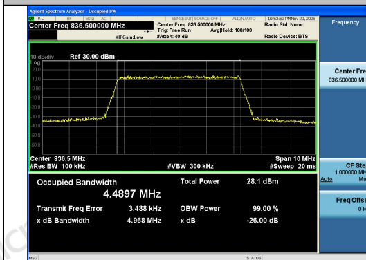
Band5-5MHz-QPSK-20525-25RB#0-PASS
