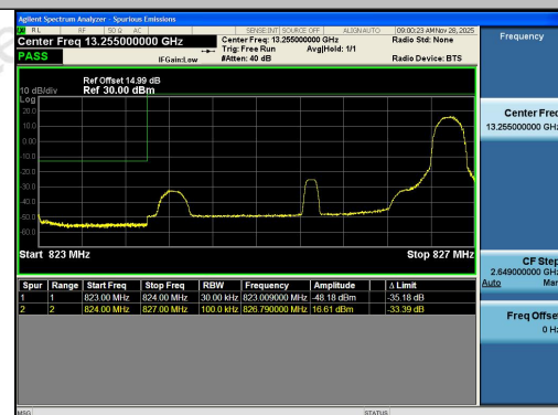
Band5-3MHz-16QAM-20415-1RB#14-PASS
