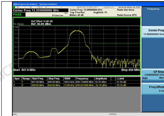
Band5-1.4MHz-QPSK-20643-1RB#5-PASS
