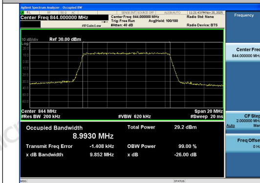
Band5-10MHz-QPSK-20600-50RB#0-PASS
