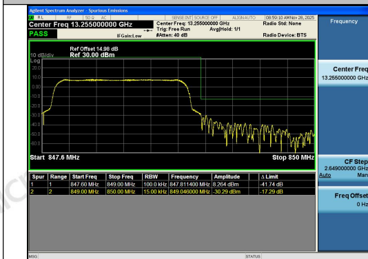
Band5-1.4MHz-QPSK-20643-6RB#0-PASS
