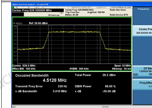
Band5-5MHz-QPSK-20425-25RB#0-PASS
