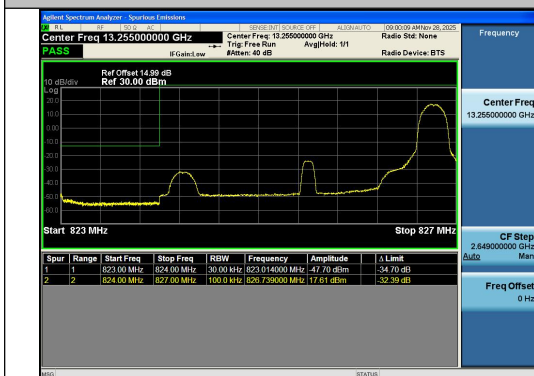
Band5-3MHz-QPSK-20415-1RB#14-PASS
