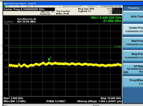
Band5-5MHz-QPSK-20425-25RB#0-3000~10000
