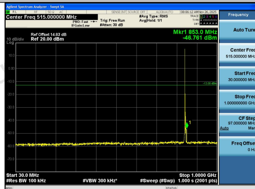
Band5-5MHz-QPSK-20625-1RB#0-30~1000-PAS
