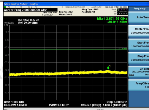
Band5-5MHz-QPSK-20625-1RB#0-1000~3000-PA
