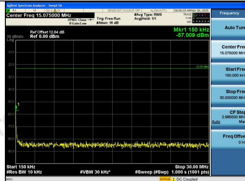
Band5-5MHz-QPSK-20625-1RB#0-0.15~30-PASS
