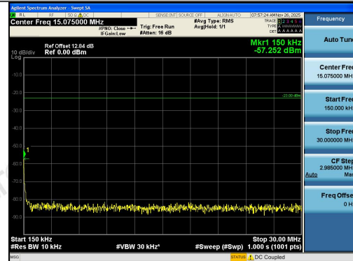
Band5-5MHz-QPSK-20425-25RB#0-0.15~30-PAS
