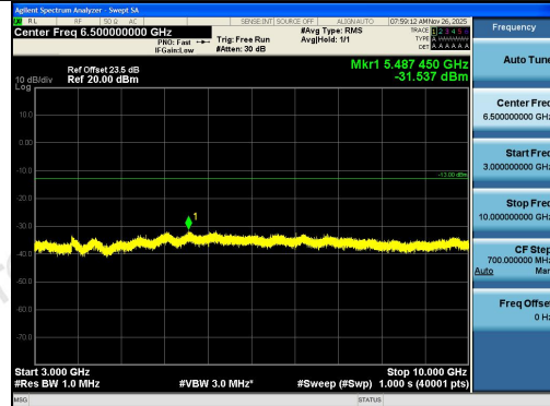
Band5-5MHz-16QAM-20425-25RB#0-3000~10000
