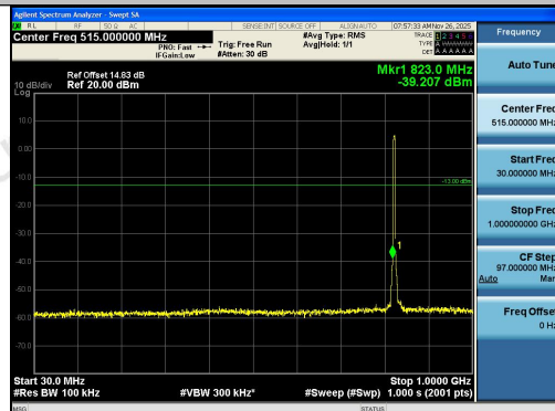
Band5-5MHz-QPSK-20425-25RB#0-30~1000-PA
