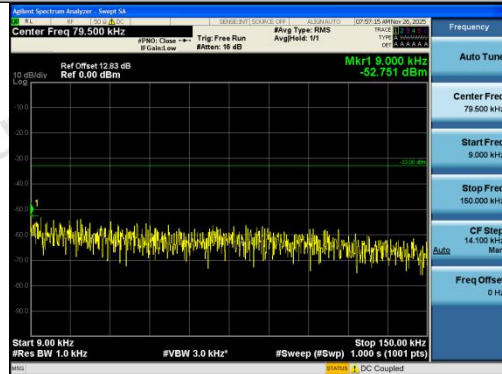
Band5-5MHz-QPSK-20425-25RB#0-0.009~0.15-
