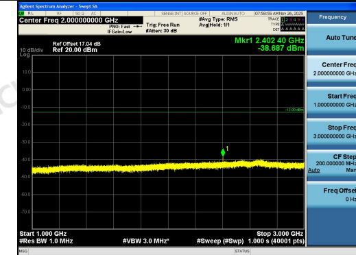
Band5-5MHz-16QAM-20425-25RB#0-1000~3000
