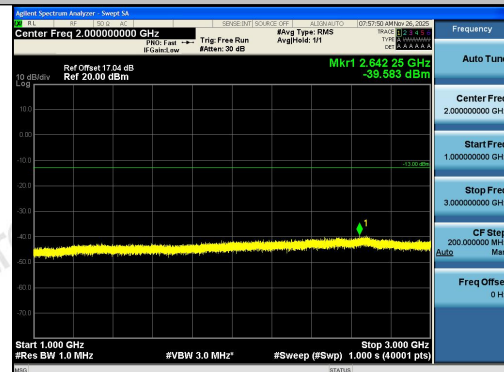
Band5-5MHz-QPSK-20425-25RB#0-1000~3000-P
