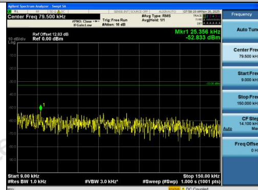
Band5-5MHz-16QAM-20425-25RB#0-0.009~0.15-
