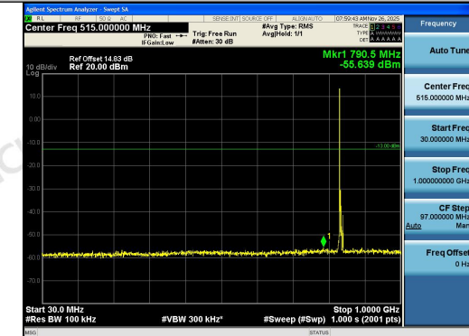
Band5-5MHz-QPSK-20525-1RB#0-30~1000-PAS
