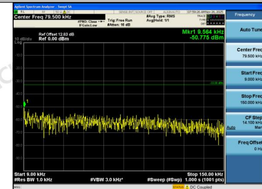
Band5-5MHz-QPSK-20525-1RB#0-0.009~0.15-P
