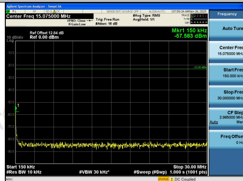
Band5-5MHz-QPSK-20525-1RB#0-0.15~30-PASS
