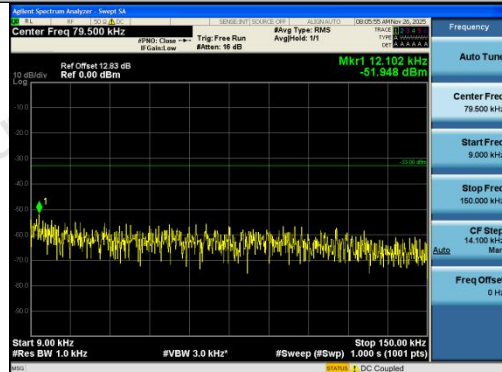
Band5-5MHz-QPSK-20625-1RB#0-0.009~0.15-P
