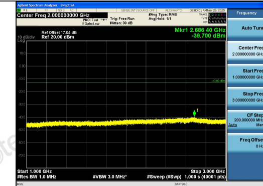
Band5-5MHz-QPSK-20525-1RB#0-1000~3000-PA
