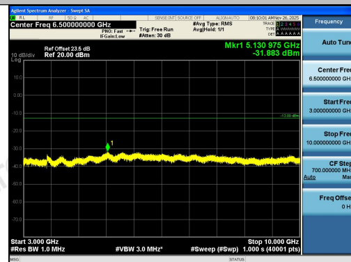
Band5-5MHz-16QAM-20625-1RB#24-3000~10000
