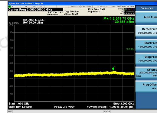
Band5-10MHz-16QAM-20450-1RB#49-1000~300
