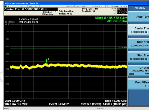
Band5-10MHz-16QAM-20450-1RB#49-3000~1000
