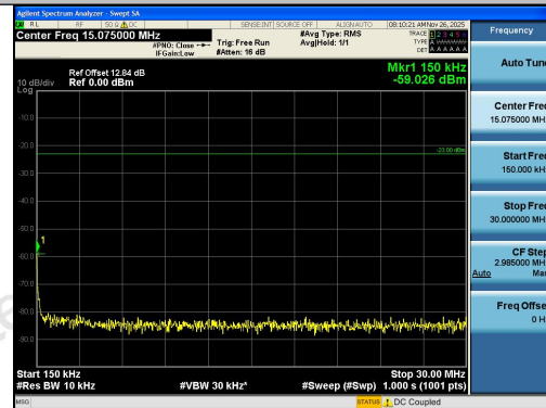
Band5-5MHz-QPSK-20625-25RB#0-0.15~30-PAS
