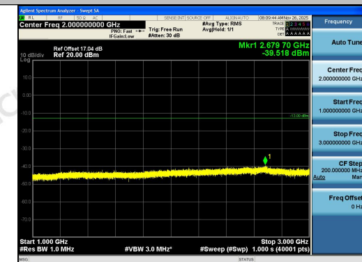
Band5-5MHz-16QAM-20625-1RB#24-1000~3000
