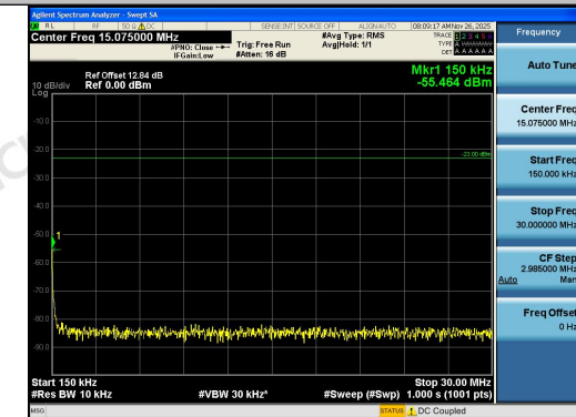
Band5-5MHz-16QAM-20625-1RB#24-0.15~30-PA
