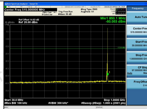
Band5-5MHz-16QAM-20625-1RB#24-30~1000-PA
