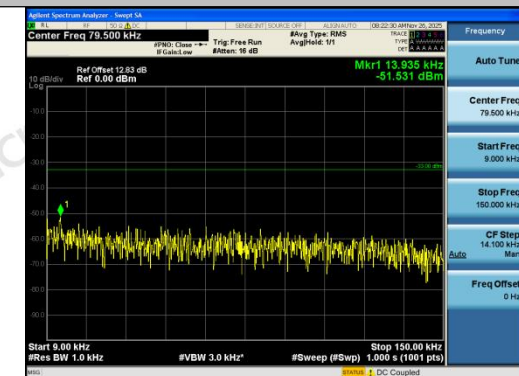
Band5-10MHz-QPSK-20525-1RB#0-0.009~0.15-
