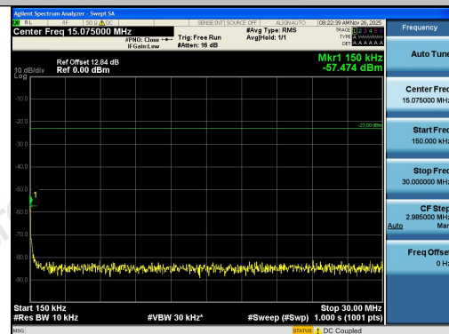
Band5-10MHz-QPSK-20525-1RB#0-0.15~30-PAS
