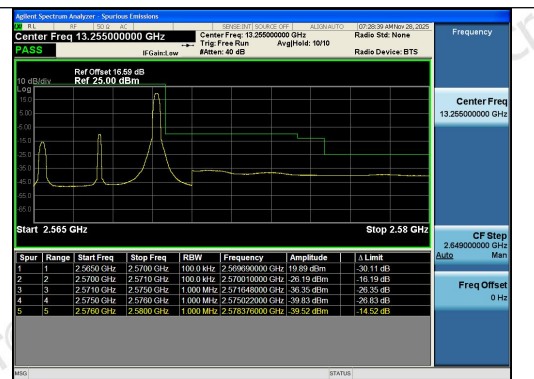
Band7-5MHz-16QAM-21425-1RB#24-PASS
