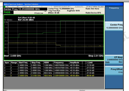
Band7-10MHz-16QAM-20800-1RB#49-PASS
