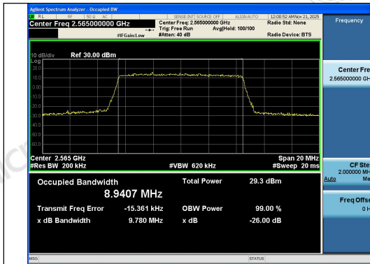
Band7-10MHz-QPSK-21400-50RB#0-PASS
