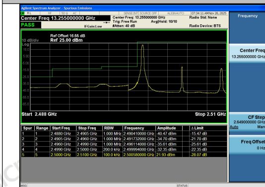
Band7-10MHz-QPSK-20800-1RB#0-PASS
