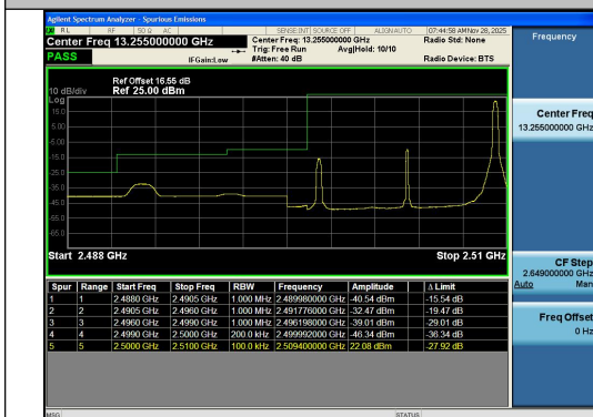
Band7-10MHz-QPSK-20800-1RB#49-PASS
