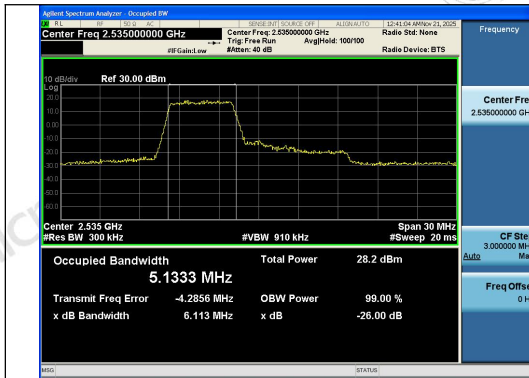
Band7-15MHz-16QAM-21100-27RB#0-PASS
