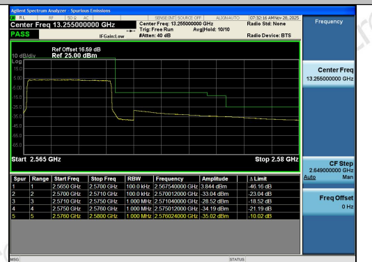
Band7-5MHz-16QAM-21425-25RB#0-PASS
