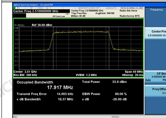
Band7-20MHz-QPSK-20850-100RB#0-PASS
