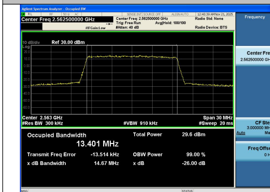
Band7-15MHz-QPSK-21375-75RB#0-PASS
