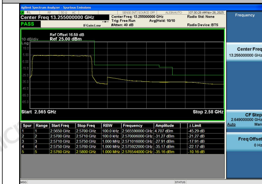
Band7-5MHz-QPSK-21425-25RB#0-PASS
