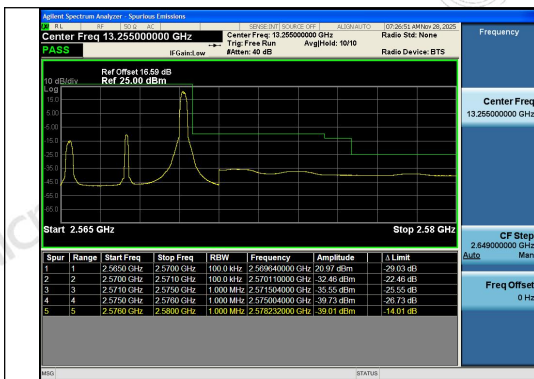
Band7-5MHz-QPSK-21425-1RB#24-PASS
