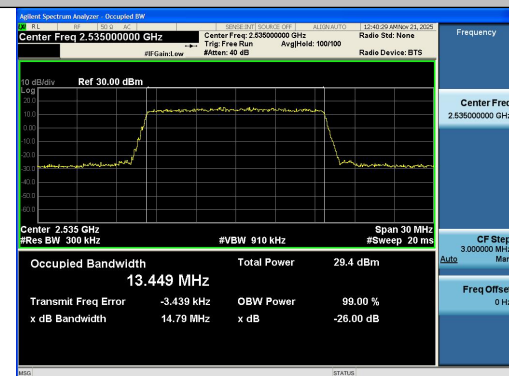
Band7-15MHz-QPSK-21100-75RB#0-PASS
