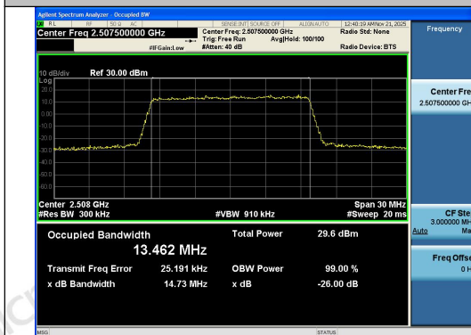
Band7-15MHz-QPSK-20825-75RB#0-PASS
