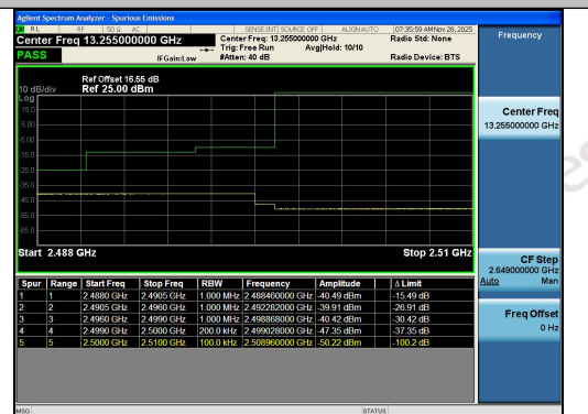
Band7-10MHz-16QAM-20800-1RB#0-PASS
