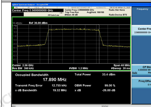
Band7-20MHz-QPSK-21350-100RB#0-PASS
