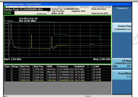
Band7-20MHz-16QAM-21350-1RB#0-PASS
