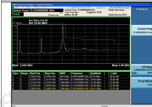
Band7-15MHz-QPSK-21375-1RB#74-PASS
