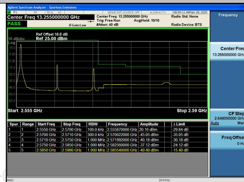
Band7-15MHz-16QAM-21375-1RB#0-PASS
