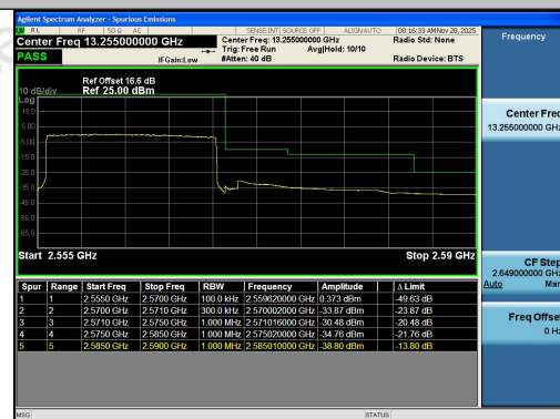
Band7-15MHz-QPSK-21375-75RB#0-PASS
