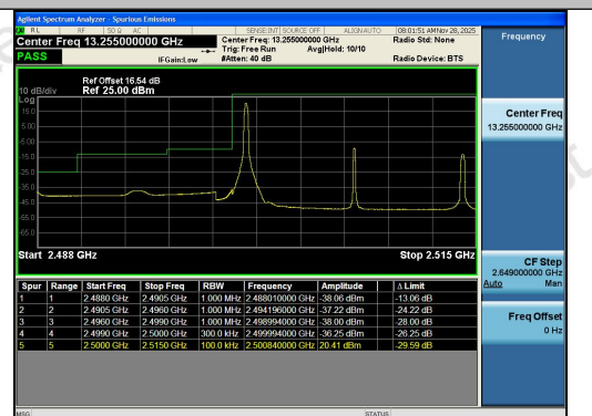
Band7-15MHz-16QAM-20825-1RB#0-PASS
