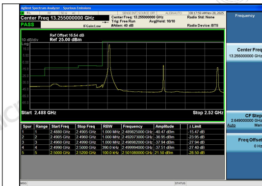
Band7-20MHz-QPSK-20850-1RB#0-PASS
