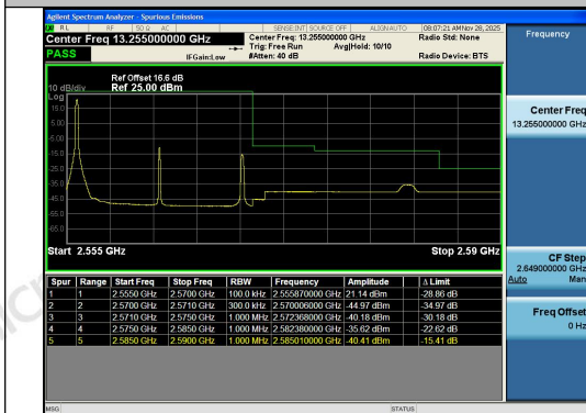
Band7-15MHz-QPSK-21375-1RB#0-PASS
