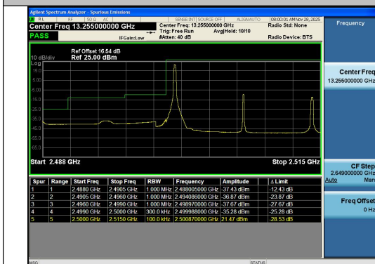
Band7-15MHz-QPSK-20825-1RB#0-PASS
