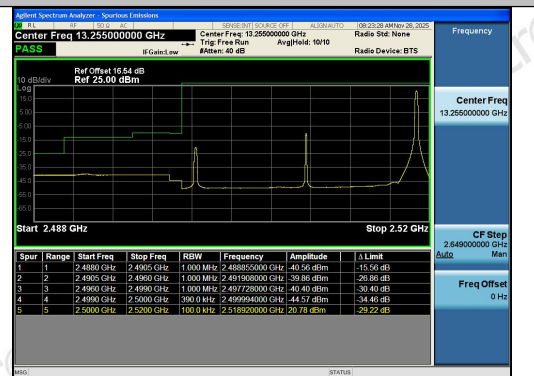
Band7-20MHz-16QAM-20850-1RB#99-PASS
