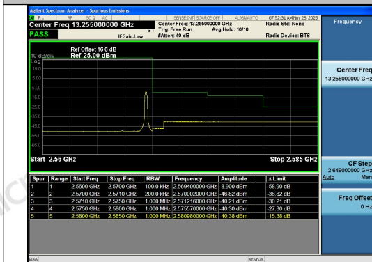
Band7-10MHz-QPSK-21400-1RB#49-PASS
