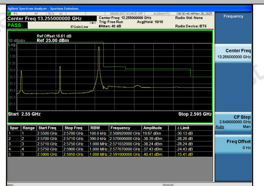
Band7-20MHz-16QAM-21350-1RB#99-PASS
