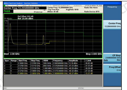
Band7-10MHz-16QAM-21400-1RB#0-PASS
