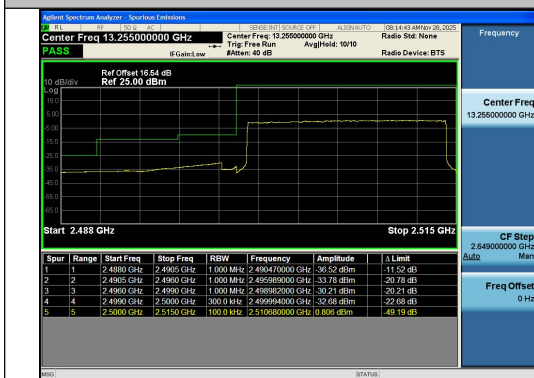
Band7-15MHz-QPSK-20825-75RB#0-PASS
