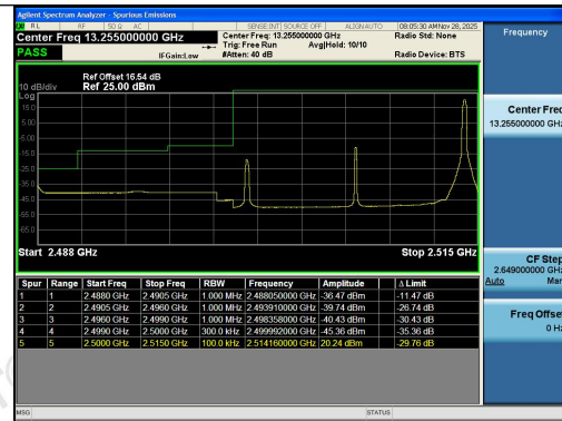
Band7-15MHz-16QAM-20825-1RB#74-PASS
