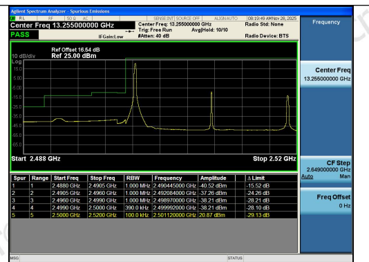
Band7-20MHz-16QAM-20850-1RB#0-PASS
