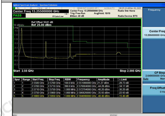
Band7-20MHz-QPSK-21350-1RB#0-PASS
