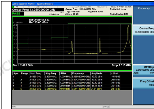
Band7-15MHz-QPSK-20825-1RB#74-PASS
