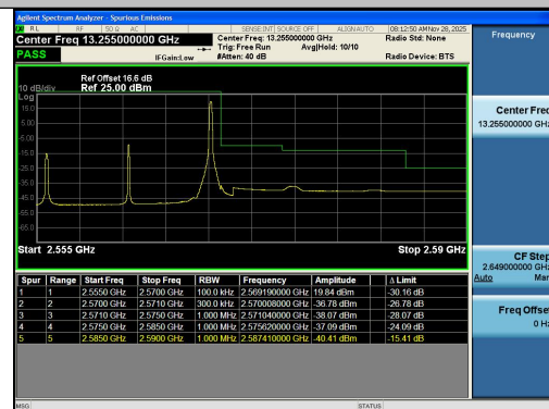
Band7-15MHz-16QAM-21375-1RB#74-PASS
