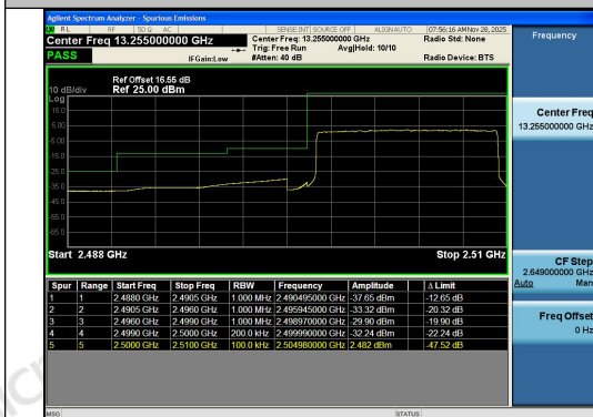
Band7-10MHz-QPSK-20800-50RB#0-PASS
