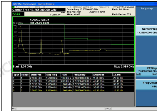
Band7-10MHz-QPSK-21400-1RB#0-PASS
