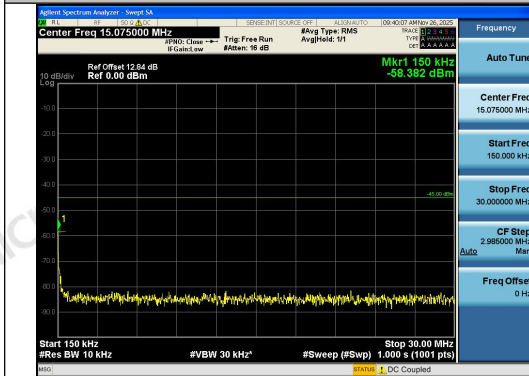
Band7-10MHz-QPSK-21100-50RB#0-0.15~30-PA SS
