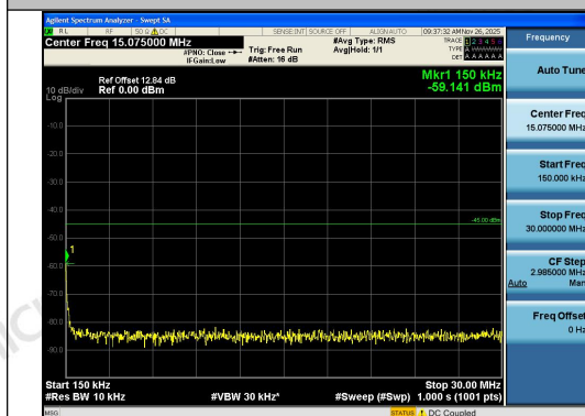
Band7-10MHz-16QAM-21400-1RB#49-0.15~30-P
