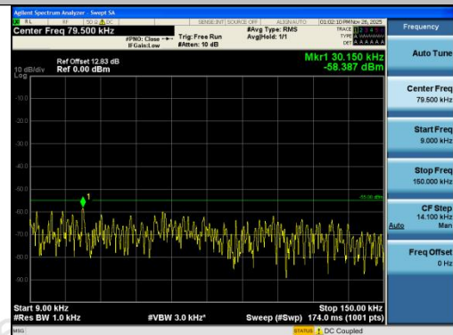
Band7-20MHz-QPSK-21350-1RB#99-0.009~0.15- PASS
