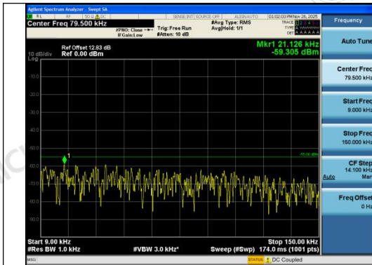
Band7-20MHz-16QAM-21350-1RB#0-0.009~0.15 -PASS
