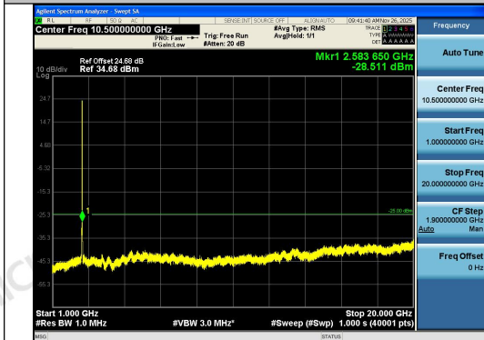
Band7-10MHz-QPSK-21400-50RB#0-1000~2000 0-PASS
