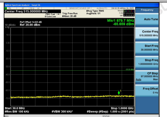
Band7-10MHz-QPSK-21400-1RB#0-30~1000-PAS S
