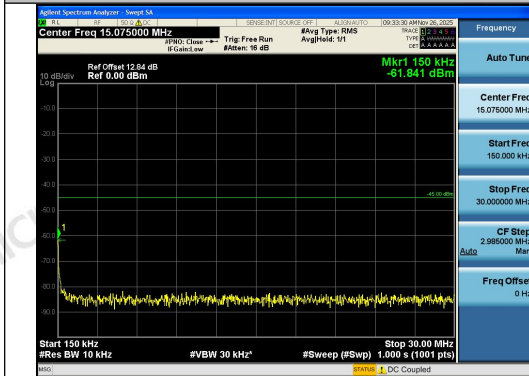
Band7-10MHz-16QAM-21400-1RB#0-0.15~30-PA SS
