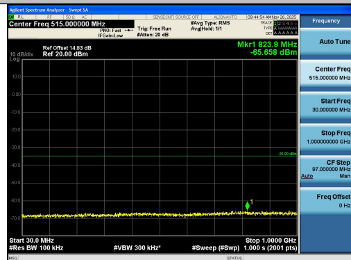
Band7-15MHz-QPSK-20825-1RB#0-30~1000-PAS S
