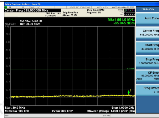
Band7-10MHz-16QAM-21400-1RB#49-30~1000-P ASS
