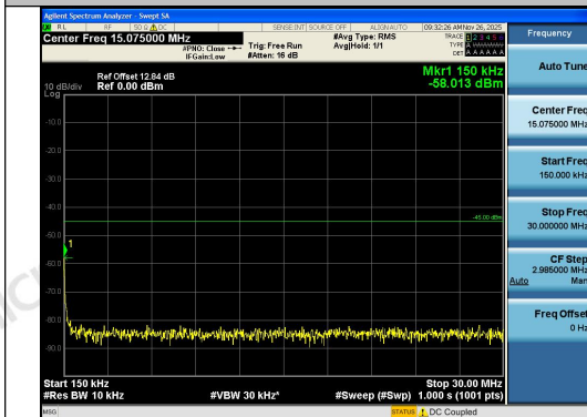
Band7-10MHz-QPSK-21400-1RB#0-0.15~30-PA SS
