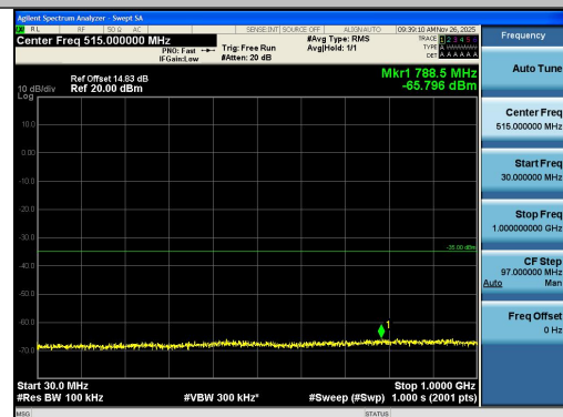
Band7-10MHz-QPSK-20800-50RB#0-30~1000-PA SS
