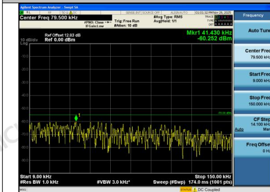
Band7-20MHz-16QAM-21100-1RB#0-0.009~0.15 -PASS
