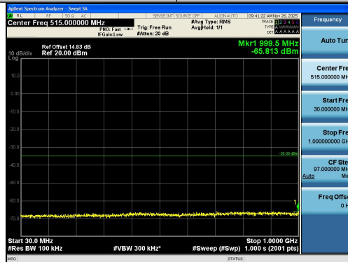
Band7-10MHz-QPSK-21400-50RB#0-30~1000-PASS
