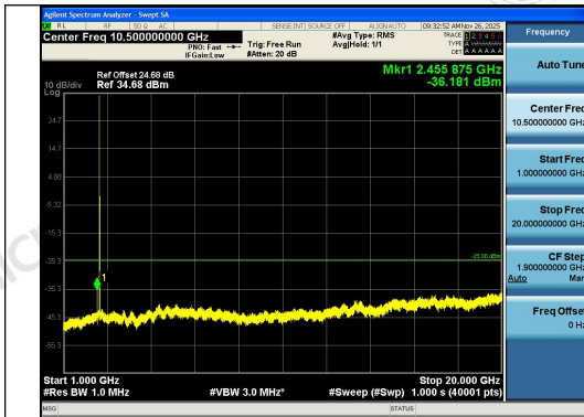
Band7-10MHz-QPSK-21400-1RB#0-1000~20000 -PASS
