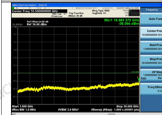
Band7-10MHz-16QAM-21400-1RB#0-1000~2000 0-PASS
