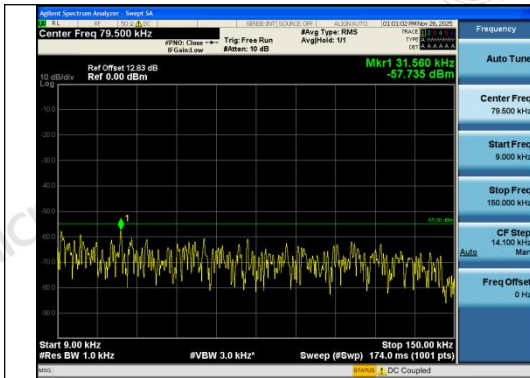
Band7-20MHz-16QAM-20850-1RB#0-0.009~0.15 -PASS
