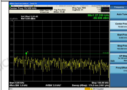
Band7-20MHz-QPSK-21100-100RB#0-0.009~0.1 5-PASS
