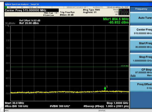
Band7-10MHz-QPSK-21100-50RB#0-30~1000-PA SS
