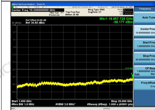
Band7-10MHz-16QAM-21400-1RB#49-1000~200 00-PASS
