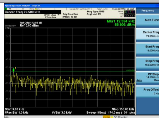
Band7-20MHz-QPSK-21350-1RB#0-0.009~0.15-P
