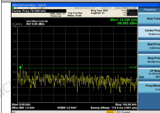
Band7-20MHz-16QAM-20850-1RB#99-0.009~0.1 5-PASS
