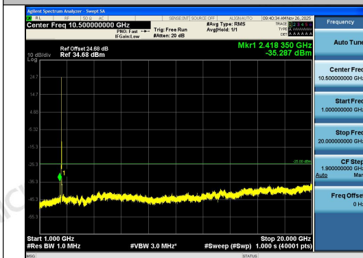
Band7-10MHz-QPSK-21100-50RB#0-1000~2000 0-PASS
