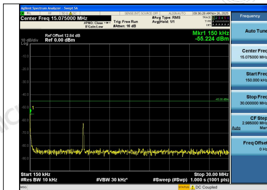
Band7-10MHz-QPSK-21400-1RB#49-0.15~30-PA
