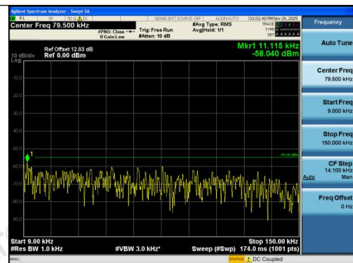
Band7-20MHz-QPSK-21100-1RB#99-0.009~0.15-
