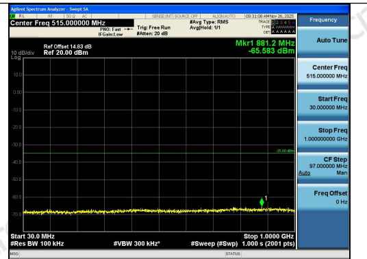
Band7-10MHz-16QAM-21100-1RB#49-30~1000-P ASS
