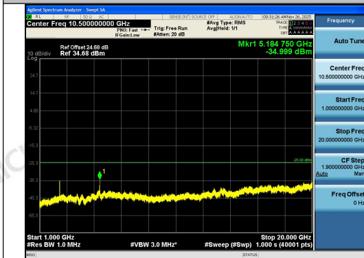
Band7-10MHz-16QAM-21100-1RB#49-1000~200 00-PASS
