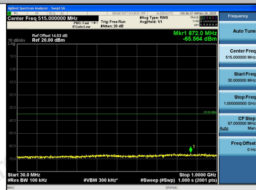
Band7-10MHz-QPSK-21400-1RB#49-30~1000-PA
