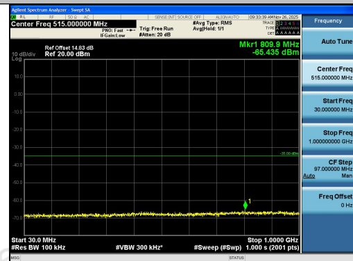
Band7-10MHz-16QAM-21400-1RB#0-30~1000-PA SS
