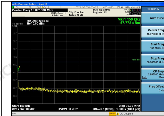
Band7-10MHz-QPSK-21400-50RB#0-0.15~30-PA SS
