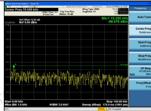
Band7-20MHz-QPSK-21100-1RB#0-0.009~0.15-P ASS
