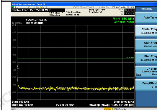
Band7-15MHz-QPSK-20825-1RB#0-0.15~30-PA SS
