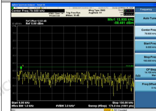
Band7-20MHz-16QAM-21350-1RB#99-0.009~0.1 5-PASS
