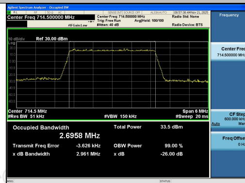
Band12-3MHz-16QAM-23165-15RB#0-PASS
