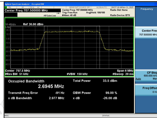
Band12-3MHz-16QAM-23095-15RB#0-PASS
