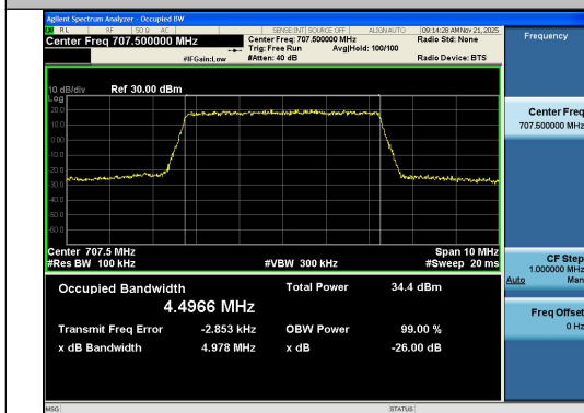
Band12-5MHz-QPSK-23095-25RB#0-PASS
