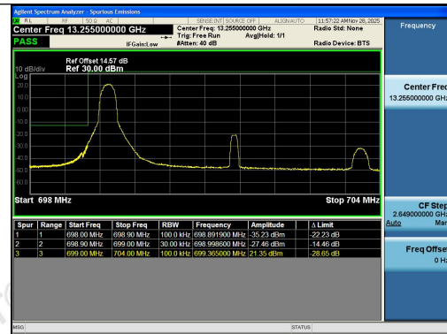
Band12-5MHz-16QAM-23035-1RB#0-PASS
