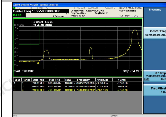
Band12-5MHz-QPSK-23035-1RB#24-PASS
