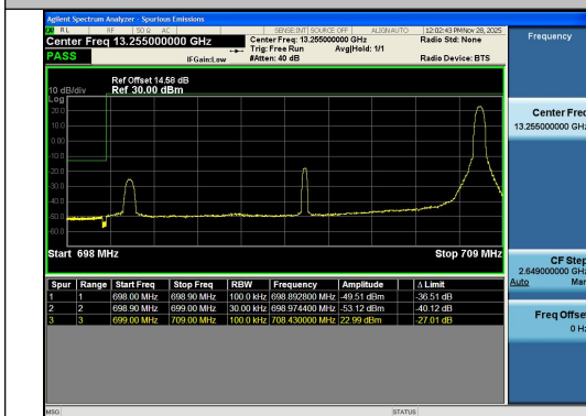
Band12-10MHz-QPSK-23060-1RB#49-PASS
