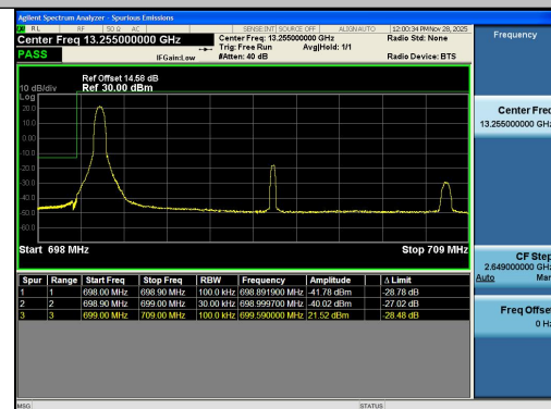
Band12-10MHz-16QAM-23060-1RB#0-PASS
