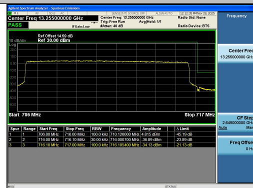
Band12-10MHz-QPSK-23130-50RB#0-PASS
