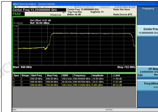
Band12-3MHz-QPSK-23025-15RB#0-PASS
