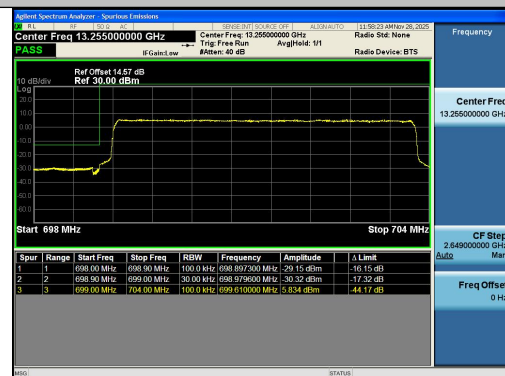
Band12-5MHz-16QAM-23035-25RB#0-PASS
