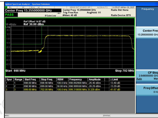
Band12-3MHz-16QAM-23025-15RB#0-PASS
