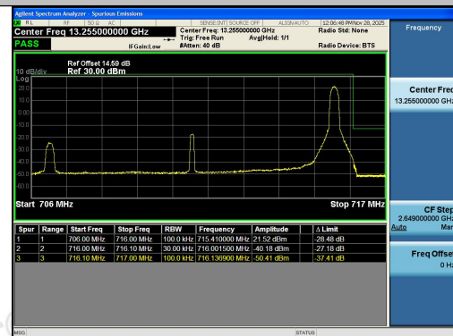
Band12-10MHz-16QAM-23130-1RB#49-PASS
