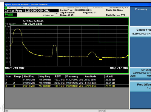
Band12-3MHz-16QAM-23165-1RB#0-PASS
