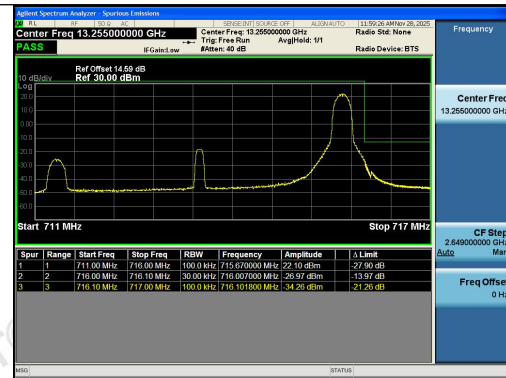
Band12-5MHz-16QAM-23155-1RB#24-PASS
