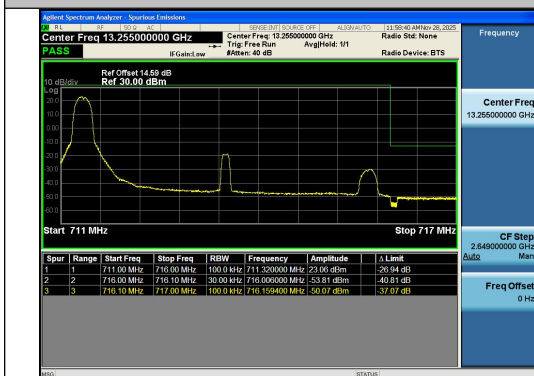
Band12-5MHz-QPSK-23155-1RB#0-PASS
