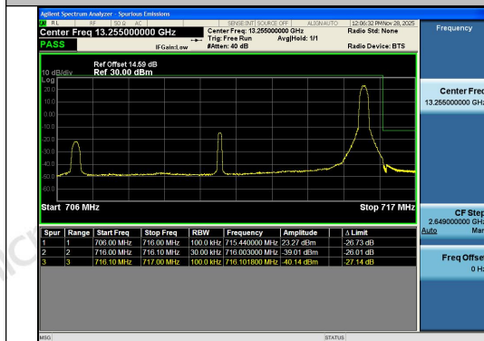
Band12-10MHz-QPSK-23130-1RB#49-PASS
