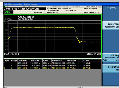
Band12-3MHz-16QAM-23165-15RB#0-PASS
