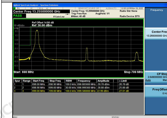
Band12-10MHz-QPSK-23060-1RB#0-PASS
