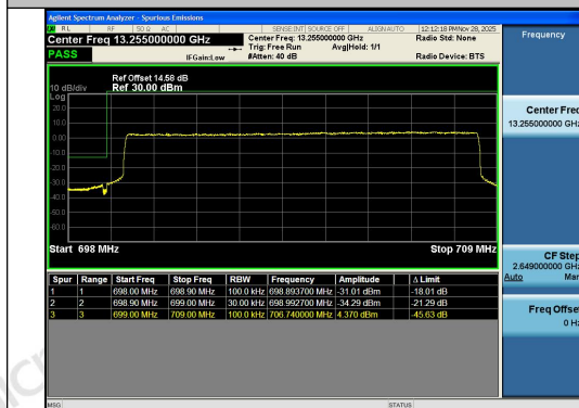
Band12-10MHz-QPSK-23060-50RB#0-PASS
