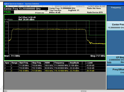
Band12-5MHz-16QAM-23155-25RB#0-PASS
