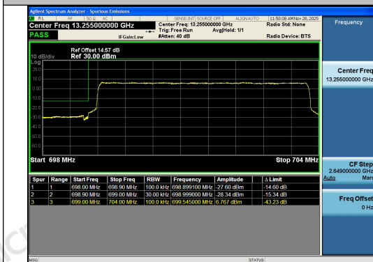
Band12-5MHz-QPSK-23035-25RB#0-PASS
