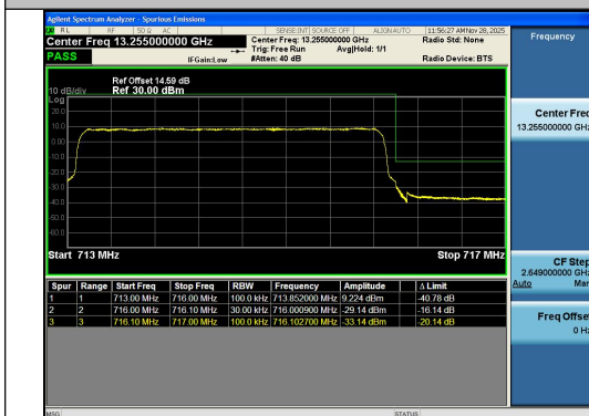
Band12-3MHz-QPSK-23165-15RB#0-PASS
