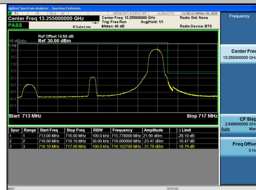
Band12-3MHz-16QAM-23165-1RB#14-PASS
