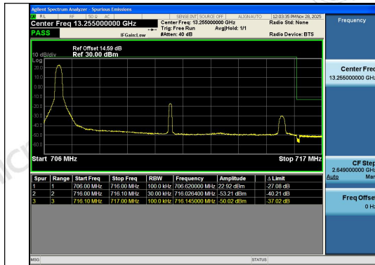
Band12-10MHz-QPSK-23130-1RB#0-PASS
