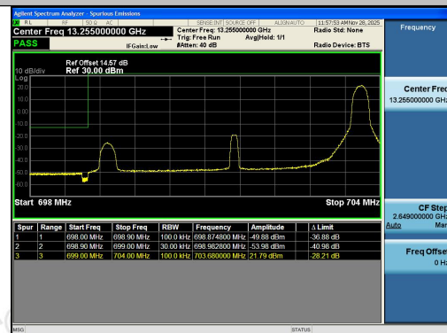
Band12-5MHz-16QAM-23035-1RB#24-PASS
