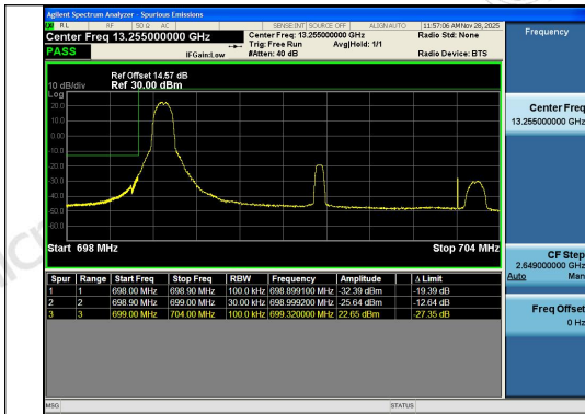
Band12-5MHz-QPSK-23035-1RB#0-PASS
