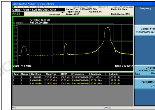
Band12-5MHz-QPSK-23155-1RB#24-PASS
