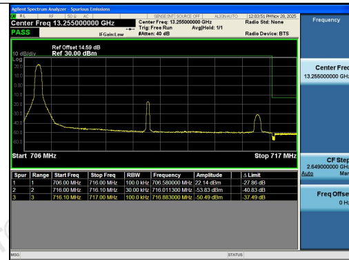
Band12-10MHz-16QAM-23130-1RB#0-PASS
