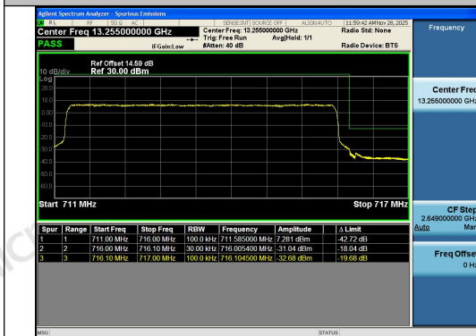
Band12-5MHz-QPSK-23155-25RB#0-PASS
