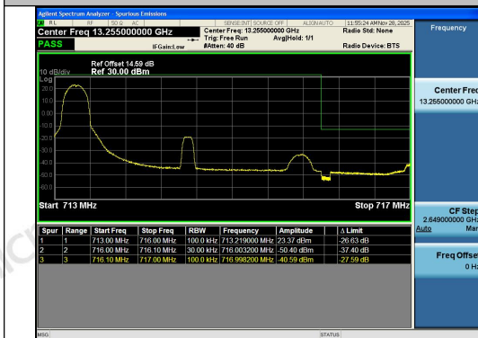
Band12-3MHz-QPSK-23165-1RB#0-PASS
