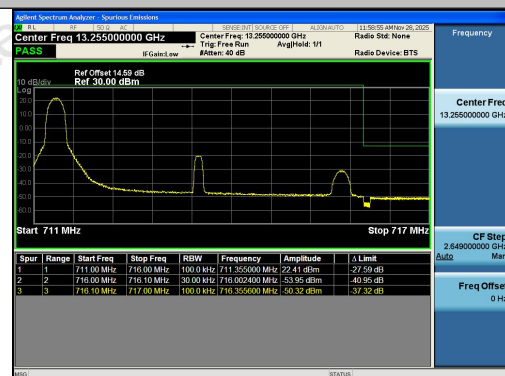
Band12-5MHz-16QAM-23155-1RB#0-PASS
