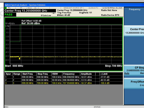
Band12-10MHz-16QAM-23060-1RB#49-PASS
