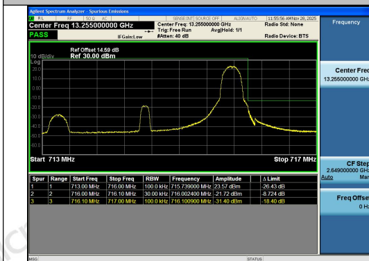
Band12-3MHz-QPSK-23165-1RB#14-PASS
