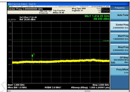
Band12-1.4MHz-QPSK-23095-1RB#0-1000~3000- PASS
