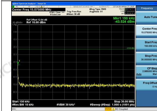
Band12-1.4MHz-QPSK-23095-1RB#5-0.15~30-P ASS
