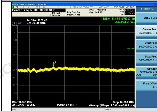
Band12-1.4MHz-QPSK-23017-1RB#5-3000~1000 0-PASS
