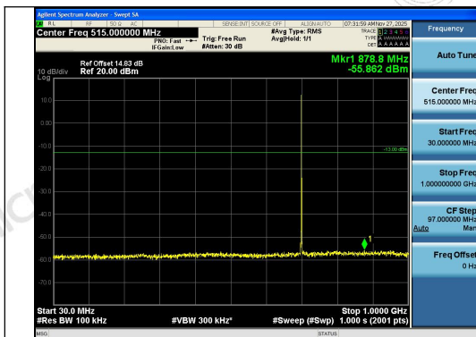
Band12-1.4MHz-QPSK-23095-1RB#0-30~1000-P ASS
