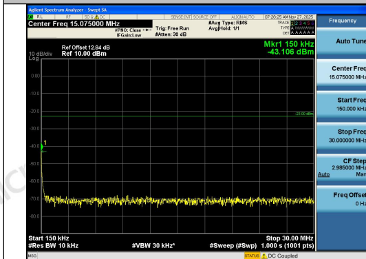
Band12-1.4MHz-16QAM-23017-1RB#5-0.15~30- PASS
