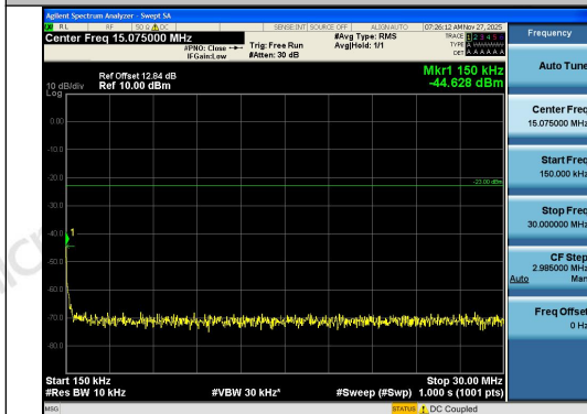
Band12-1.4MHz-16QAM-23017-1RB#0-0.15~30 PASS
