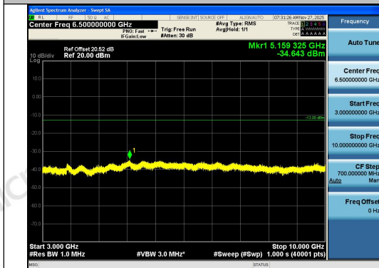
Band12-1.4MHz-16QAM-23017-6RB#0-3000~100 00-PASS
