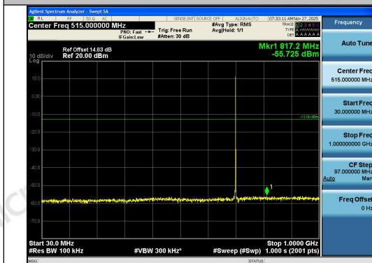
Band12-1.4MHz-16QAM-23095-1RB#0-30~1000- PASS
