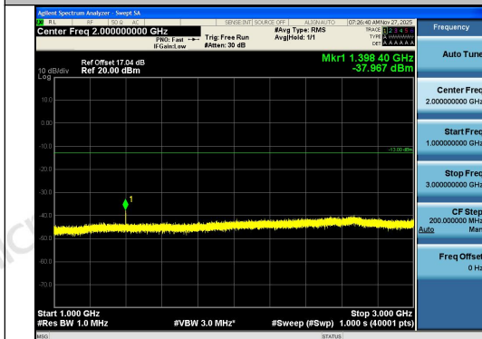
Band12-1.4MHz-16QAM-23017-1RB#0-1000~300 0-PASS
