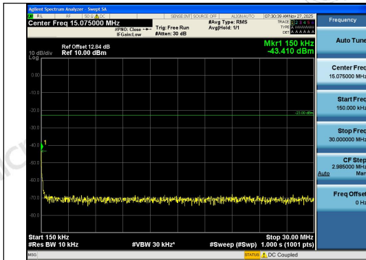
Band12-1.4MHz-16QAM-23017-6RB#0-0.15~30- PASS
