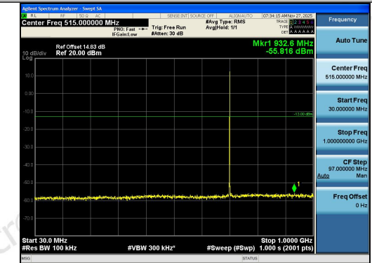
Band12-1.4MHz-QPSK-23095-1RB#5-30~1000-P ASS
