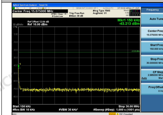
Band12-1.4MHz-16QAM-23095-1RB#0-0.15~30- PASS
