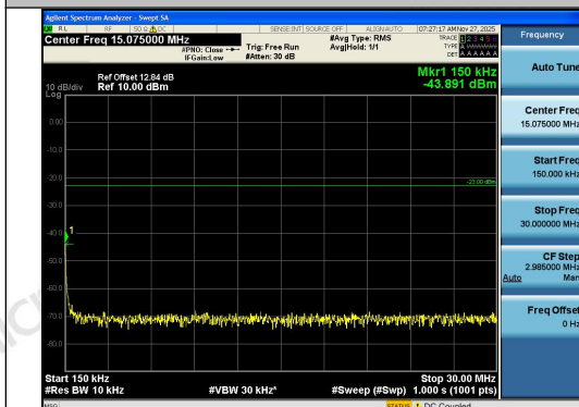
Band12-1.4MHz-QPSK-23017-1RB#5-0.15~30-P ASS
