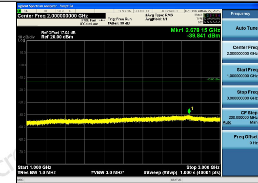
Band12-1.4MHz-16QAM-23017-6RB#0-1000~300 0-PASS
