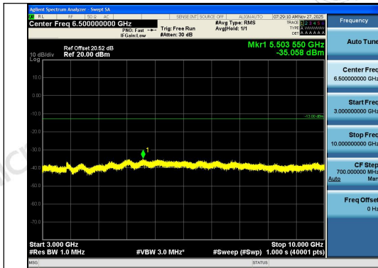
Band12-1.4MHz-16QAM-23017-1RB#5-3000~100 00-PASS
