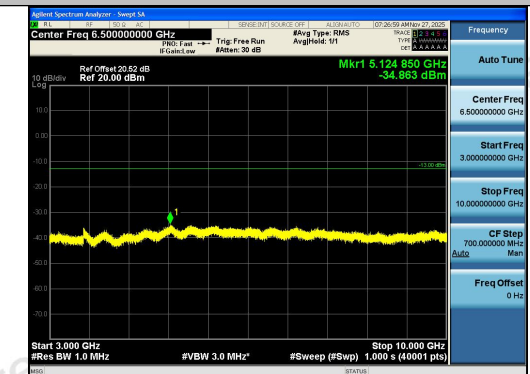
Band12-1.4MHz-16QAM-23017-1RB#0-3000~100 00-PASS
