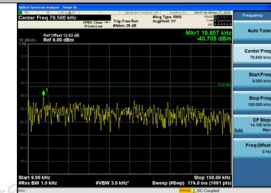
Band12-1.4MHz-16QAM-23095-6RB#0-0.009~0.1 5-PASS
