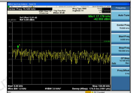
Band12-1.4MHz-16QAM-23173-1RB#0-0.009~0.1 5-PASS
