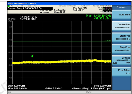
Band12-1.4MHz-QPSK-23017-1RB#5-1000~3000- PASS
