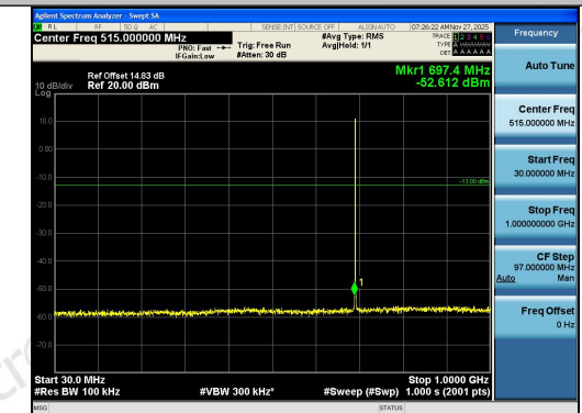
Band12-1.4MHz-16QAM-23017-1RB#0-30~1000 PASS
