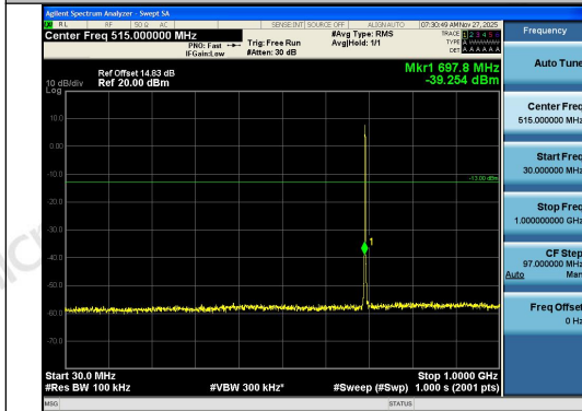
Band12-1.4MHz-16QAM-23017-6RB#0-30~1000- PASS
