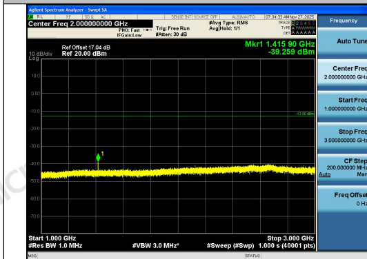
Band12-1.4MHz-QPSK-23095-1RB#5-1000~3000 -PASS
