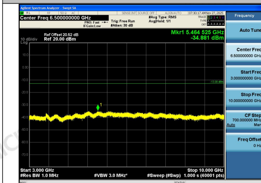
Band12-1.4MHz-QPSK-23017-6RB#0-3000~1000 0-PASS
