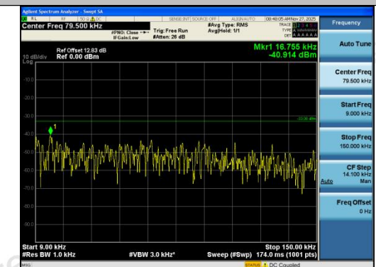
Band12-1.4MHz-QPSK-23173-1RB#5-0.009~0.15- PASS
