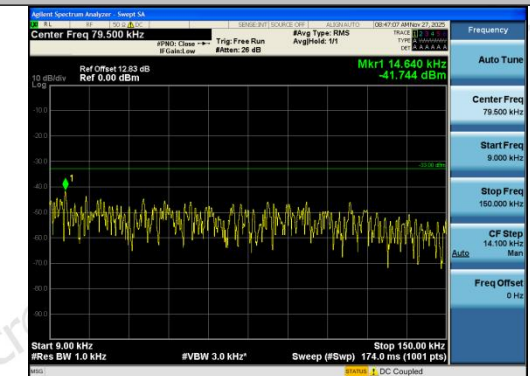
Band12-1.4MHz-16QAM-23017-6RB#0-0.009~0.1 5-PASS
