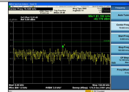
Band12-1.4MHz-QPSK-23173-1RB#0-0.009~0.15- PASS
