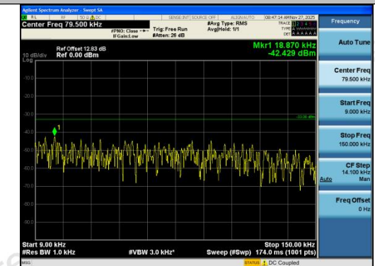
Band12-1.4MHz-QPSK-23095-1RB#0-0.009~0.15- PASS
