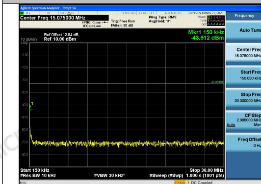
Band12-1.4MHz-16QAM-23095-1RB#5-0.15~30-PASS
