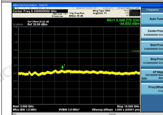
Band12-1.4MHz-QPSK-23095-1RB#0-3000~1000 0-PASS
