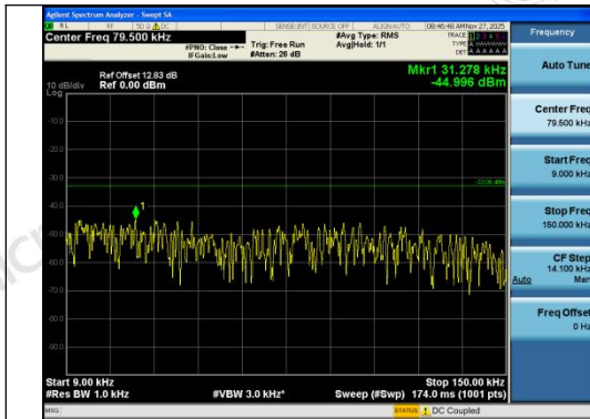
Band12-1.4MHz-QPSK-23017-1RB#5-0.009~0.15 -PASS
