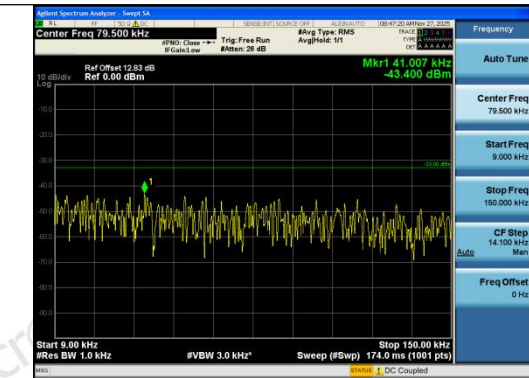
Band12-1.4MHz-16QAM-23095-1RB#0-0.009~0.1 5-PASS
