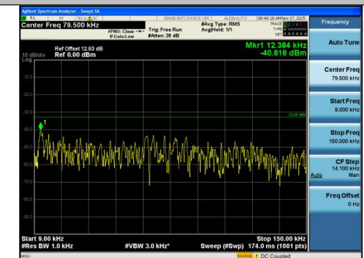
Band12-1.4MHz-QPSK-23173-6RB#0-0.009~0.15-PASS
