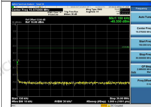
Band12-1.4MHz-QPSK-23017-6RB#0-0.15~30-P ASS
