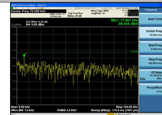
Band12-1.4MHz-16QAM-23095-1RB#5-0.009~0.1 5-PASS
