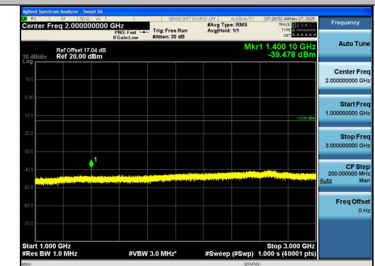
Band12-1.4MHz-16QAM-23017-1RB#5-1000~300 0-PASS
