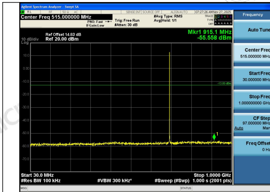
Band12-1.4MHz-QPSK-23017-1RB#5-30~1000-P ASS
