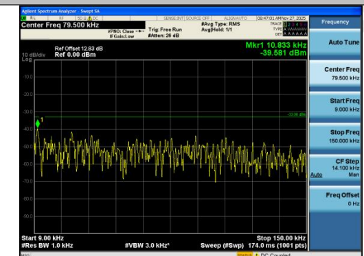
Band12-1.4MHz-QPSK-23017-6RB#0-0.009~0.15- PASS
