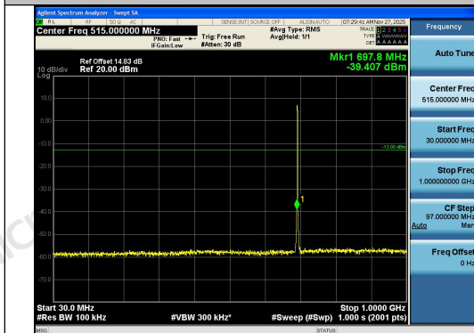
Band12-1.4MHz-QPSK-23017-6RB#0-30~1000-P ASS
