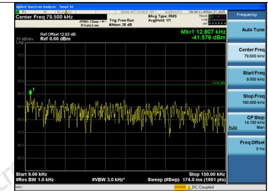
Band12-1.4MHz-16QAM-23173-1RB#5-0.009~0.1 5-PASS
