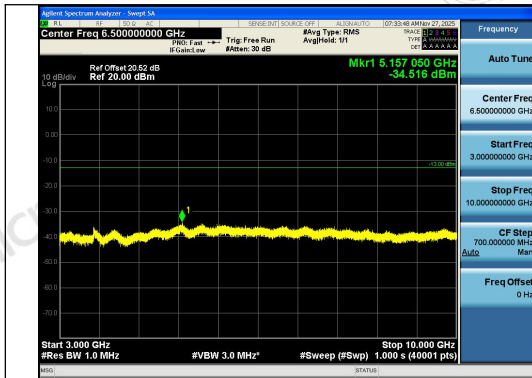
Band12-1.4MHz-16QAM-23095-1RB#0-3000~100 00-PASS
