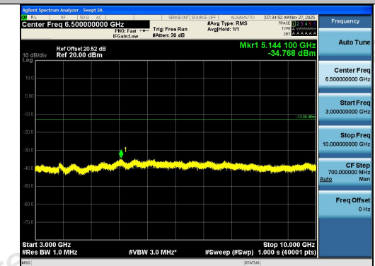
Band12-1.4MHz-QPSK-23095-1RB#5-3000~1000 0-PASS
