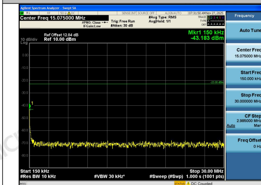
Band12-1.4MHz-QPSK-23095-1RB#0-0.15~30-P ASS
