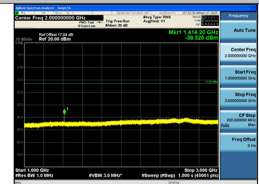
Band12-1.4MHz-16QAM-23095-1RB#0-1000~300 0-PASS
