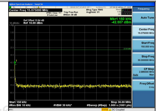
Band12-1.4MHz-16QAM-23173-1RB#0-0.15~30-P ASS
