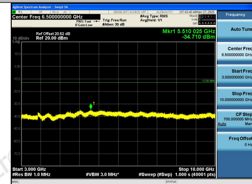
Band12-1.4MHz-QPSK-23173-6RB#0-3000~1000 0-PASS
