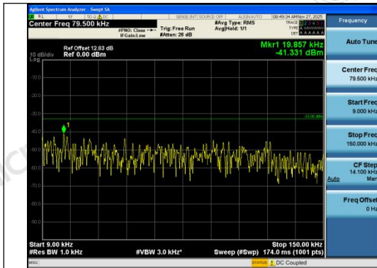
Band12-3MHz-QPSK-23095-15RB#0-0.009~0.15- PASS
