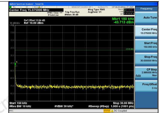
Band12-1.4MHz-QPSK-23173-1RB#0-0.15~30-PA SS
