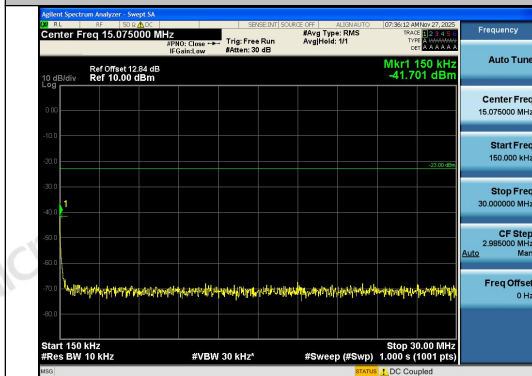
Band12-1.4MHz-QPSK-23095-6RB#0-0.15~30-P ASS
