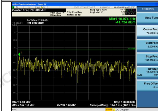
Band12-3MHz-QPSK-23095-1RB#0-0.009~0.15-P ASS
