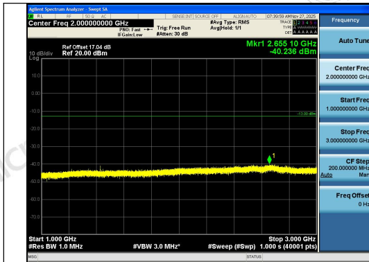
Band12-1.4MHz-16QAM-23173-1RB#0-1000~300 0-PASS
