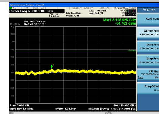
Band12-1.4MHz-QPSK-23173-1RB#5-3000~1000 0-PASS
