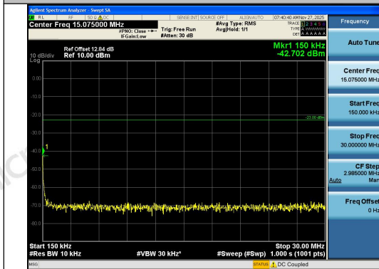
Band12-1.4MHz-QPSK-23173-1RB#5-0.15~30-P ASS
