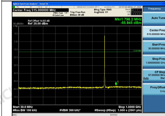
Band12-1.4MHz-16QAM-23095-6RB#0-30~1000- PASS
