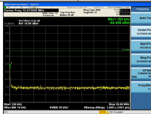
Band12-1.4MHz-16QAM-23095-6RB#0-0.15~30-PASS
