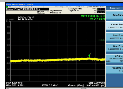
Band12-1.4MHz-16QAM-23173-6RB#0-1000~300 0-PASS
