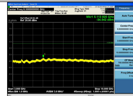
Band12-1.4MHz-QPSK-23095-6RB#0-3000~1000- 0-PASS
