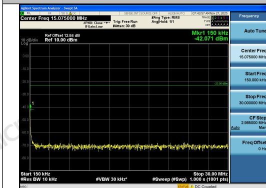
Band12-1.4MHz-16QAM-23173-6RB#0-0.15~30- PASS
