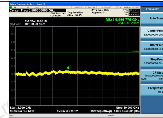
Band12-1.4MHz-16QAM-23173-1RB#0-3000~100 00-PASS
