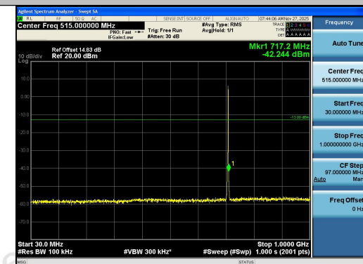
Band12-1.4MHz-16QAM-23173-6RB#0-30~1000- PASS
