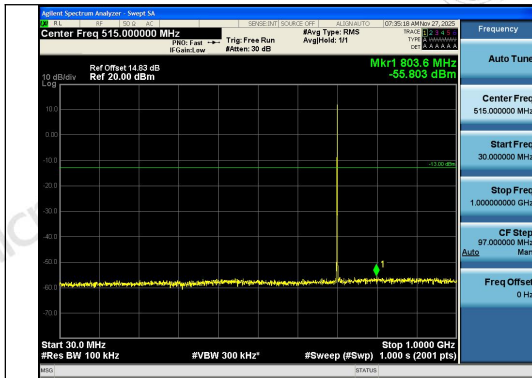
Band12-1.4MHz-16QAM-23095-1RB#5-30~1000- PASS
