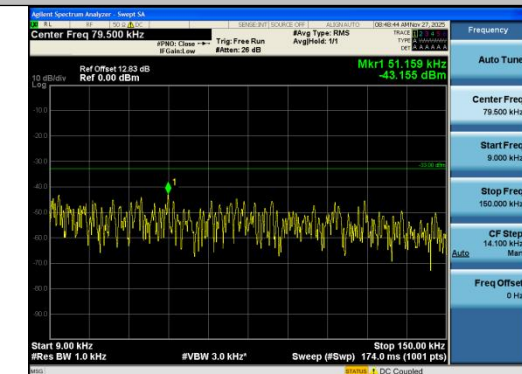
Band12-3MHz-QPSK-23025-1RB#14-0.009~0.15- PASS
