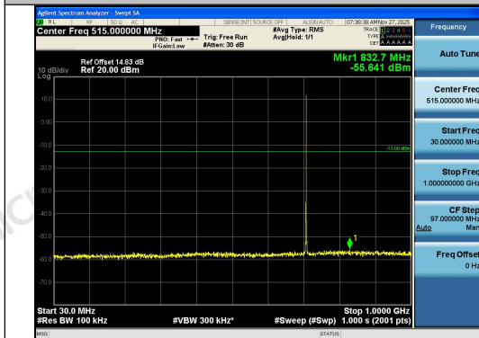
Band12-1.4MHz-QPSK-23173-1RB#0-30~1000-P ASS
