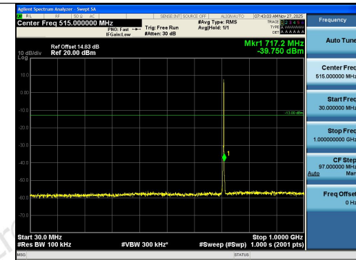
Band12-1.4MHz-QPSK-23173-6RB#0-30~1000-P ASS
