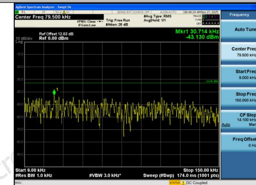
Band12-1.4MHz-16QAM-23173-6RB#0-0.009~0.1- 5-PASS
