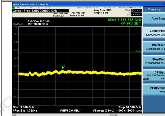
Band12-1.4MHz-16QAM-23095-6RB#0-3000~10000-PASS
