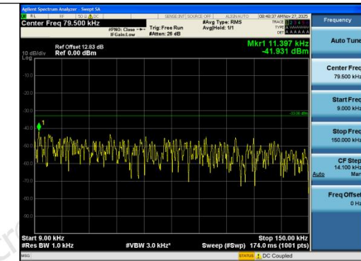
Band12-3MHz-16QAM-23025-1RB#0-0.009~0.15- PASS
