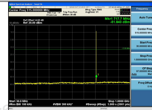
Band12-1.4MHz-QPSK-23173-1RB#5-30~1000-P ASS
