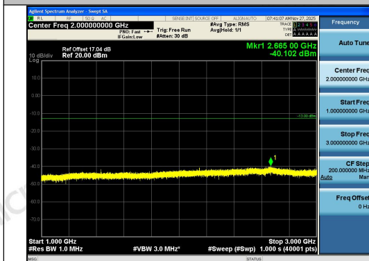
Band12-1.4MHz-QPSK-23173-1RB#5-1000~3000 -PASS
