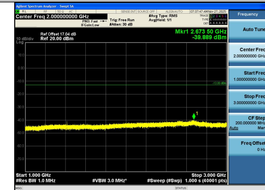
Band12-1.4MHz-16QAM-23095-6RB#0-1000~3000 0-PASS
