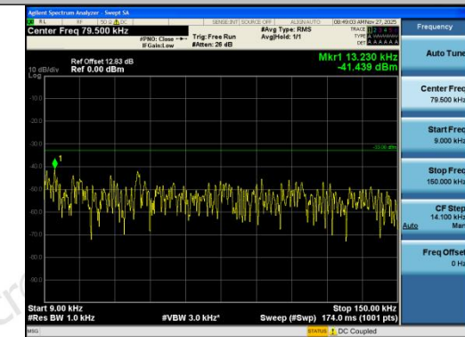
Band12-3MHz-16QAM-23025-15RB#0-0.009~0.15 -PASS
