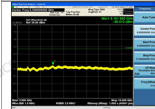
Band12-1.4MHz-16QAM-23095-1RB#5-3000~100- 00-PASS
