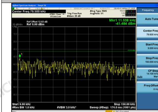
Band12-3MHz-16QAM-23095-15RB#0-0.009~0.1 5-PASS
