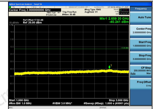
Band12-1.4MHz-QPSK-23173-1RB#0-1000~3000- PASS
