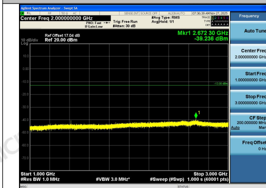
Band12-1.4MHz-QPSK-23095-6RB#0-1000~3000- -PASS
