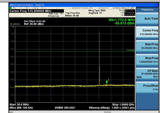
Band12-1.4MHz-16QAM-23173-1RB#0-30~1000- PASS
