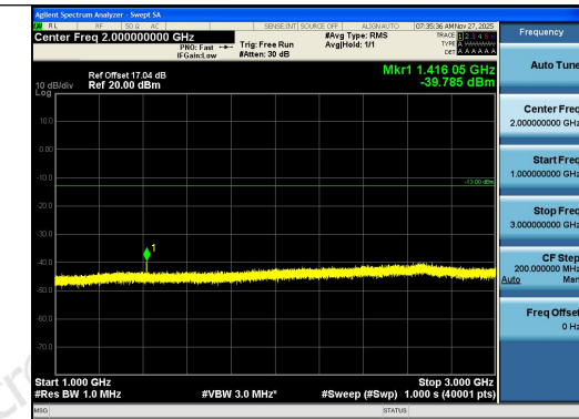
Band12-1.4MHz-16QAM-23095-1RB#5-1000~300- 0-PASS
