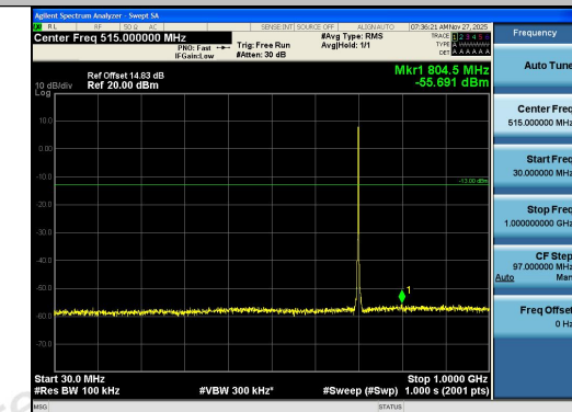
Band12-1.4MHz-QPSK-23095-6RB#0-30~1000-P ASS
