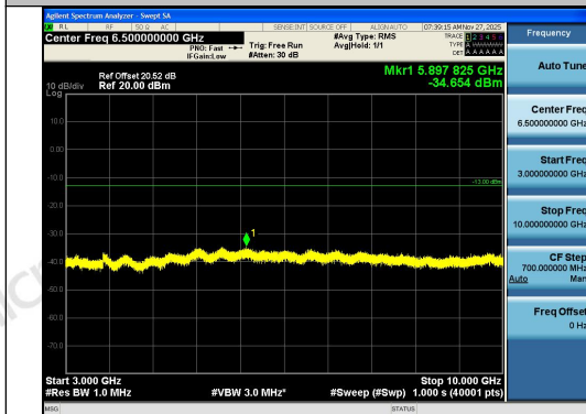
Band12-1.4MHz-QPSK-23173-1RB#0-3000~1000 0-PASS
