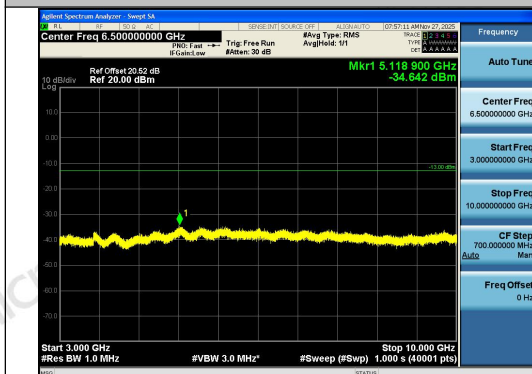
Band12-3MHz-QPSK-23095-15RB#0-3000~1000 0-PASS
