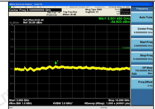
Band12-3MHz-QPSK-23095-1RB#14-3000~10000
