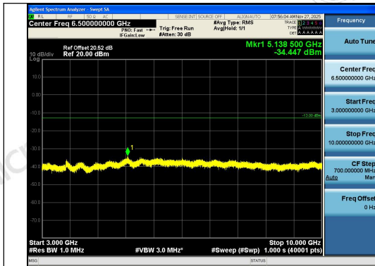
Band12-3MHz-16QAM-23095-1RB#14-3000~100 00-PASS
