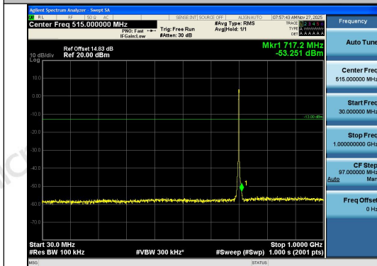
Band12-3MHz-16QAM-23095-15RB#0-30~1000- PASS
