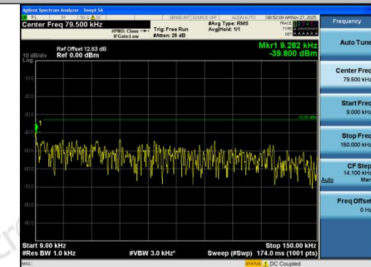
Band12-5MHz-QPSK-23155-25RB#0-0.009~0.15- PASS
