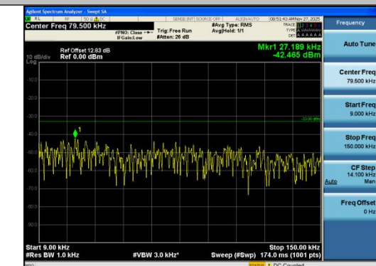
Band12-5MHz-QPSK-23155-1RB#0-0.009~0.15-P ASS
