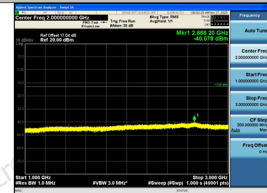
Band12-3MHz-16QAM-23165-1RB#14-1000~3000-PASS
