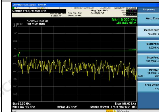
Band12-10MHz-16QAM-23095-1RB#0-0.009~0.15-5-PASS
