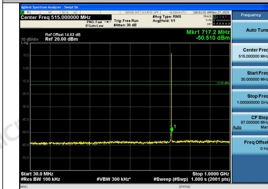
Band12-3MHz-QPSK-23165-1RB#14-30~1000-P ASS
