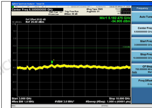
Band12-3MHz-16QAM-23165-1RB#0-3000~1000 0-PASS
