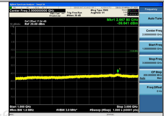
Band12-3MHz-QPSK-23165-1RB#14-1000~3000- PASS
