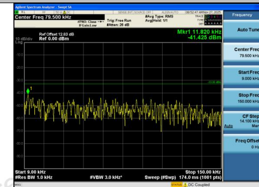
Band12-10MHz-QPSK-23095-1RB#0-0.009~0.15-PASS
