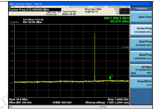
Band12-3MHz-QPSK-23095-1RB#14-30~1000-PA
