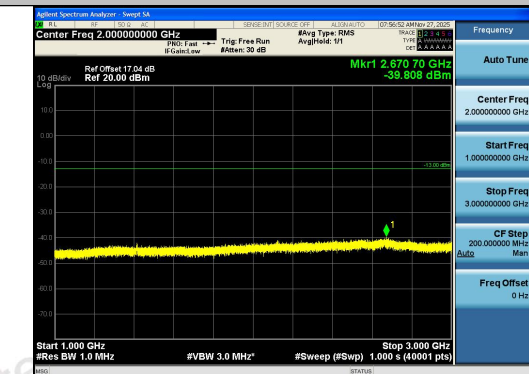
Band12-3MHz-QPSK-23095-15RB#0-1000~3000- PASS
