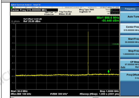
Band12-3MHz-16QAM-23095-1RB#14-30~1000-
