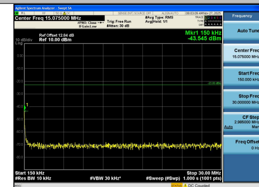
Band12-3MHz-QPSK-23165-15RB#0-0.15~30-PA SS
