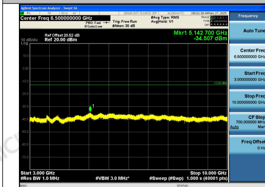
Band12-3MHz-QPSK-23165-1RB#14-3000~1000 0-PASS
