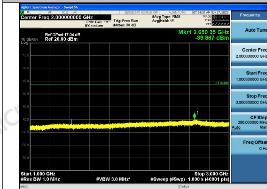
Band12-3MHz-QPSK-23095-1RB#14-1000~3000-
