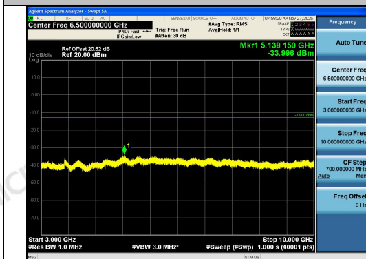
Band12-3MHz-16QAM-23095-15RB#0-3000~100 00-PASS
