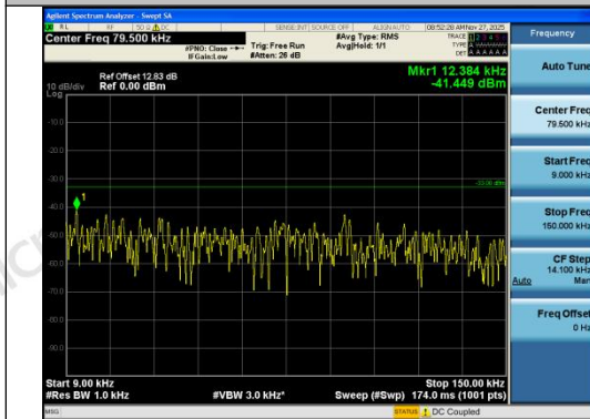
Band12-10MHz-16QAM-23060-1RB#0-0.009~0.1 5-PASS
