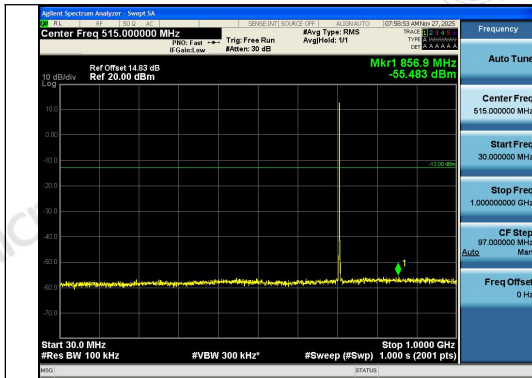
Band12-3MHz-QPSK-23165-1RB#0-30~1000-PA SS
