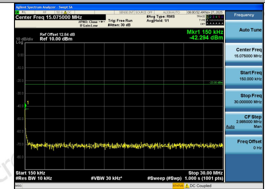
Band12-3MHz-QPSK-23165-1RB#14-0.15~30-PA SS
