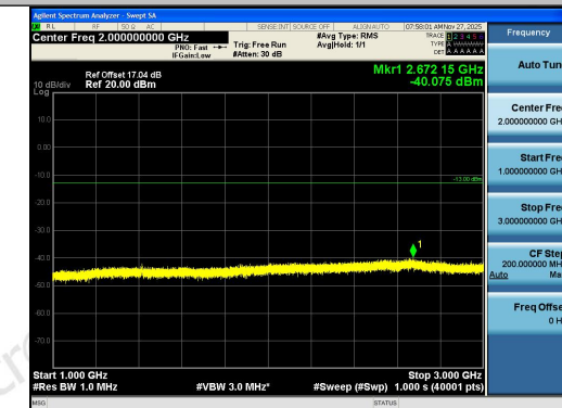
Band12-3MHz-16QAM-23095-15RB#0-1000~3000 -PASS
