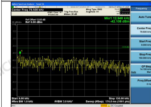
Band12-5MHz-16QAM-23095-25RB#0-0.009~0.1 5-PASS
