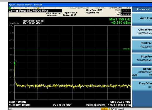
Band12-3MHz-QPSK-23165-1RB#0-0.15~30-PAS S
