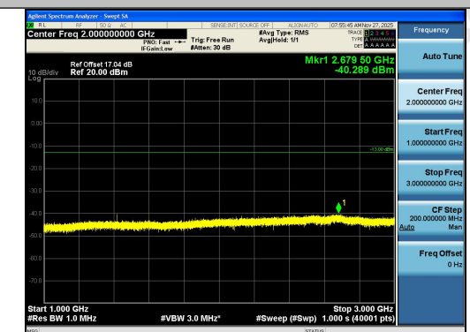
Band12-3MHz-16QAM-23095-1RB#14-1000~3000
