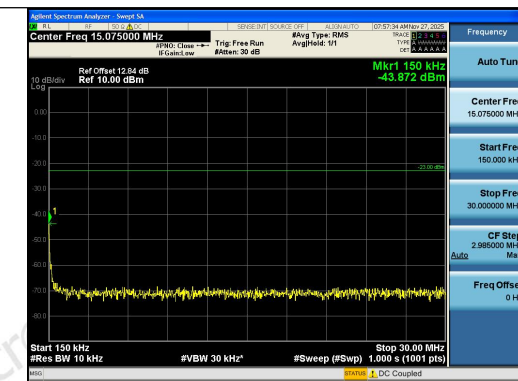
Band12-3MHz-16QAM-23095-15RB#0-0.15~30-P ASS
