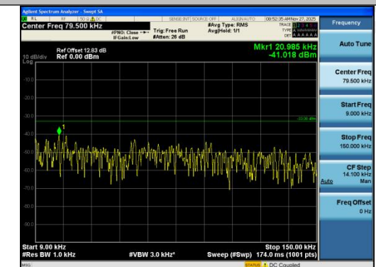
Band12-10MHz-QPSK-23060-1RB#49-0.009~0.15 -PASS
