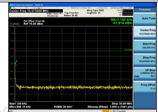
Band12-3MHz-16QAM-23095-1RB#14-0.15~30-P
