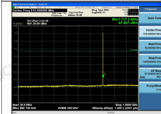
Band12-3MHz-16QAM-23165-1RB#14-30~1000-PASS
