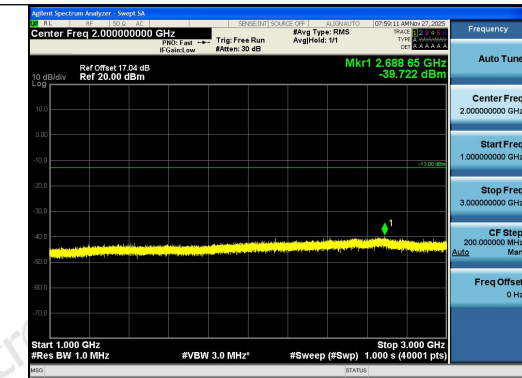
Band12-3MHz-QPSK-23165-1RB#0-1000~3000-P ASS
