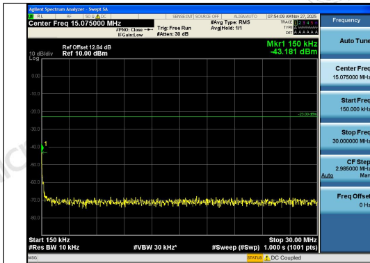
Band12-3MHz-QPSK-23095-1RB#14-0.15~30-PA
