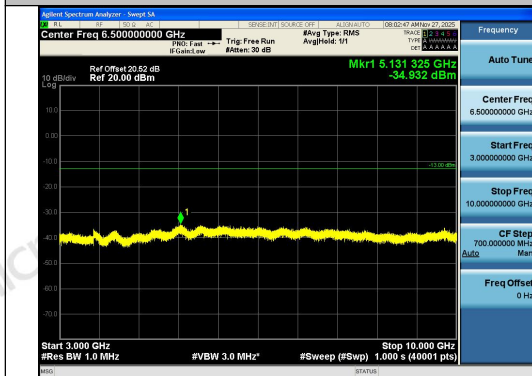
Band12-3MHz-16QAM-23165-1RB#14-3000~10000-PASS
