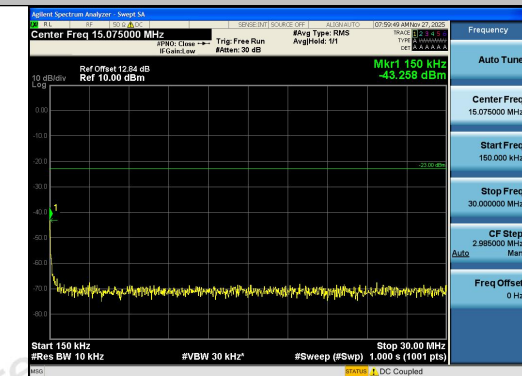
Band12-3MHz-16QAM-23165-1RB#0-0.15~30-PA SS
