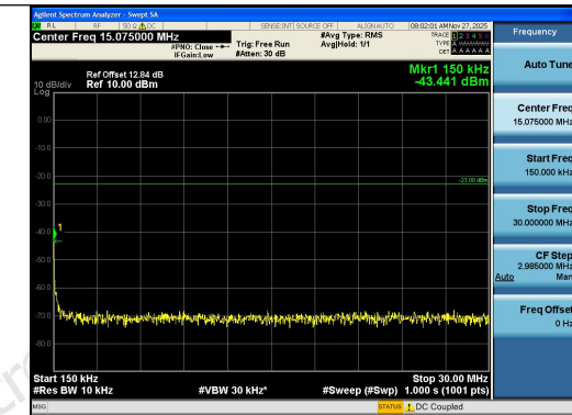
Band12-3MHz-16QAM-23165-1RB#14-0.15~30-P ASS
