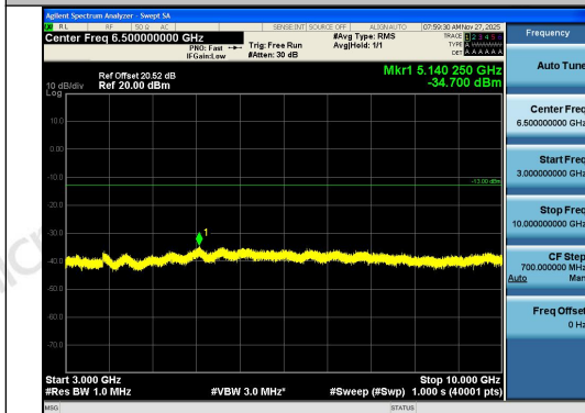
Band12-3MHz-QPSK-23165-1RB#0-3000~10000- PASS
