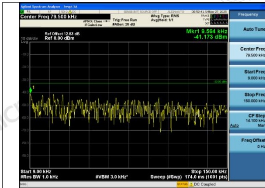
Band12-10MHz-16QAM-23060-1RB#49-0.009~0.15-PASS
