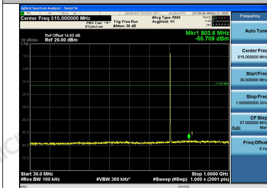
Band12-3MHz-16QAM-23165-1RB#0-30~1000-P ASS
