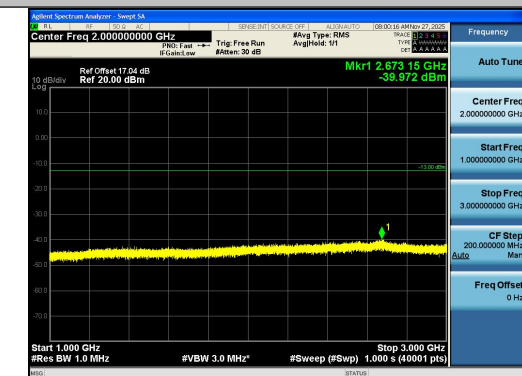
Band12-3MHz-16QAM-23165-1RB#0-1000~3000- PASS
