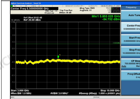
Band12-5MHz-QPSK-23035-1RB#24-3000~1000 0-PASS
