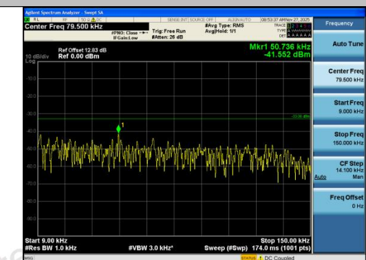
Band12-10MHz-QPSK-23060-50RB#0-0.009~0.15
