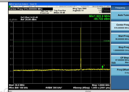
Band12-5MHz-16QAM-23095-1RB#0-30~1000-PA
