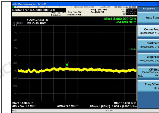
Band12-3MHz-16QAM-23165-15RB#0-3000~100 00-PASS
