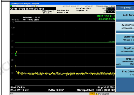
Band12-5MHz-16QAM-23035-25RB#0-0.15~30-P
