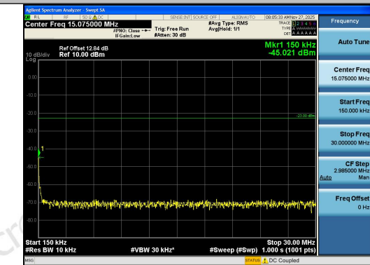
Band12-5MHz-QPSK-23035-1RB#0-0.15~30-PAS S
