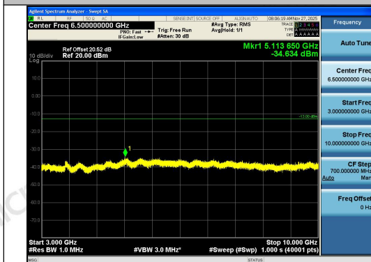
Band12-5MHz-QPSK-23035-1RB#0-3000~10000- PASS
