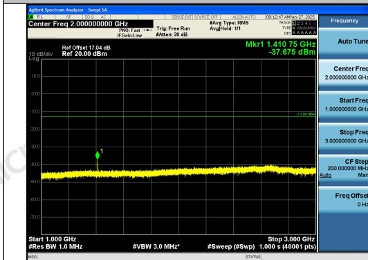
Band12-5MHz-QPSK-23095-1RB#0-1000~3000-P
