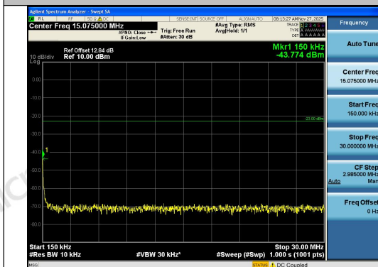
Band12-5MHz-16QAM-23095-1RB#0-0.15~30-PA
