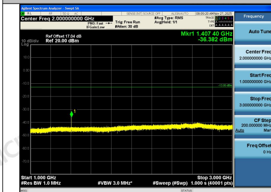
Band12-5MHz-16QAM-23035-1RB#24-1000~300 0-PASS
