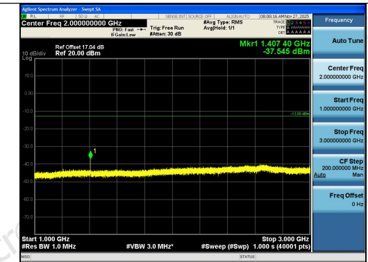
Band12-5MHz-QPSK-23035-1RB#24-1000~3000-PASS
