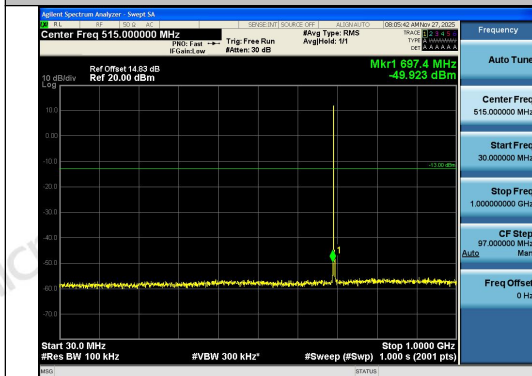
Band12-5MHz-QPSK-23035-1RB#0-30~1000-PASS
