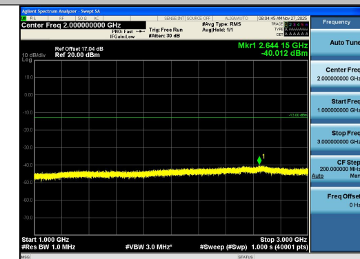
Band12-3MHz-16QAM-23165-15RB#0-1000~3000 -PASS
