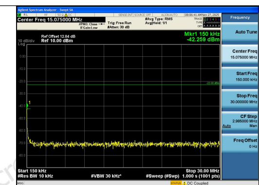
Band12-5MHz-16QAM-23035-1RB#0-0.15~30-PA
