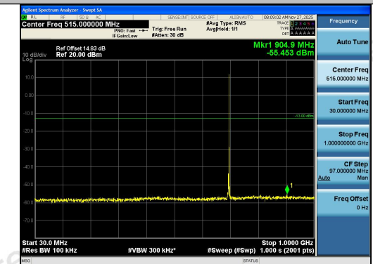
Band12-5MHz-16QAM-23035-1RB#24-30~1000-P ASS
