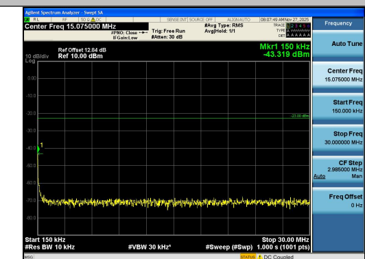
Band12-5MHz-QPSK-23035-1RB#24-0.15~30-PA
