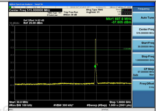
Band12-5MHz-16QAM-23035-25RB#0-30~1000-P
