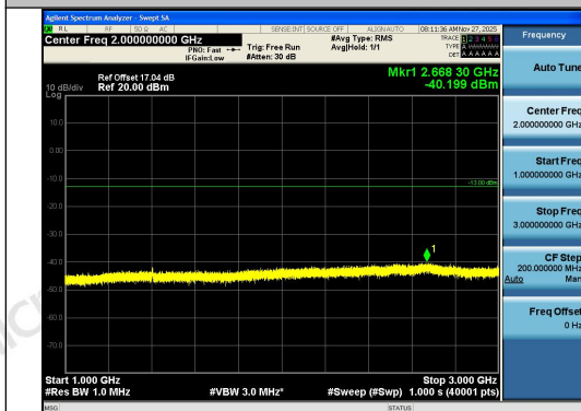
Band12-5MHz-16QAM-23035-25RB#0-1000~300
