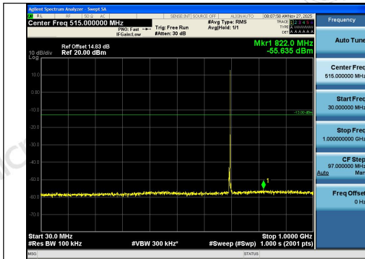
Band12-5MHz-QPSK-23035-1RB#24-30~1000-P ASS
