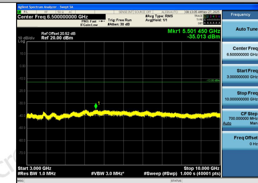
Band12-5MHz-QPSK-23095-1RB#0-3000~10000-
