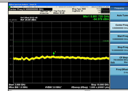
Band12-5MHz-16QAM-23095-1RB#0-3000~10000-
