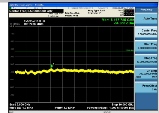
Band12-5MHz-16QAM-23035-1RB#24-3000~1000 0-PASS
