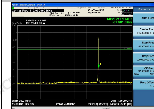
Band12-3MHz-16QAM-23165-15RB#0-30~1000-PASS
