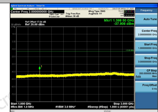
Band12-5MHz-16QAM-23035-1RB#0-1000~3000-
