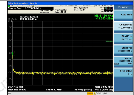
Band12-5MHz-16QAM-23035-1RB#24-0.15~30-P ASS
