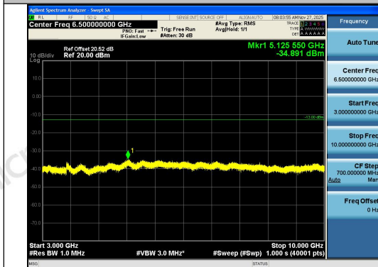
Band12-3MHz-QPSK-23165-15RB#0-3000~1000 0-PASS
