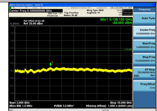
Band12-5MHz-16QAM-23035-25RB#0-3000~1000
