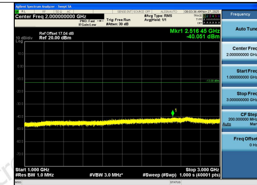
Band12-3MHz-QPSK-23165-15RB#0-1000~3000-PASS
