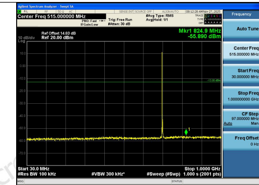
Band12-5MHz-QPSK-23095-1RB#0-30~1000-PAS
