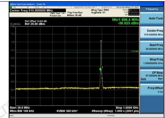
Band12-5MHz-QPSK-23035-25RB#0-30~1000-PA
