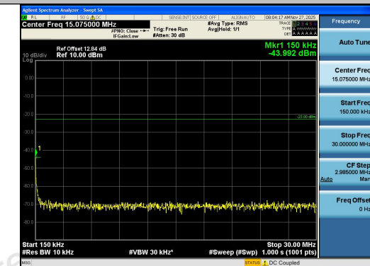
Band12-3MHz-16QAM-23165-15RB#0-0.15~30-P ASS
