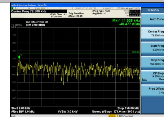
Band12-10MHz-QPSK-23130-1RB#49-0.009~0.15 -PASS
