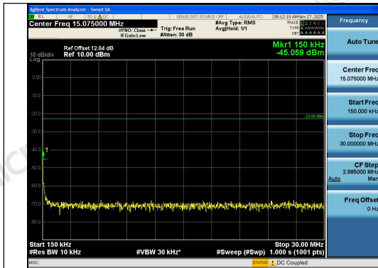
Band12-5MHz-QPSK-23095-1RB#0-0.15~30-PAS
