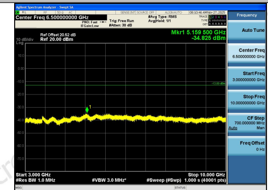
Band12-5MHz-QPSK-23035-25RB#0-3000~10000
