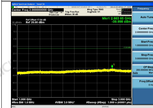
Band12-5MHz-QPSK-23035-25RB#0-1000~3000-
