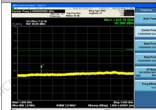
Band12-5MHz-16QAM-23095-1RB#0-1000~3000-
