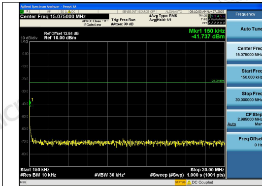
Band12-5MHz-QPSK-23035-25RB#0-0.15~30-PA
