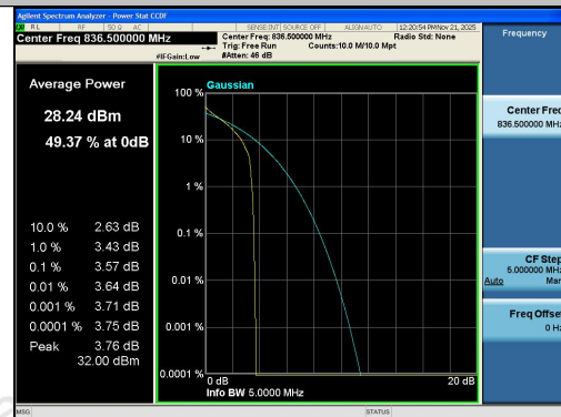
Band26(824-849)-5MHz-QPSK-26915-1RB#0-PA
