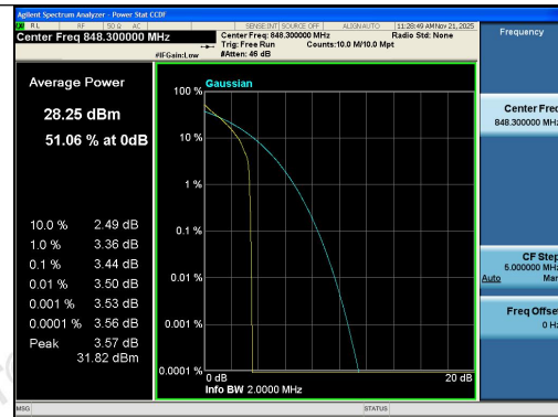
Band26(824-849)-1.4MHz-QPSK-27033-1RB#0-PASS
