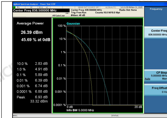
Band26(824-849)-5MHz-16QAM-26915-25RB#0-P
