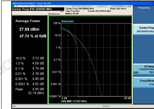
Band26(824-849)-10MHz-16QAM-26915-1RB#0-P
