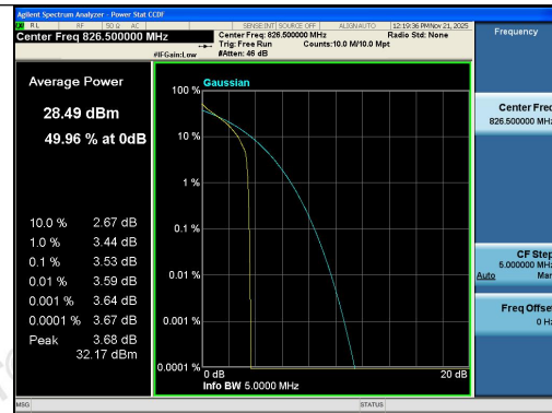
Band26(824-849)-5MHz-QPSK-26815-1RB#0-PA
