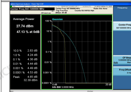
Band26(824-849)-3MHz-16QAM-27025-1RB#0-P ASS
