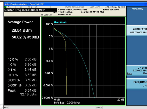
Band26(824-849)-10MHz-QPSK-26840-1RB#0-P
