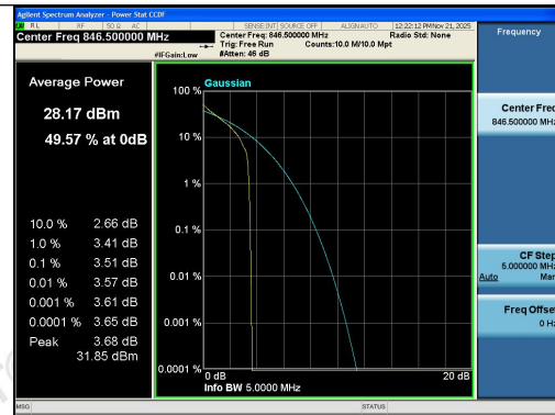
Band26(824-849)-5MHz-QPSK-27015-1RB#0-PA
