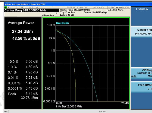
Band26(824-849)-1.4MHz-QPSK-27033-6RB#0-PASS
