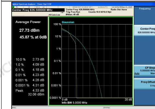
Band26(824-849)-5MHz-16QAM-26815-1RB#0-P
