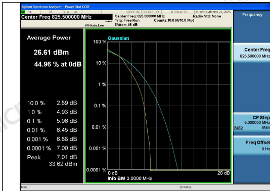
Band26(824-849)-3MHz-16QAM-26805-15RB#0-P ASS
