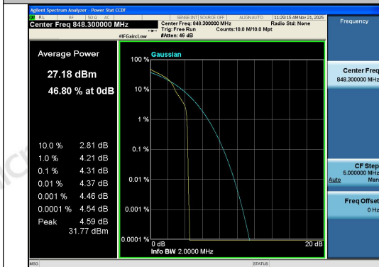
Band26(824-849)-1.4MHz-16QAM-27033-1RB#0-PASS
