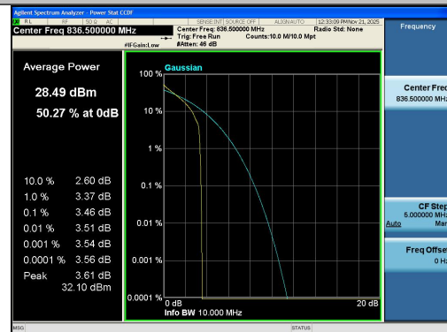
Band26(824-849)-10MHz-QPSK-26915-1RB#0-P
