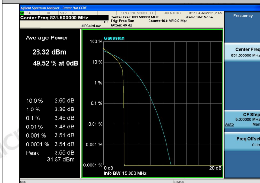
Band26(824-849)-15MHz-QPSK-26865-1RB#0-P
