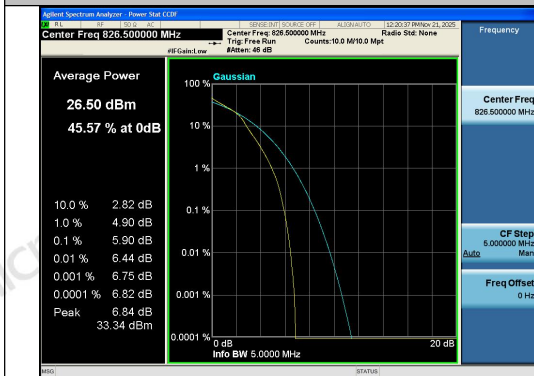
Band26(824-849)-5MHz-16QAM-26815-25RB#0-P
