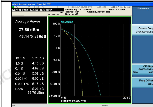
Band26(824-849)-10MHz-QPSK-26915-50RB#0-P
