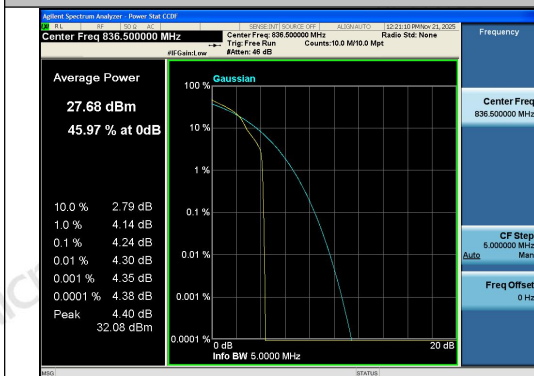
Band26(824-849)-5MHz-16QAM-26915-1RB#0-P
