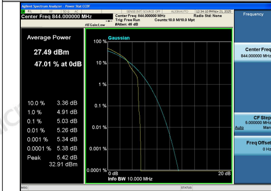
Band26(824-849)-10MHz-16QAM-26990-1RB#0-P
