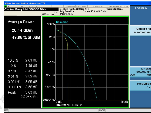
Band26(824-849)-10MHz-QPSK-26990-1RB#0-P
