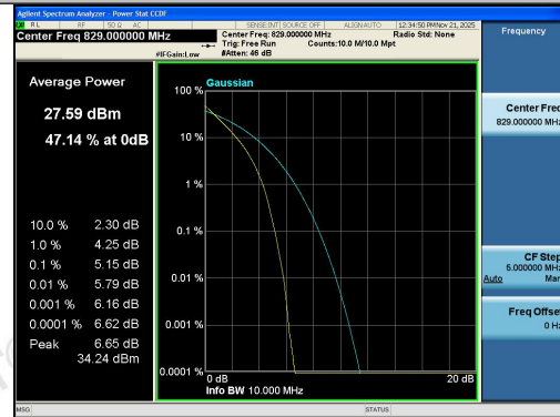
Band26(824-849)-10MHz-QPSK-26840-50RB#0-P
