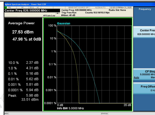
Band26(824-849)-5MHz-QPSK-26815-25RB#0-P
