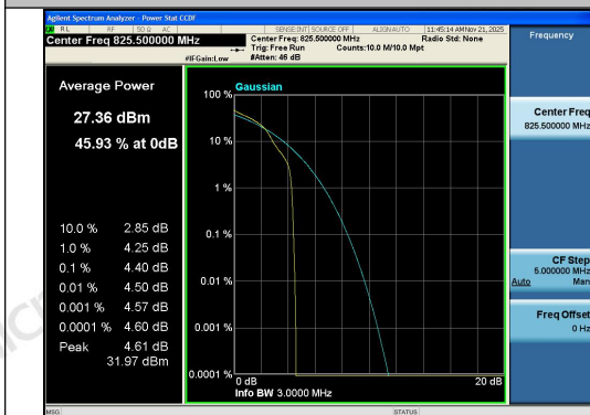
Band26(824-849)-3MHz-16QAM-26805-1RB#0-PASS
