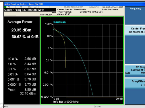
Band26(824-849)-3MHz-QPSK-27025-1RB#0-PA SS
