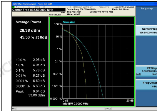
Band26(824-849)-1.4MHz-16QAM-26915-6RB#0-PASS
