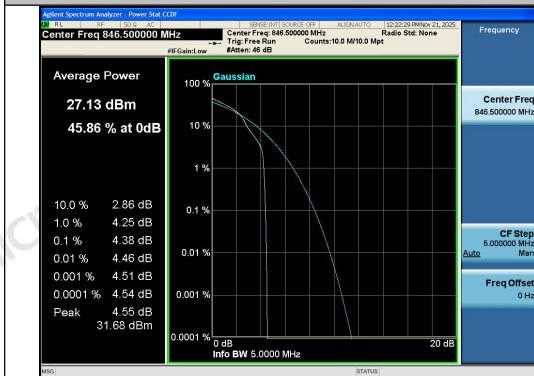
Band26(824-849)-5MHz-16QAM-27015-1RB#0-P
