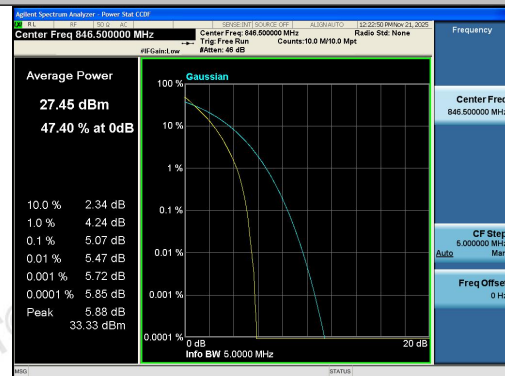
Band26(824-849)-5MHz-QPSK-27015-25RB#0-P
