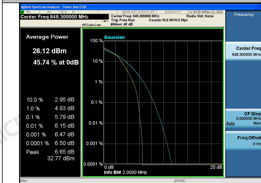
Band26(824-849)-1.4MHz-16QAM-27033-6RB#0-PASS
