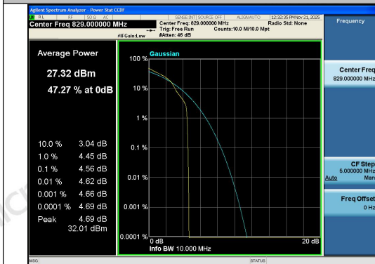
Band26(824-849)-10MHz-16QAM-26840-1RB#0-P
