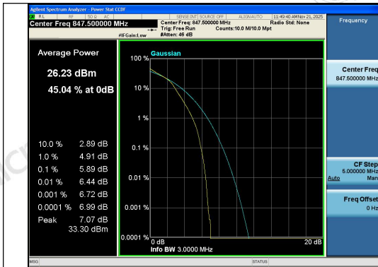
Band26(824-849)-3MHz-16QAM-27025-15RB#0-P
