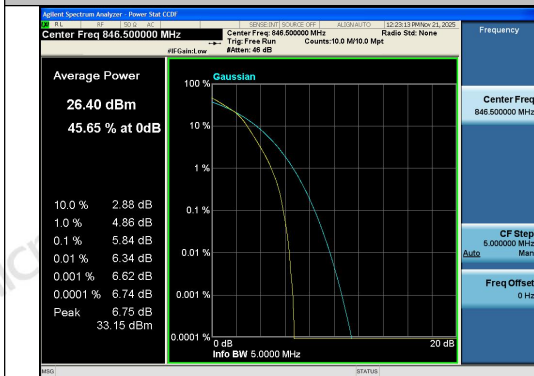
Band26(824-849)-5MHz-16QAM-27015-25RB#0-P
