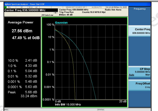
Band26(824-849)-15MHz-QPSK-26915-75RB#0-P ASS
