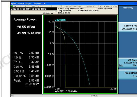
Band26(824-849)-15MHz-QPSK-26965-1RB#0-P ASS
