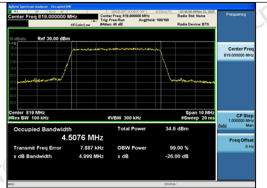
Band26(814-824)-5MHz-16QAM-26740-25RB#0-P ASS
