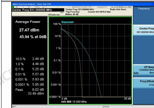
Band26(824-849)-15MHz-QPSK-26865-75RB#0-P ASS
