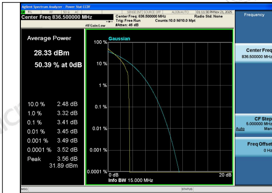
Band26(824-849)-15MHz-QPSK-26915-1RB#0-P ASS
