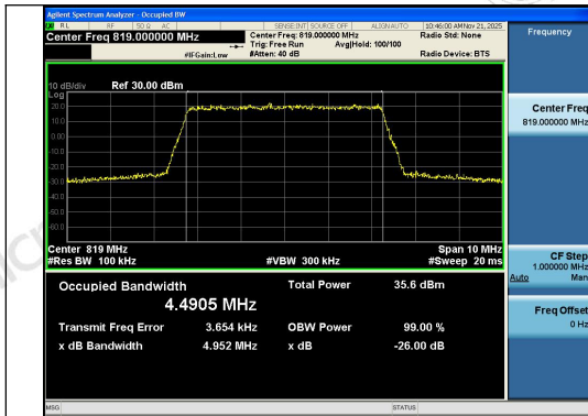
Band26(814-824)-5MHz-QPSK-26740-25RB#0-P ASS
