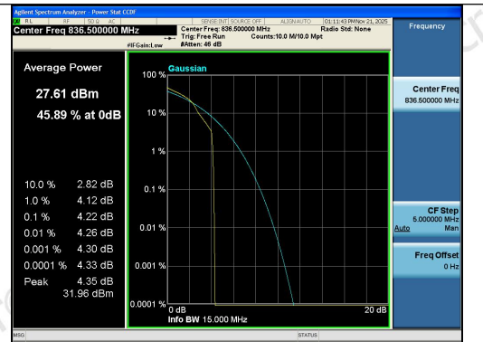
Band26(824-849)-15MHz-16QAM-26915-1RB#0-P ASS
