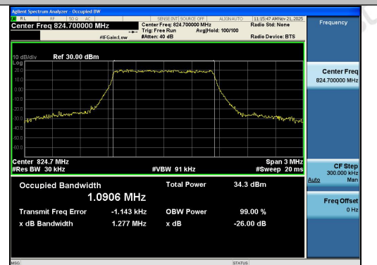
Band26(824-849)-1.4MHz-16QAM-26797-6RB#0-P PASS
