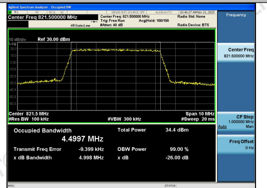
Band26(814-824)-5MHz-16QAM-26765-25RB#0-P ASS
