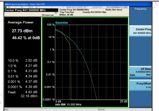
Band26(824-849)-15MHz-16QAM-26965-1RB#0-P ASS
