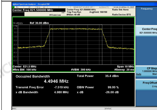
Band26(814-824)-5MHz-QPSK-26765-25RB#0-P ASS
