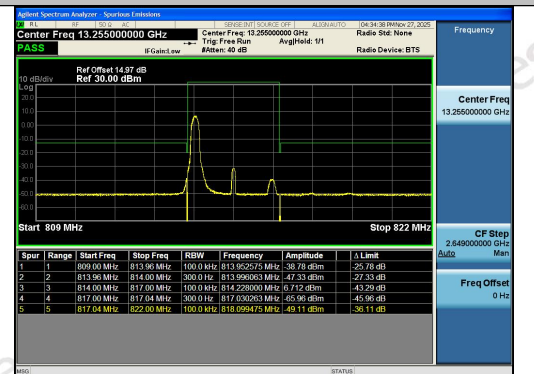
Band26(814-824)-3MHz-QPSK-26705-1RB#0-PA SS
