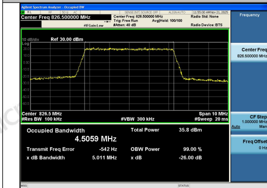
Band26(824-849)-5MHz-QPSK-26815-25RB#0-P ASS
