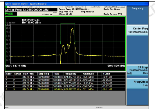
Band26(814-824)-1.4MHz-QPSK-26783-1RB#5-P ASS
