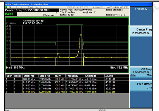
Band26(814-824)-3MHz-QPSK-26705-1RB#14-P ASS
