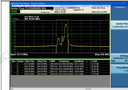
Band26(814-824)-1.4MHz-16QAM-26783-1RB#5-P PASS
