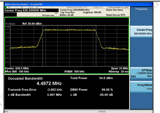
Band26(824-849)-5MHz-16QAM-26815-25RB#0-P ASS
