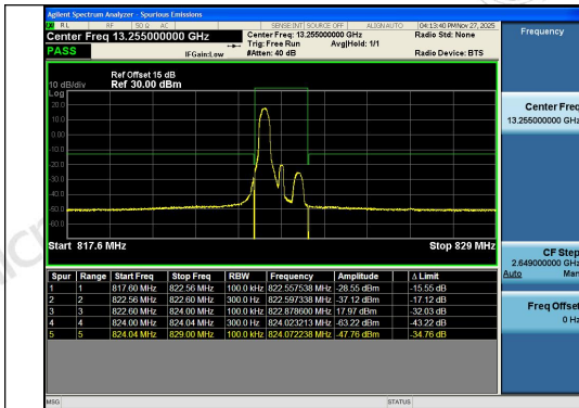
Band26(814-824)-1.4MHz-16QAM-26783-1RB#0-P PASS
