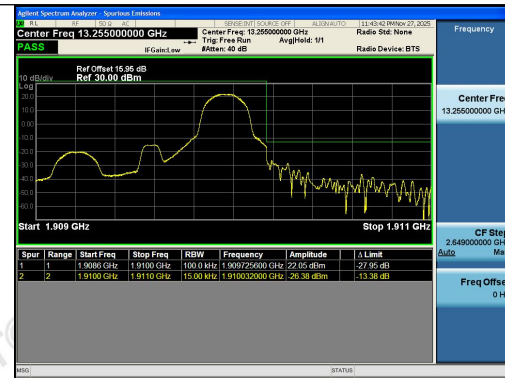
Band2-1.4MHz-16QAM-19193-1RB#5-PASS
