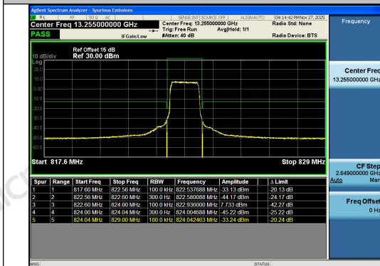
Band26(814-824)-1.4MHz-16QAM-26783-6RB#0-P PASS
