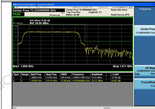
Band2-1.4MHz-QPSK-19193-6RB#0-PASS
