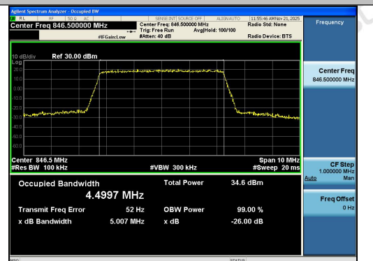
Band26(824-849)-5MHz-16QAM-27015-25RB#0-P ASS
