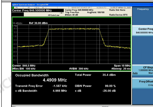
Band26(824-849)-5MHz-QPSK-27015-25RB#0-P ASS
