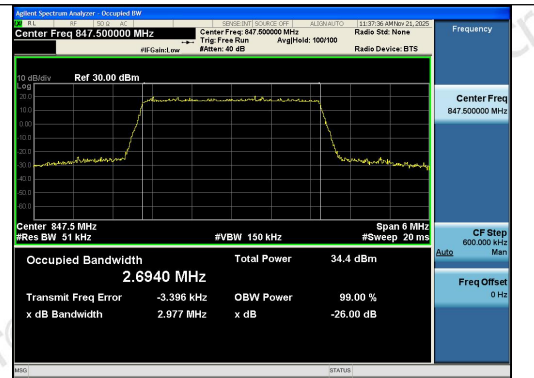
Band26(824-849)-3MHz-16QAM-27025-15RB#0-P ASS
