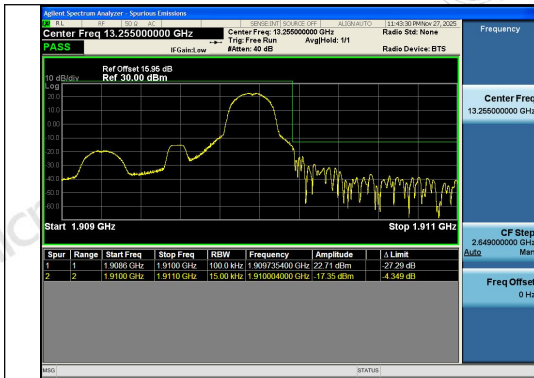
Band2-1.4MHz-QPSK-19193-1RB#5-PASS
