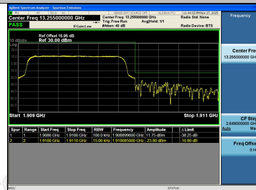
Band2-1.4MHz-16QAM-19193-6RB#0-PASS
