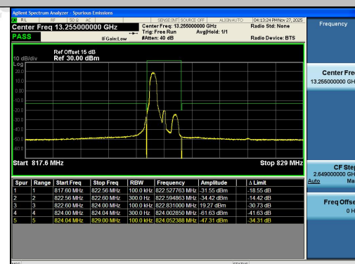
Band26(814-824)-1.4MHz-QPSK-26783-1RB#0-PASS
