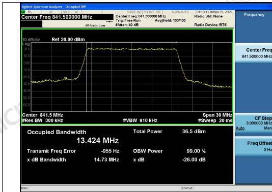
Band26(824-849)-15MHz-QPSK-26965-75RB#0-P ASS
