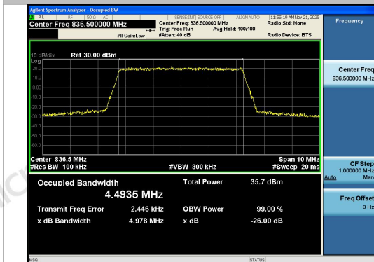
Band26(824-849)-5MHz-QPSK-26915-25RB#0-P ASS
