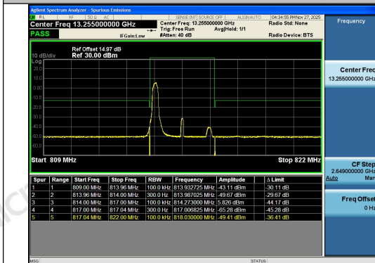
Band26(814-824)-3MHz-16QAM-26705-1RB#0-PA SS
