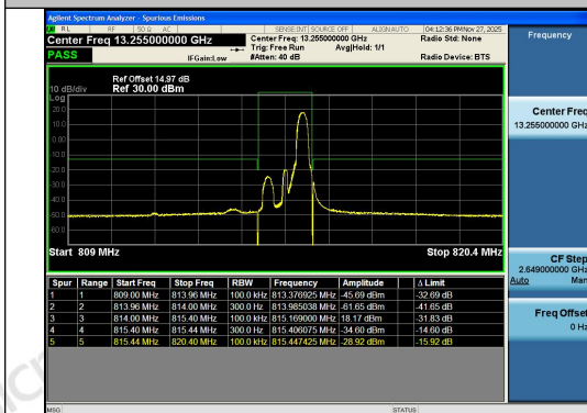
Band26(814-824)-1.4MHz-16QAM-26697-1RB#5-PASS
