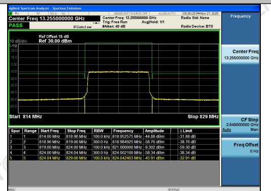
Band26(814-824)-5MHz-QPSK-26765-25RB#0-P
