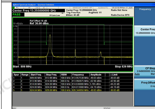
Band26(814-824)-10MHz-16QAM-26740-1RB#0-P
