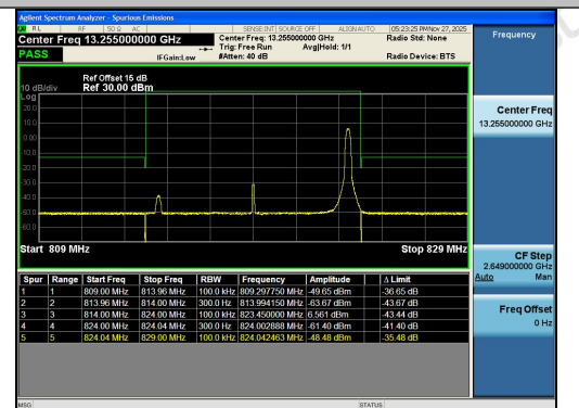
Band26(814-824)-10MHz-QPSK-26740-1RB#49-PASS
