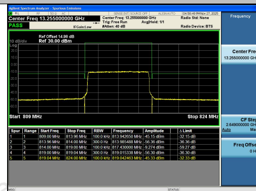
Band26(814-824)-5MHz-QPSK-26715-25RB#0-P
