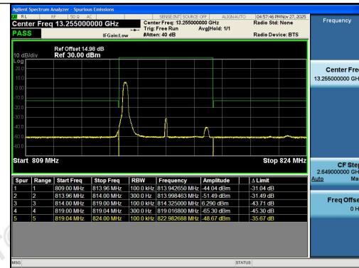
Band26(814-824)-5MHz-QPSK-26715-1RB#0-PA
