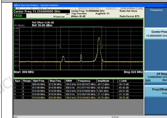
Band26(814-824)-5MHz-16QAM-26715-1RB#24-P
