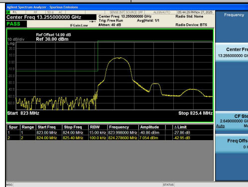
Band26(824-849)-1.4MHz-QPSK-26797-1RB#0-PASS
