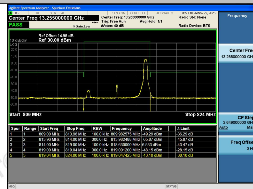
Band26(814-824)-5MHz-QPSK-26715-1RB#24-P
