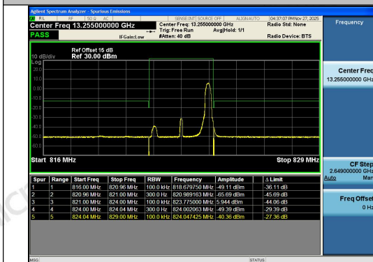
Band26(814-824)-3MHz-16QAM-26775-1RB#14-P
