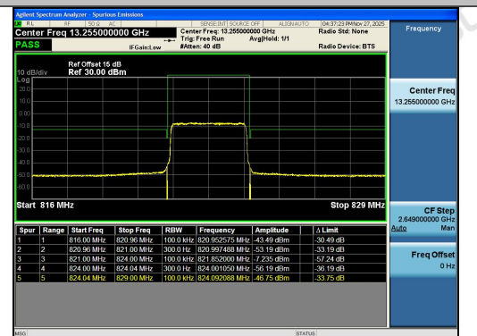
Band26(814-824)-3MHz-QPSK-26775-15RB#0-P
