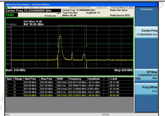
Band26(814-824)-3MHz-QPSK-26775-1RB#0-PA
