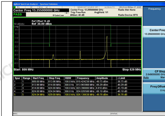
Band26(814-824)-10MHz-16QAM-26740-1RB#49-
