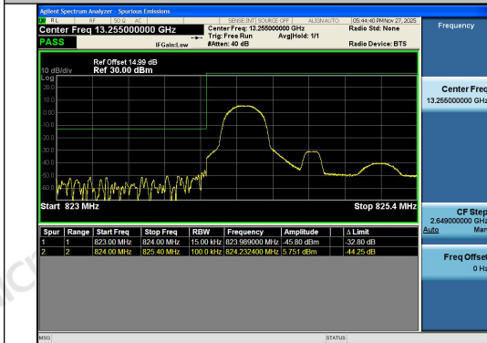
Band26(824-849)-1.4MHz-16QAM-26797-1RB#0-
