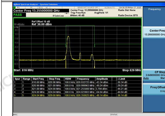
Band26(814-824)-3MHz-16QAM-26775-1RB#0-PA
