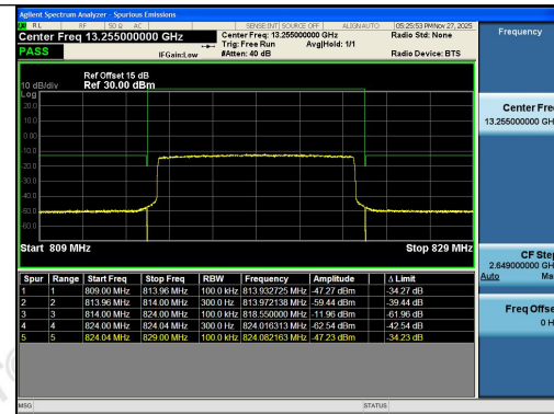
Band26(814-824)-10MHz-QPSK-26740-50RB#0-
