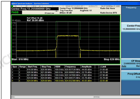
Band26(814-824)-3MHz-16QAM-26775-15RB#0-P
