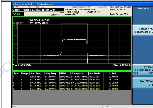
Band26(814-824)-3MHz-16QAM-26705-15RB#0-P
