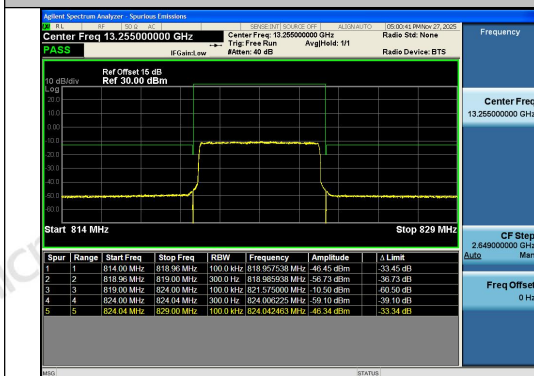
Band26(814-824)-5MHz-16QAM-26765-25RB#0-P
