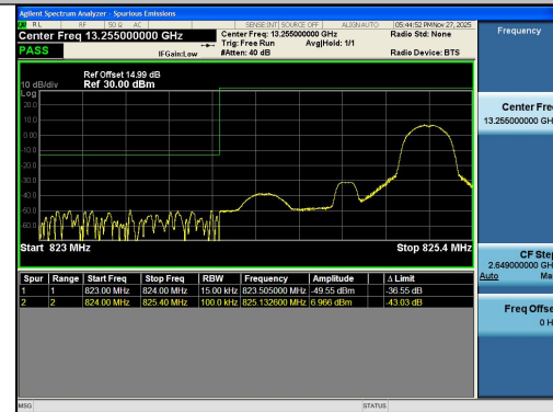
Band26(824-849)-1.4MHz-QPSK-26797-1RB#5-P
