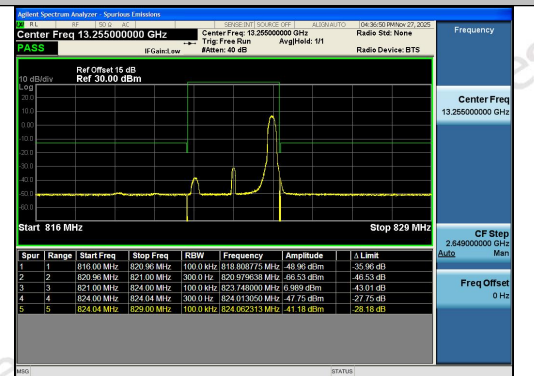
Band26(814-824)-3MHz-QPSK-26775-1RB#14-P
