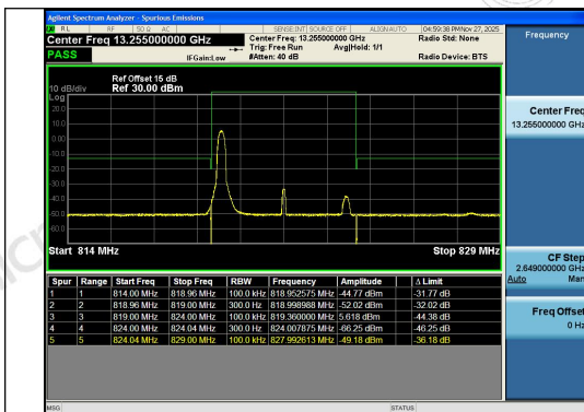
Band26(814-824)-5MHz-16QAM-26765-1RB#0-PA
