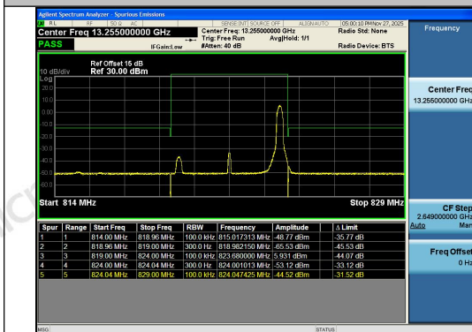
Band26(814-824)-5MHz-16QAM-26765-1RB#24-P
