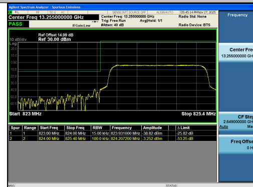
Band26(824-849)-1.4MHz-QPSK-26797-6RB#0-P
