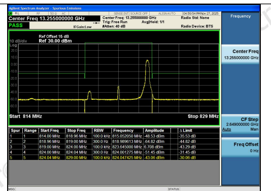
Band26(814-824)-5MHz-QPSK-26765-1RB#24-P
