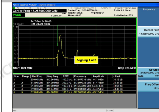
Band26(814-824)-5MHz-16QAM-26715-1RB#0-PA
