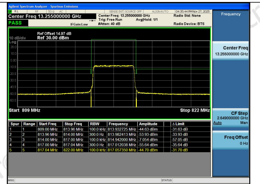
Band26(814-824)-3MHz-QPSK-26705-15RB#0-P
