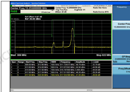
Band26(814-824)-3MHz-16QAM-26705-1RB#14-P
