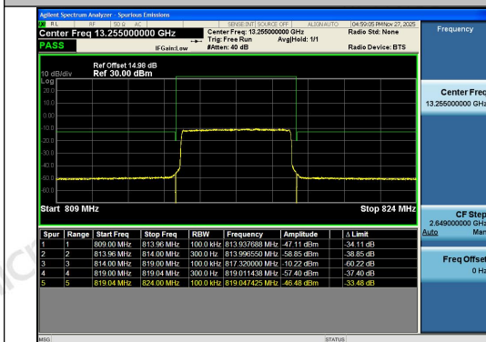
Band26(814-824)-5MHz-16QAM-26715-25RB#0-P
