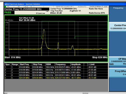
Band26(814-824)-5MHz-QPSK-26765-1RB#0-PA
