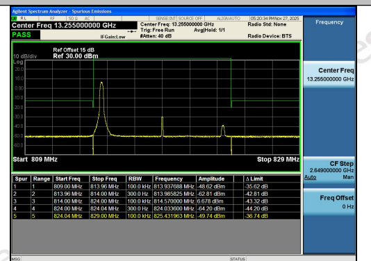
Band26(814-824)-10MHz-QPSK-26740-1RB#0-P
