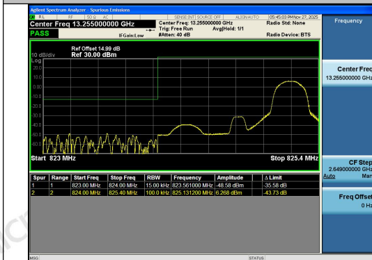
Band26(824-849)-1.4MHz-16QAM-26797-1RB#5-
