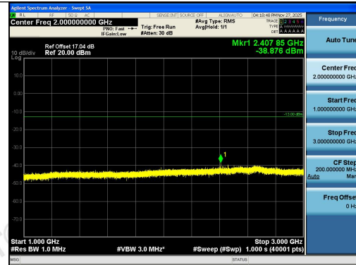
Band26(814-824)-1.4MHz-16QAM-26697-1RB#5- 1000~3000-PASS
