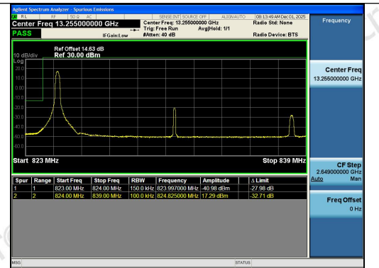
Band26(824-849)-15MHz-QPSK-26865-1RB#0-P
