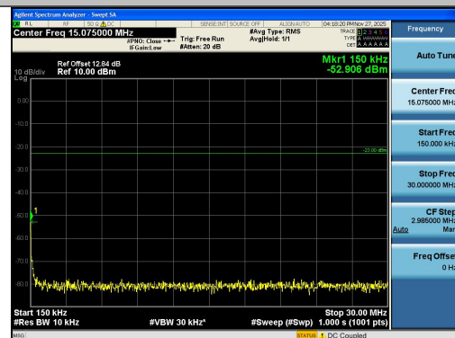
Band26(814-824)-1.4MHz-16QAM-26697-1RB#5- 0.15~30-PASS
