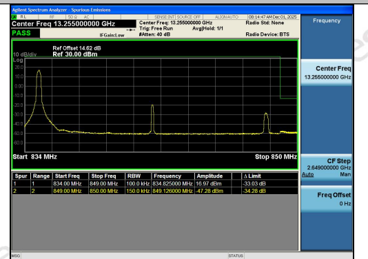
Band26(824-849)-15MHz-QPSK-26965-1RB#0-P
