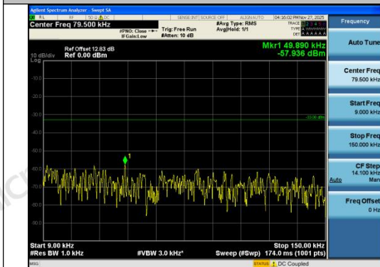
Band26(814-824)-1.4MHz-16QAM-26697-1RB#0-0. 0.009~0.15-PASS
