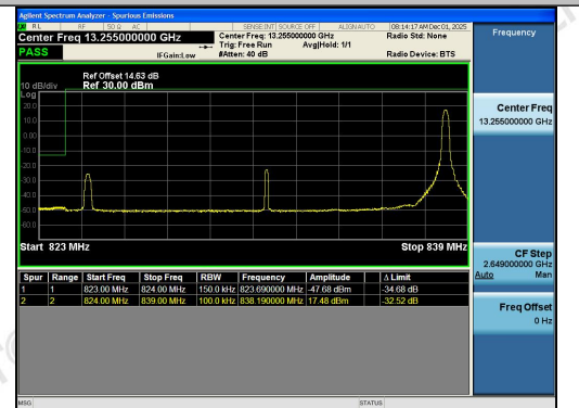
Band26(824-849)-15MHz-QPSK-26865-1RB#74-
