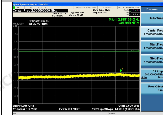
Band26(814-824)-1.4MHz-QPSK-26697-1RB#5-1 000~3000-PASS
