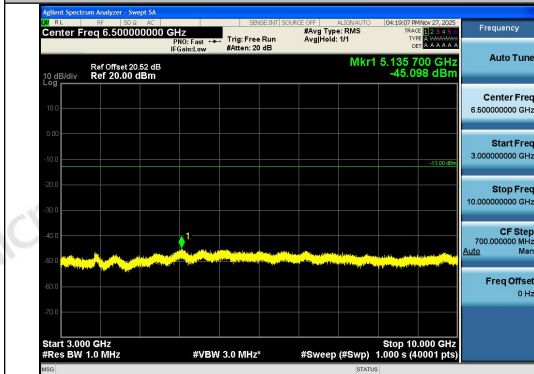
Band26(814-824)-1.4MHz-16QAM-26697-1RB#5- 3000~10000-PASS
