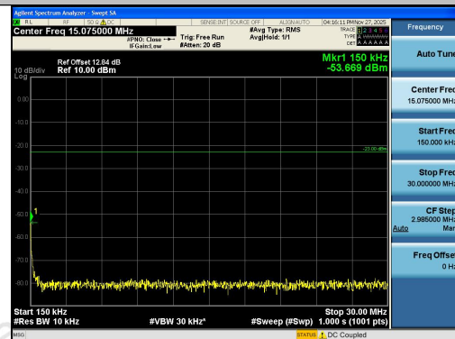
Band26(814-824)-1.4MHz-16QAM-26697-1RB#0-0. 0.15~30-PASS
