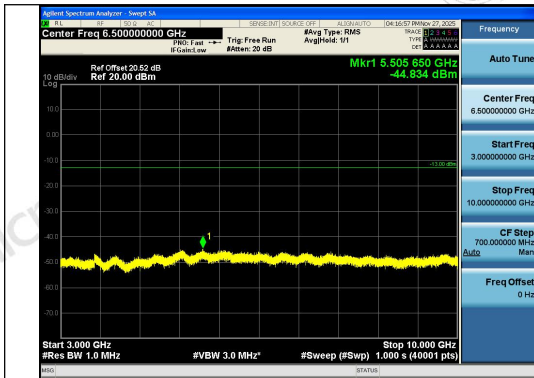
Band26(814-824)-1.4MHz-16QAM-26697-1RB#0- 3000~10000-PASS
