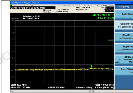
Band26(814-824)-1.4MHz-16QAM-26697-1RB#5- 30~1000-PASS
