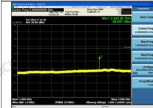
Band26(814-824)-1.4MHz-QPSK-26697-1RB#0-1 000~3000-PASS
