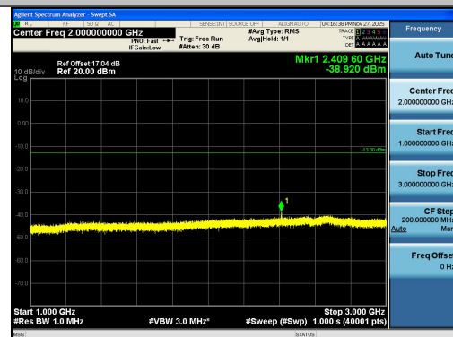
Band26(814-824)-1.4MHz-16QAM-26697-1RB#0-0. 1000~3000-PASS
