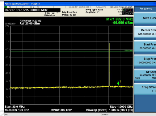
Band26(814-824)-1.4MHz-QPSK-26697-6RB#0-3 0~1000-PASS
