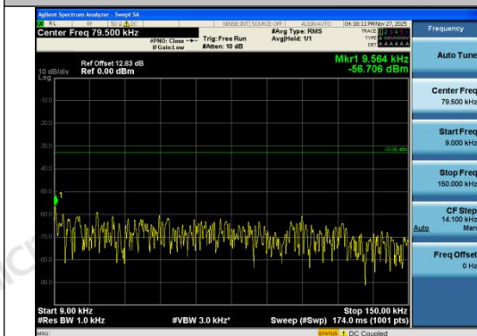
Band26(814-824)-1.4MHz-16QAM-26697-1RB#5- 0.009~0.15-PASS
