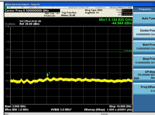
Band26(814-824)-1.4MHz-QPSK-26697-6RB#0-3 000~10000-PASS
