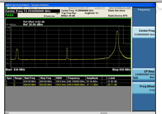
Band26(824-849)-15MHz-QPSK-26965-1RB#74-
