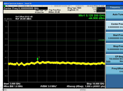
Band26(814-824)-1.4MHz-QPSK-26697-1RB#5-3 000~10000-PASS
