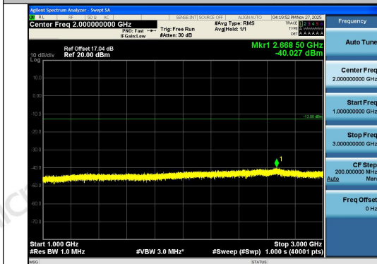
Band26(814-824)-1.4MHz-QPSK-26697-6RB#0-1 000~3000-PASS
