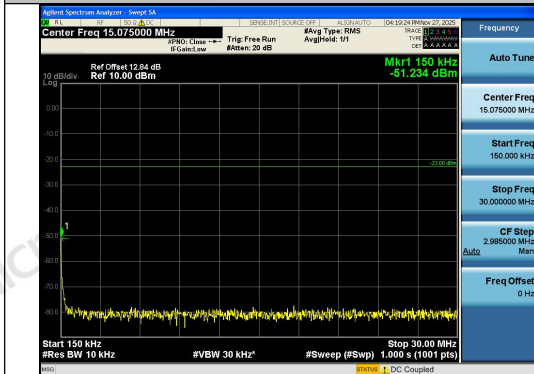
Band26(814-824)-1.4MHz-QPSK-26697-6RB#0-0. 15~30-PASS
