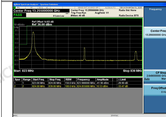
Band26(824-849)-15MHz-16QAM-26865-1RB#0-P
