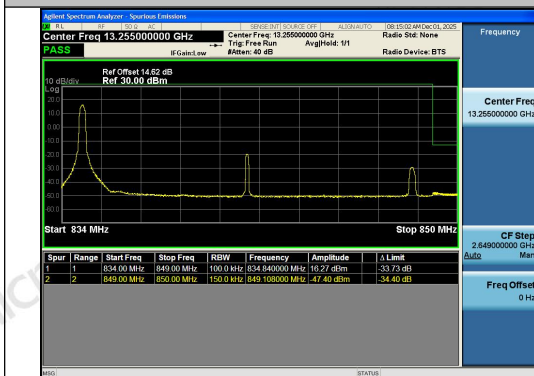
Band26(824-849)-15MHz-16QAM-26965-1RB#0-P
