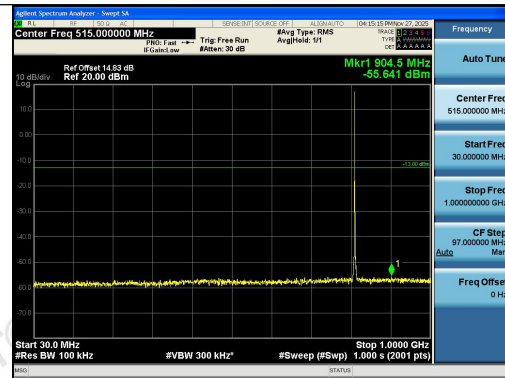
Band26(814-824)-1.4MHz-QPSK-26697-1RB#0-3 0~1000-PASS
