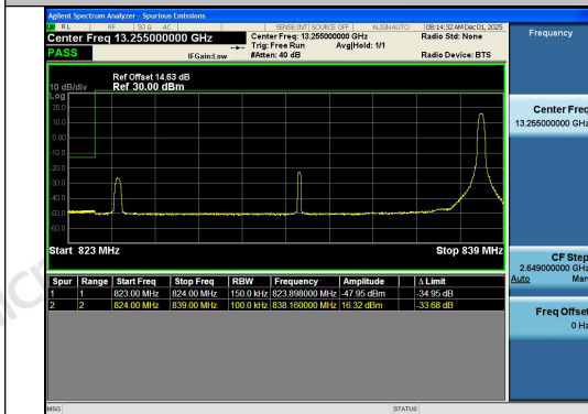
Band26(824-849)-15MHz-16QAM-26865-1RB#74-
