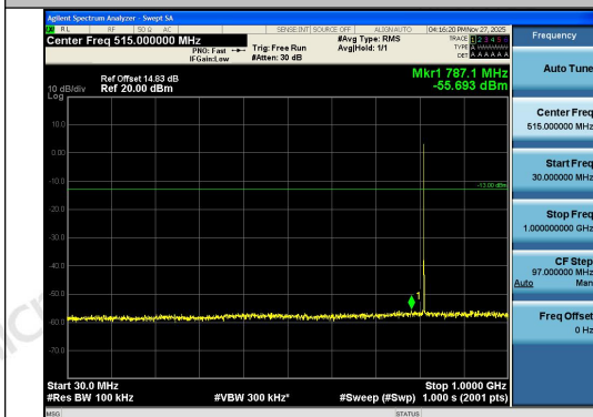
Band26(814-824)-1.4MHz-16QAM-26697-1RB#0-0. 30~1000-PASS
