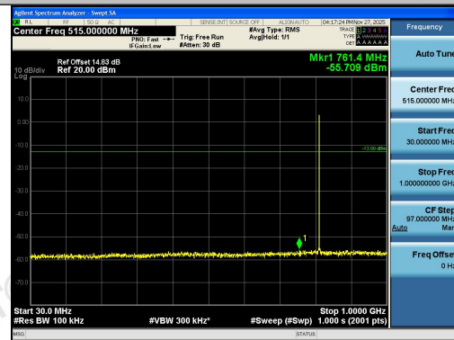
Band26(814-824)-1.4MHz-QPSK-26697-1RB#5-3 0~1000-PASS
