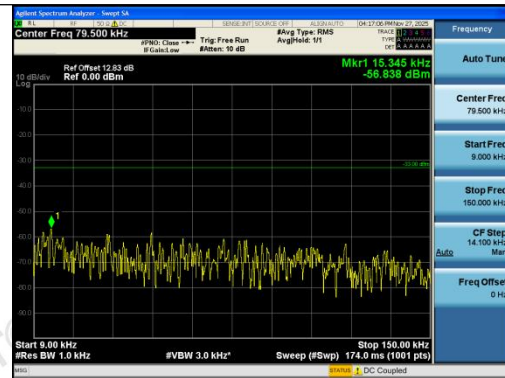
Band26(814-824)-1.4MHz-QPSK-26697-1RB#5-0. 009~0.15-PASS
