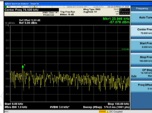
Band26(814-824)-1.4MHz-QPSK-26697-6RB#0-0. 009~0.15-PASS
