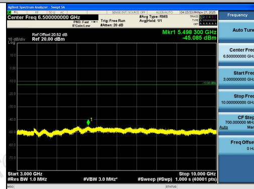
Band26(814-824)-1.4MHz-QPSK-26697-1RB#0-3 000~10000-PASS
