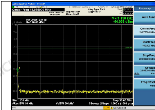
Band26(814-824)-1.4MHz-QPSK-26697-1RB#0-0. 15~30-PASS
