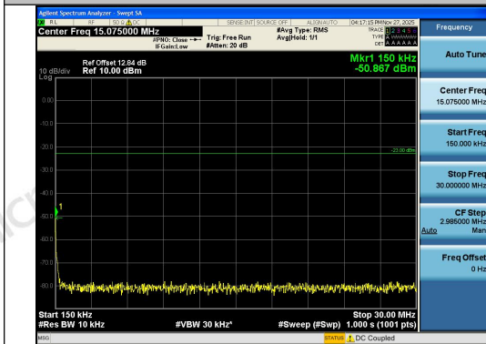
Band26(814-824)-1.4MHz-QPSK-26697-1RB#5-0. 15~30-PASS
