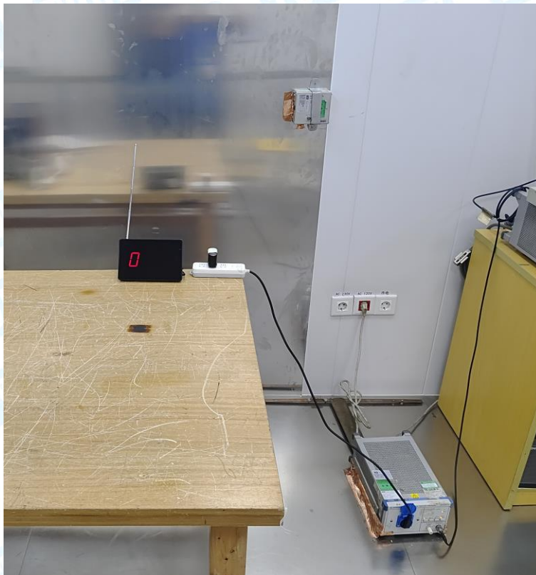
Photo of Setup for Radiated Emission (Below 1 GHz)
