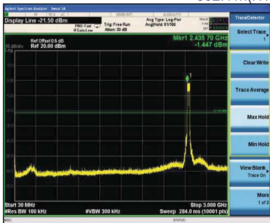
802.11n(HT40)-Highest channel
