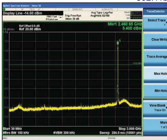
802.11b-Highest channel
