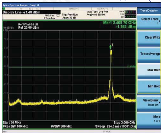
802.11n(HT40)-Lowest channel
