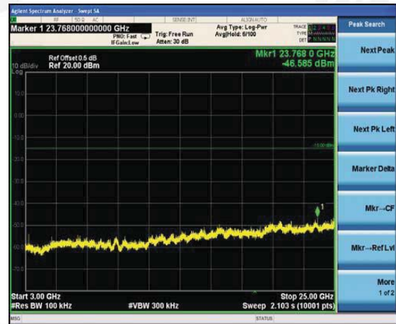
802.11b-Middle channel
