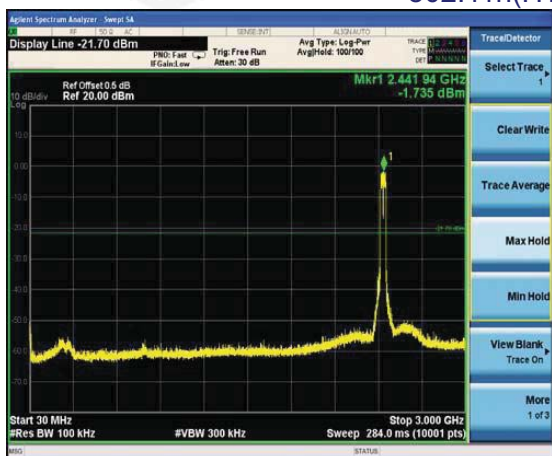
802.11n(HT40)-Middle channel
