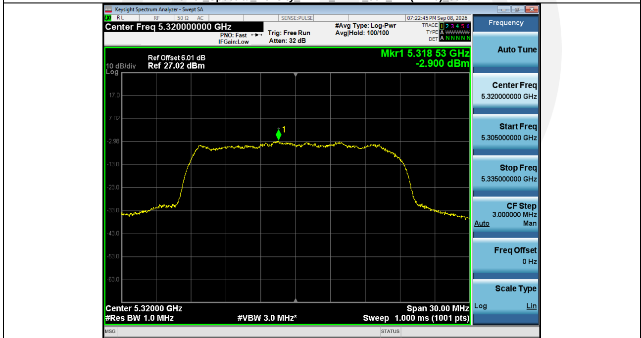
Power Spectral Density NVNT_ANT1_802_11n(HT20)_5320
