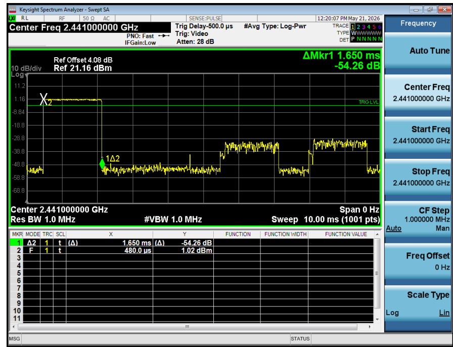
Dwell_Time_(Hopping)_NVNT_ANT1_2-DH3_2441_00_Accumulated
