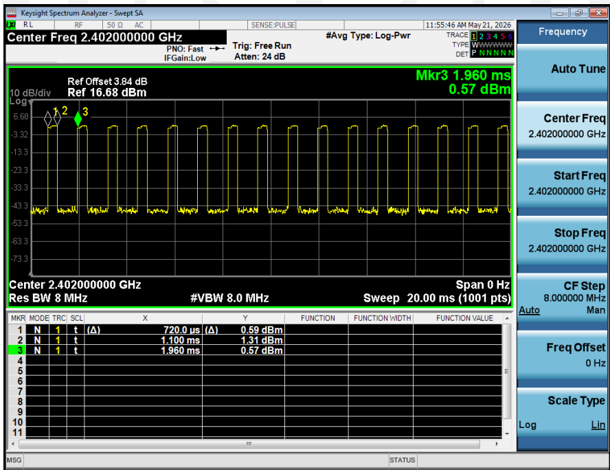
Duty_Cycle_NVNT_ANT1_3-DH1_2402
