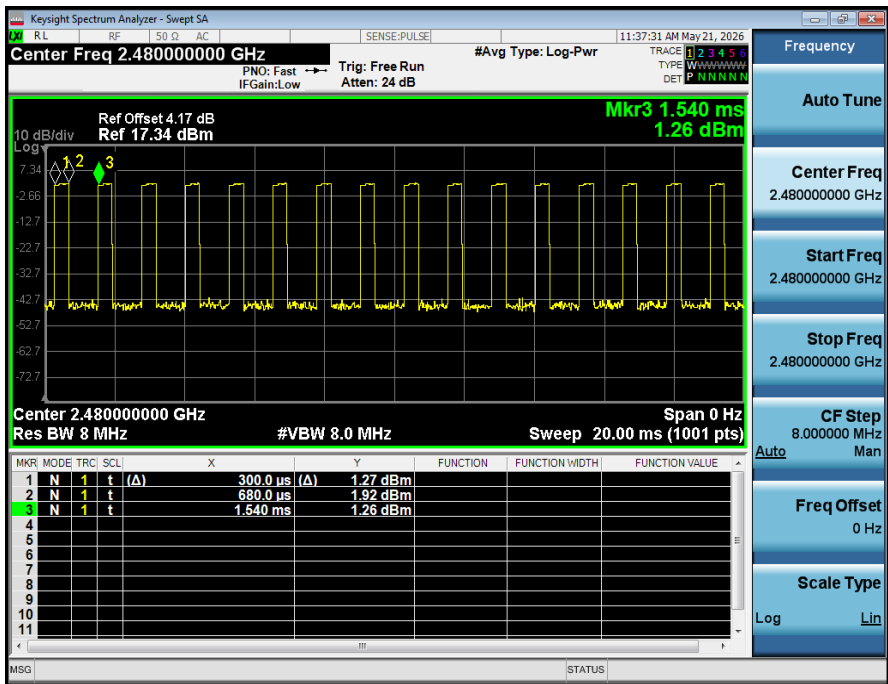
Duty_Cycle_NVNT_ANT1_2-DH1_2480
