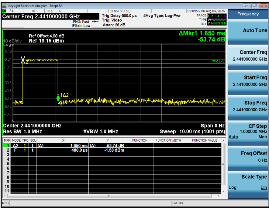
Dwell_Time_(Hopping)_NVNT_ANT1_3-DH3_2441_00_Accumulated
