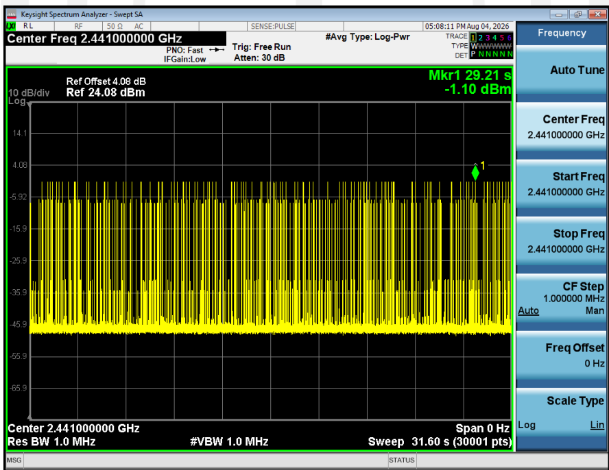
Dwell_Time_(Hopping)_NVNT_ANT1_2-DH5_2441_00_Accumulated
