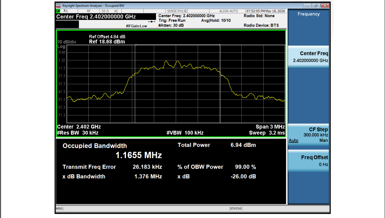
99%_Occupied_Bandwidth_NVNT_ANT1_2-DH1_2402_00
