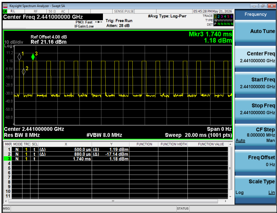
Duty_Cycle_NVNT_ANT1_1-DH1_2441
