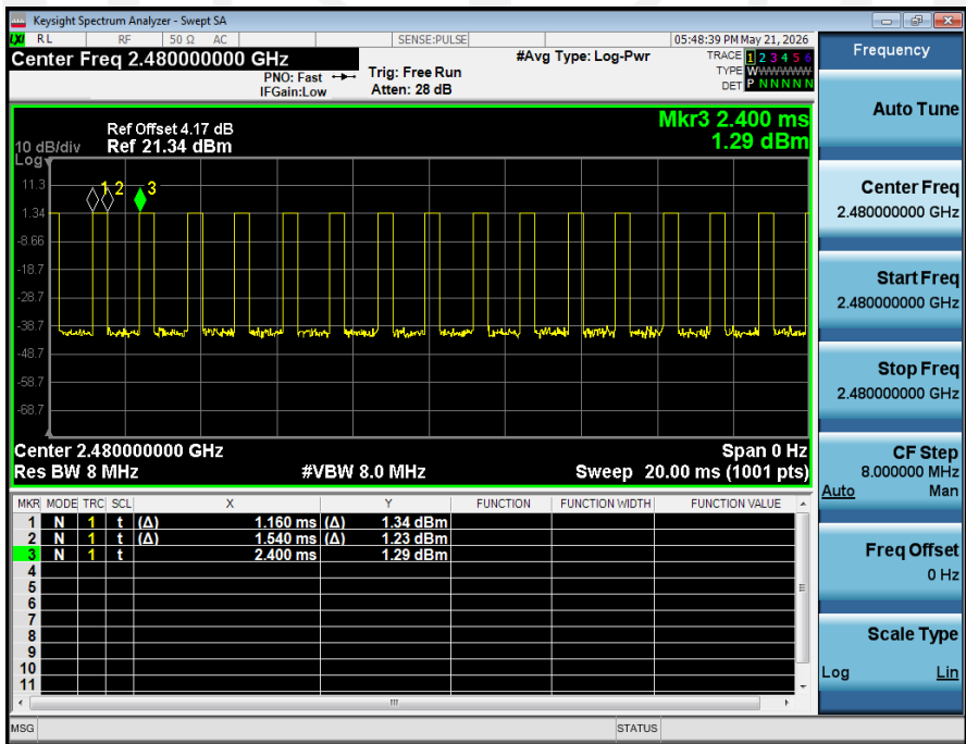
Duty_Cycle_NVNT_ANT1_1-DH1_2480
