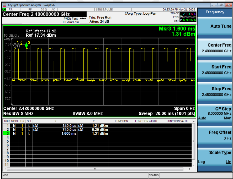
Duty_Cycle_NVNT_ANT1_3-DH1_2480
