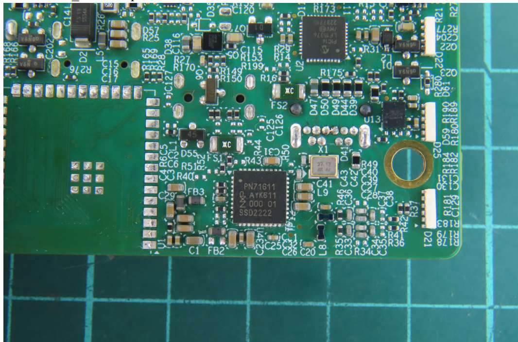
(20) EUT Photo _NFC Chip
