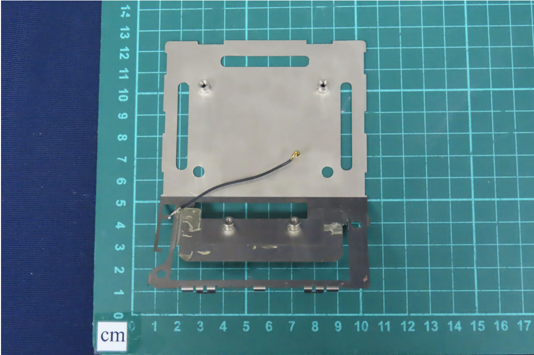
(25) EUT Photo _RF Antenna
