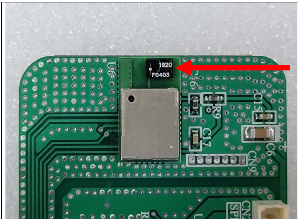
Chip Antenna in RF Module
