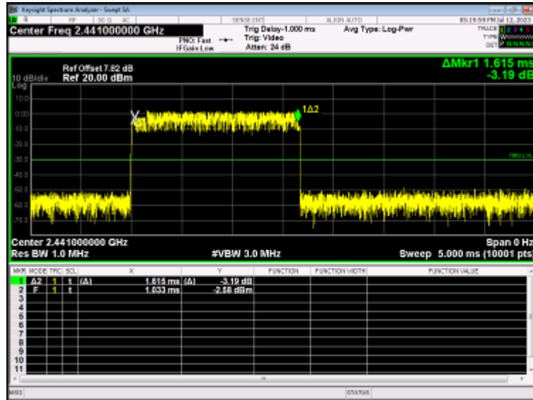
Dwell NVNT 2-DH3 2441MHz
