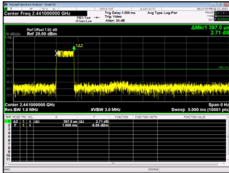
Dwell NVNT 1-DH1 2441MHz
