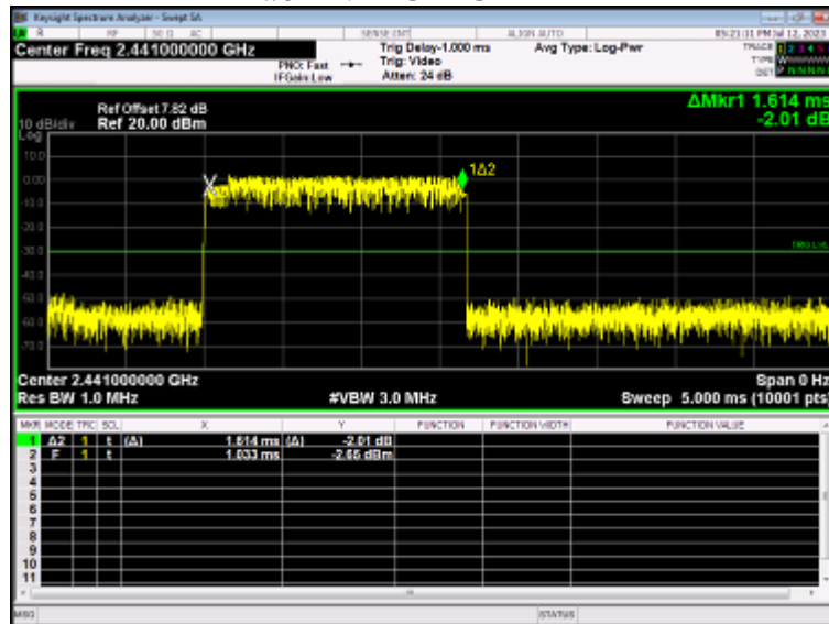
Dwell NVNT 3-DH3 2441MHz
