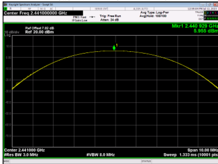
Power NVNT 1-DH5 2441MHz Ant1
