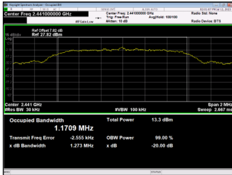
OBW NVNT 3-DH5 2441MHz Ant1
