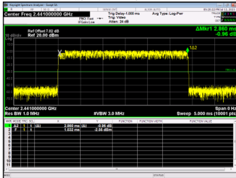
Dwell NVNT 2-DH5 2441MHz
