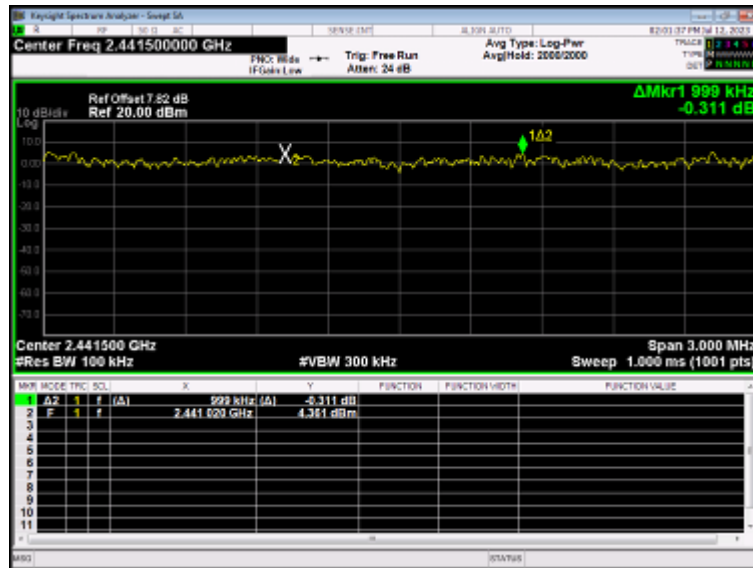
CFS NVNT 3-DH5 2441MHz
