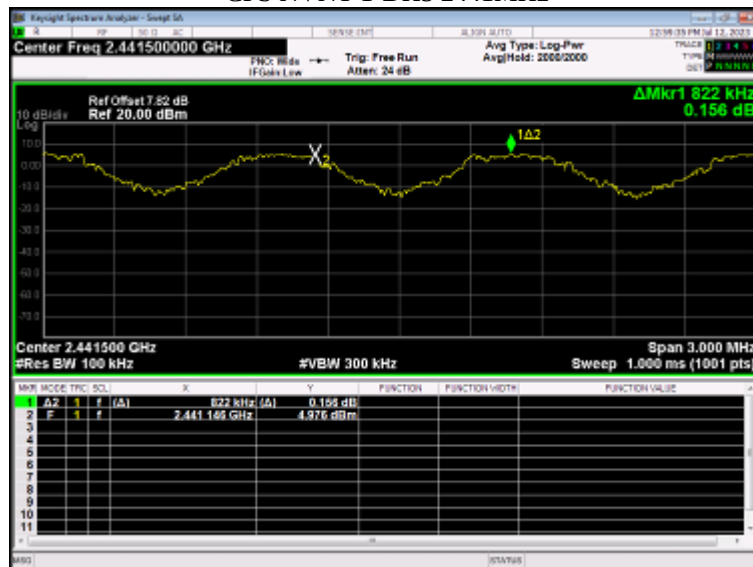
CFS NVNT 1-DH5 2441MHz
