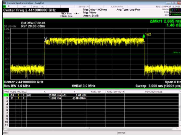
Dwell NVNT 3-DH5 2441MHz
