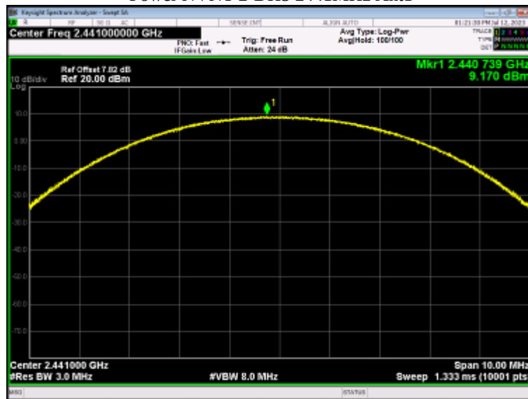
Power NVNT 2-DH5 2441MHz Ant1
