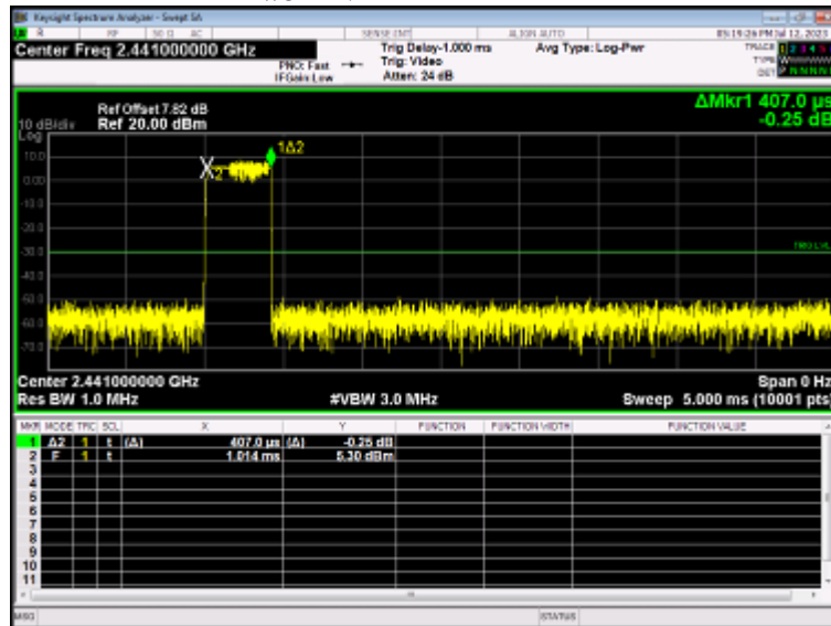
Dwell NVNT 2-DH1 2441MHz
