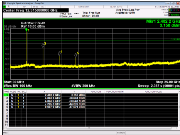
Tx. Spurious NVNT 2-DH5 2402MHz Ant1 Emission
