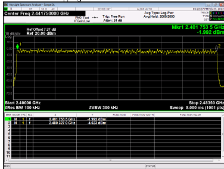
Hopping No. NVNT 3-DH5 2441MHz
