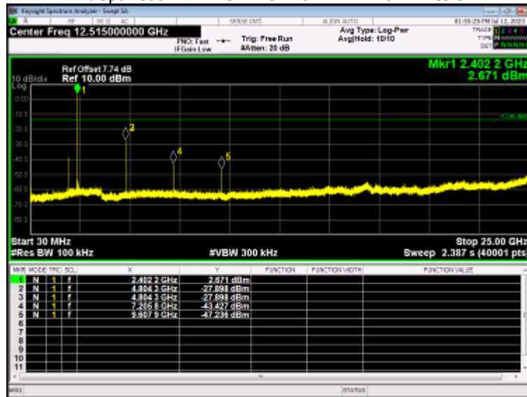
Tx. Spurious NVNT 3-DH5 2402MHz Ant1 Emission
