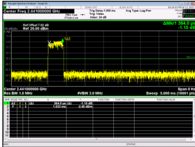
Dwell NVNT 3-DH1 2441MHz
