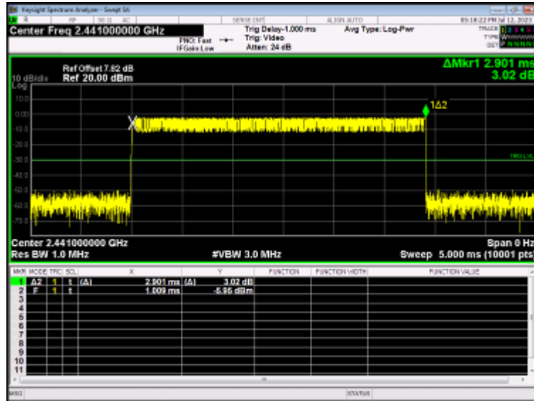
Dwell NVNT 1-DH5 2441MHz
