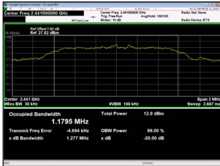
OBW NVNT 2-DH5 2441MHz Ant1
