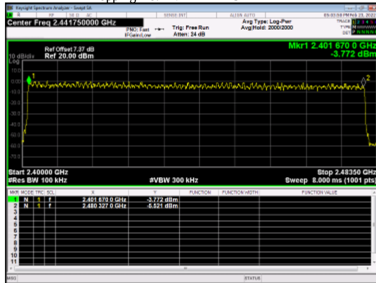
Hopping No. NVNT 2-DH5 2441MHz
