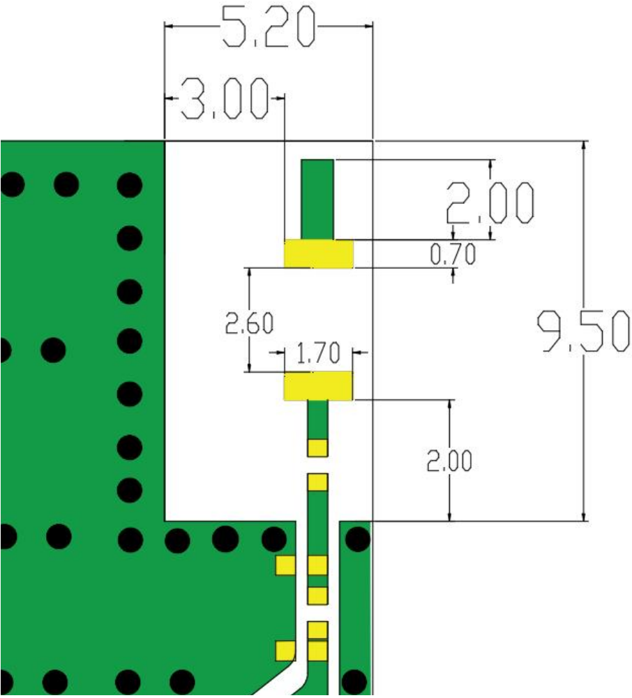
6-2-2. Matching Circuit:
