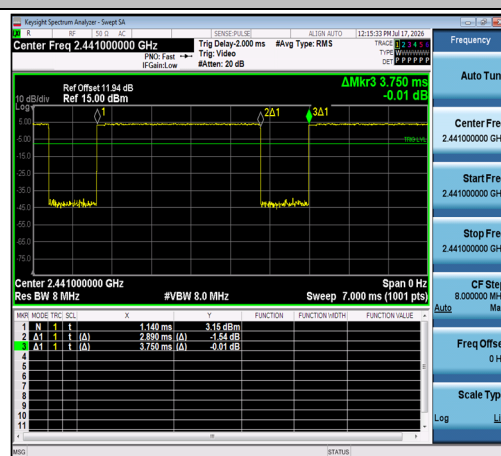
NTNV-2DH5-Ant1-2441
