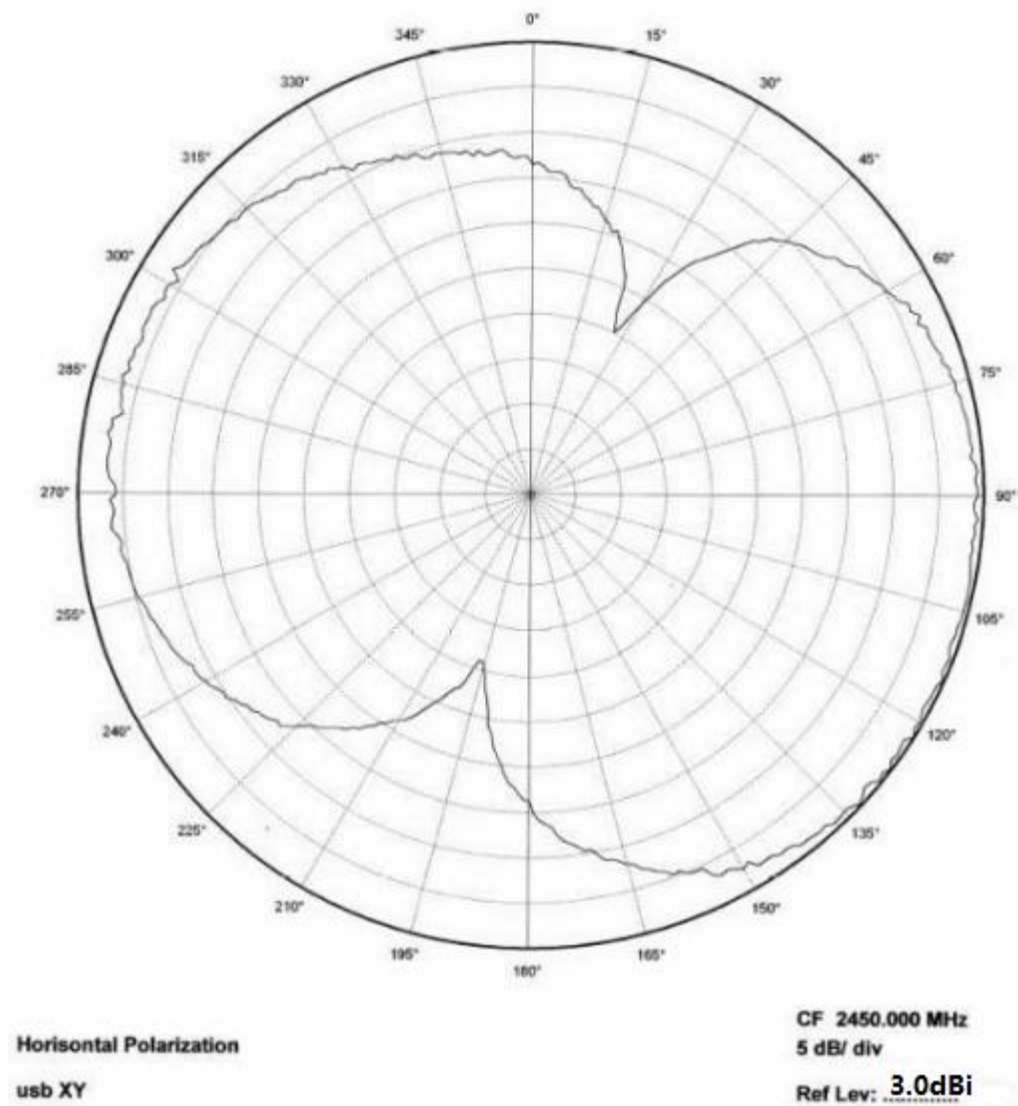
Figure 8: WLT5283M XY Plane
