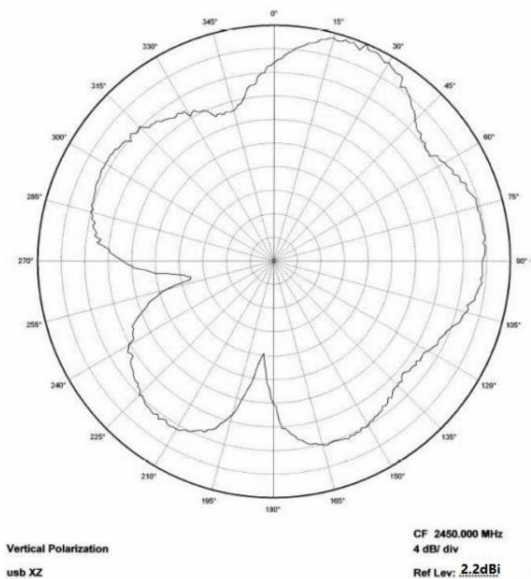
Figure 9: WLT5283M XZ Plane
