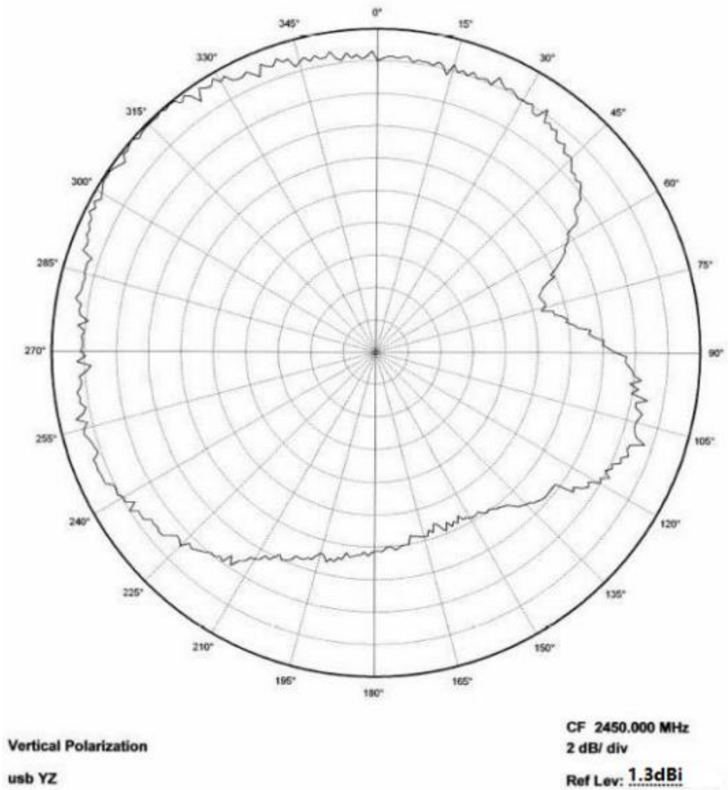
Figure 11: WLT5283M YZ Plane
