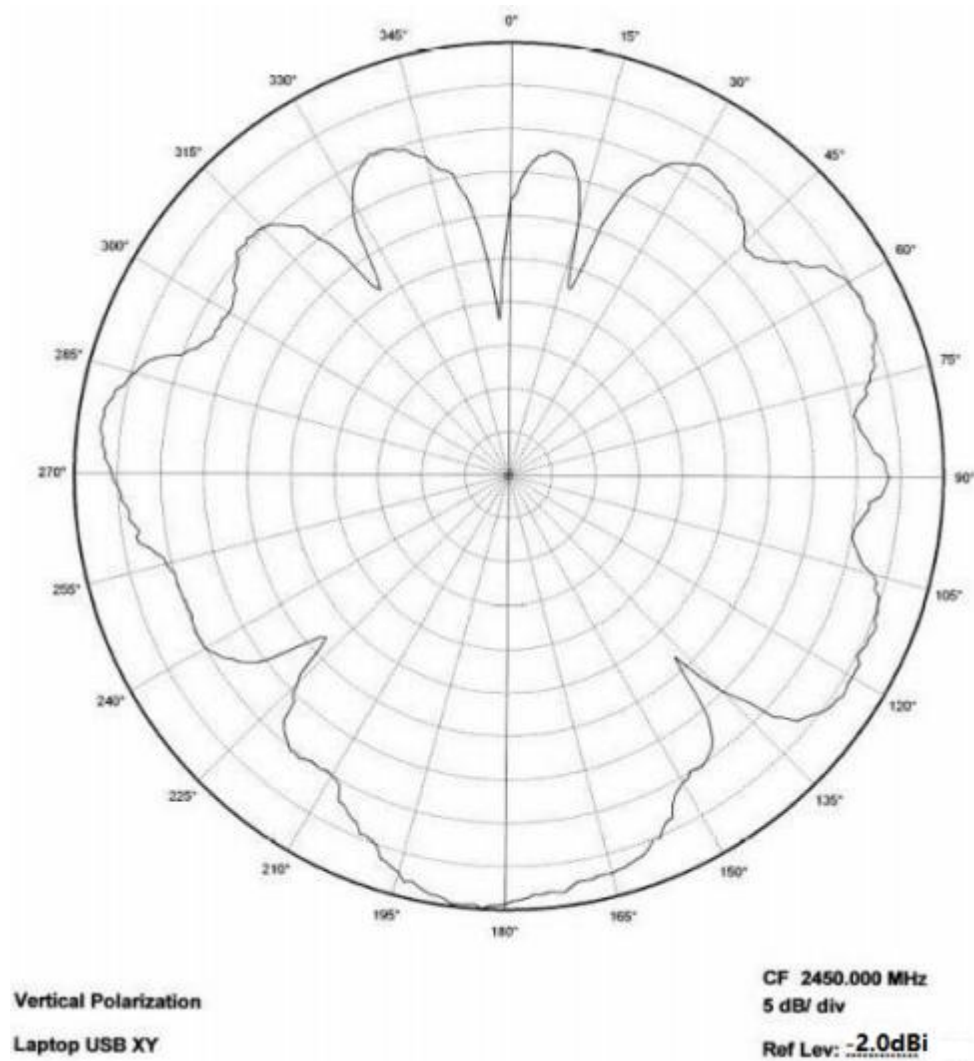
Figure 13: WLT5283M in Laptop XY Plane
