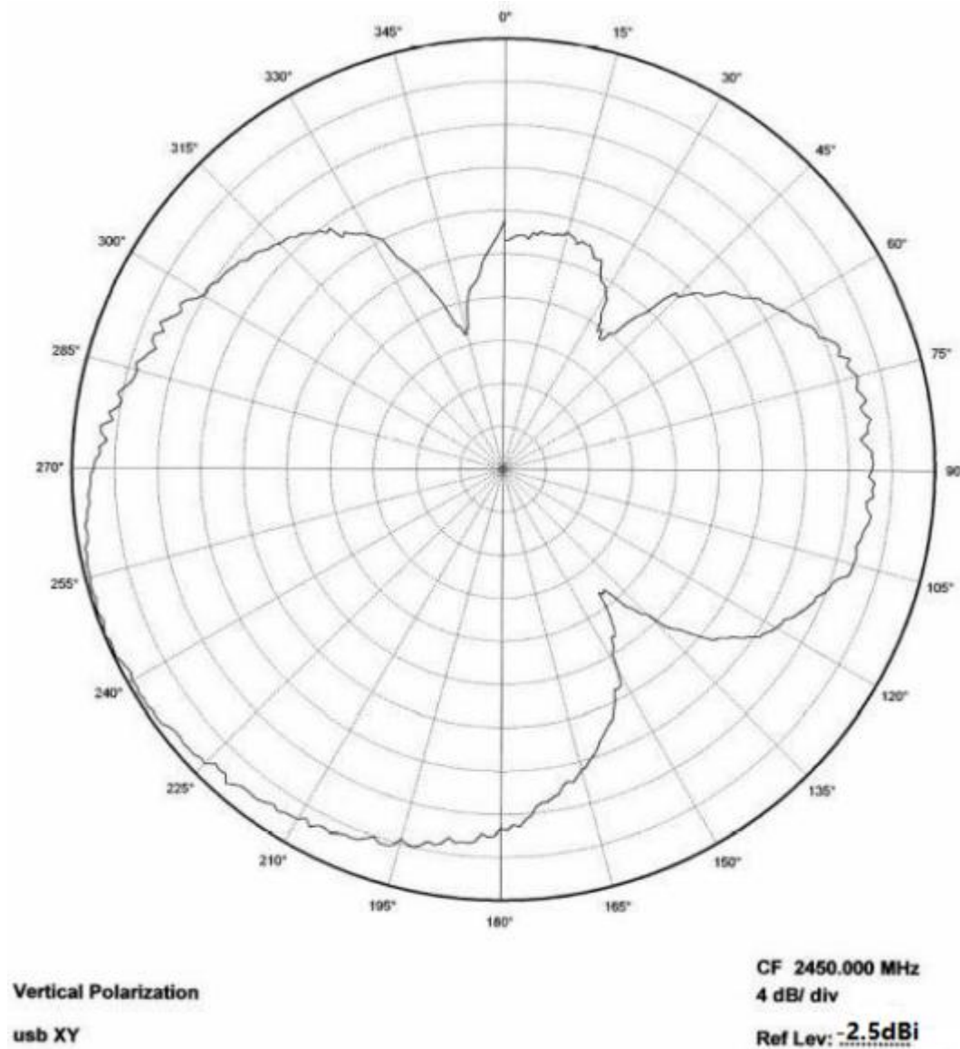
Figure 7: WLT5283M XY Plane
