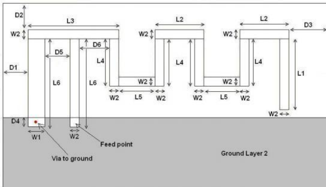
Figure 3: Antenna Dimensions
