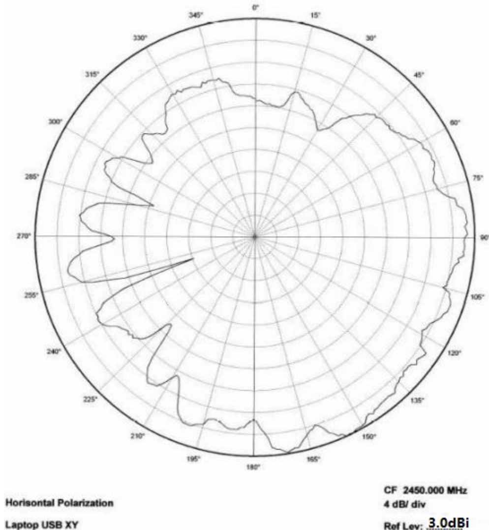
Figure 14: WLT5283M in Laptop XY Plane
