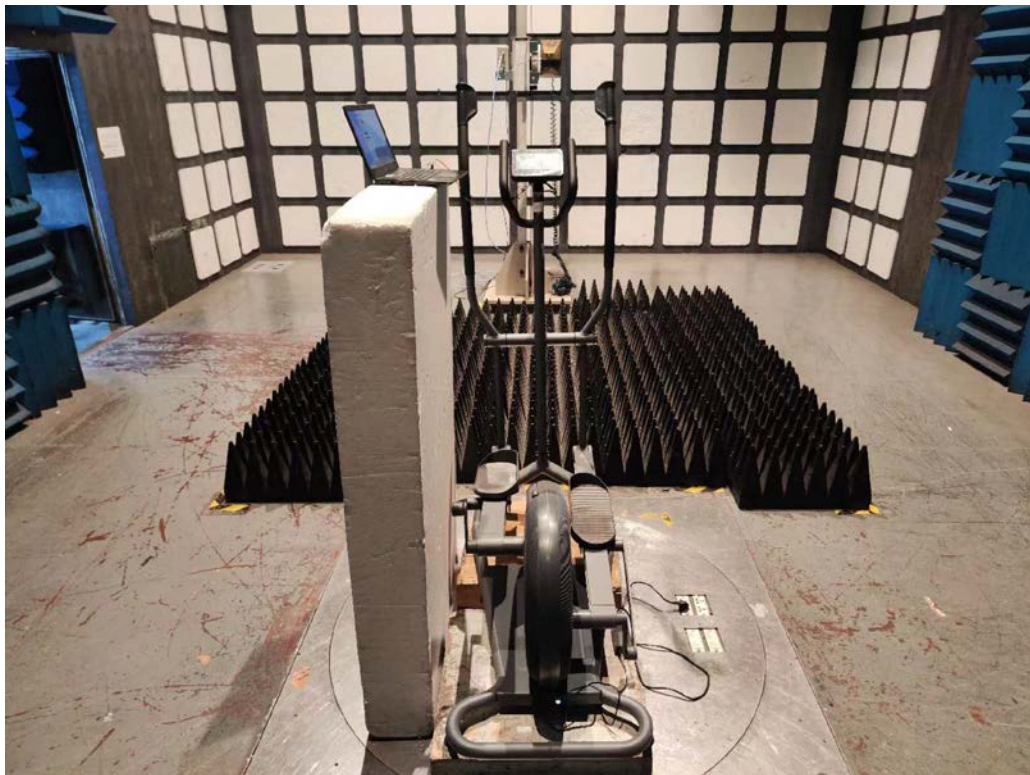
(ABOVE 1GHz) SIDE
