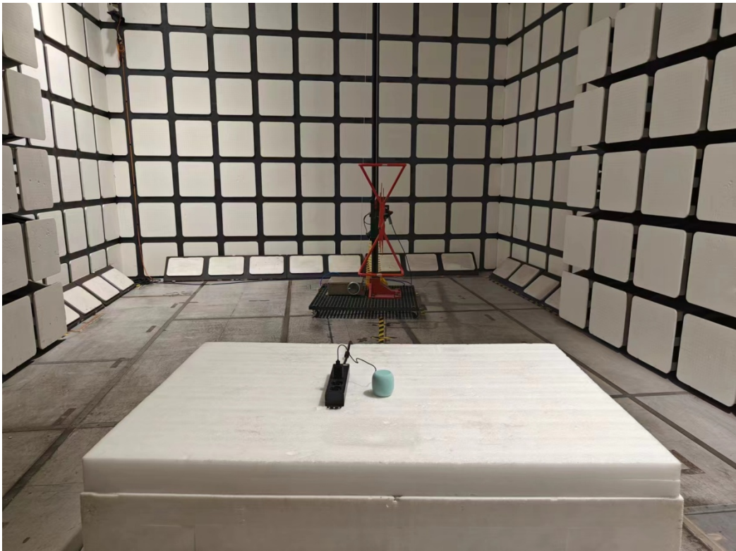
Radiated Emissions View (30MHz-1000MHz)
