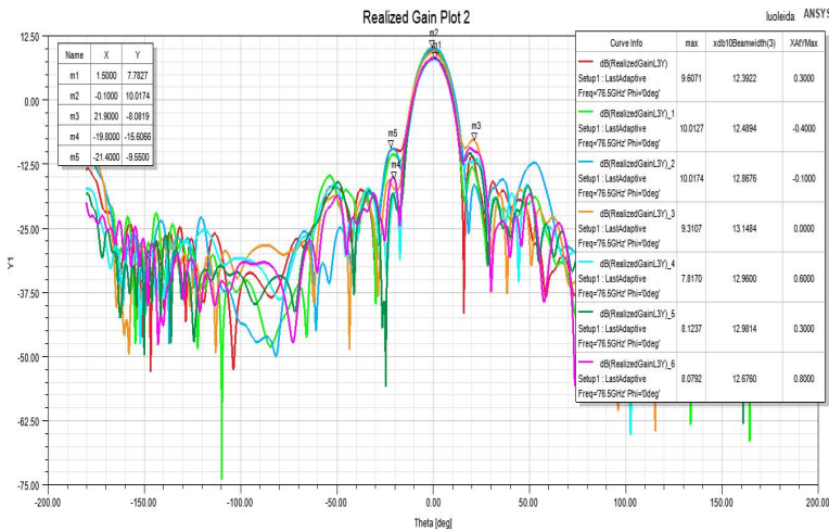
Antenna elevation pattern
