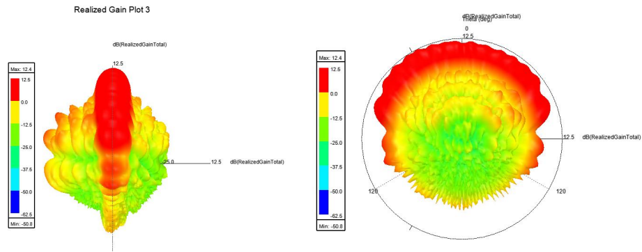
Antenna 3D Radiation Pattern
