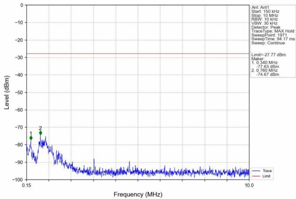
8DPSK_3DH5_LCH_2402MHz_Ant1_NTNV
