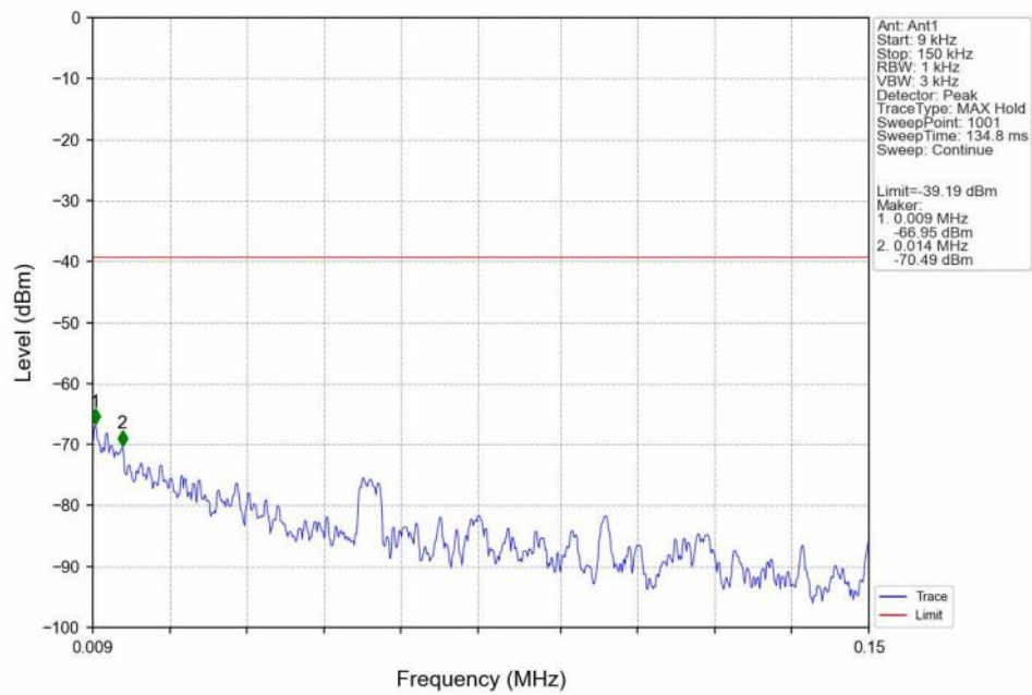
GFSK_DH5_HCH_2480MHz_Ant1_NTNV
