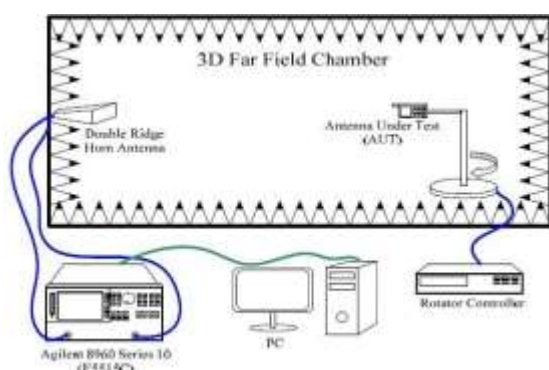
Fig.2 FAR-field Chamber
