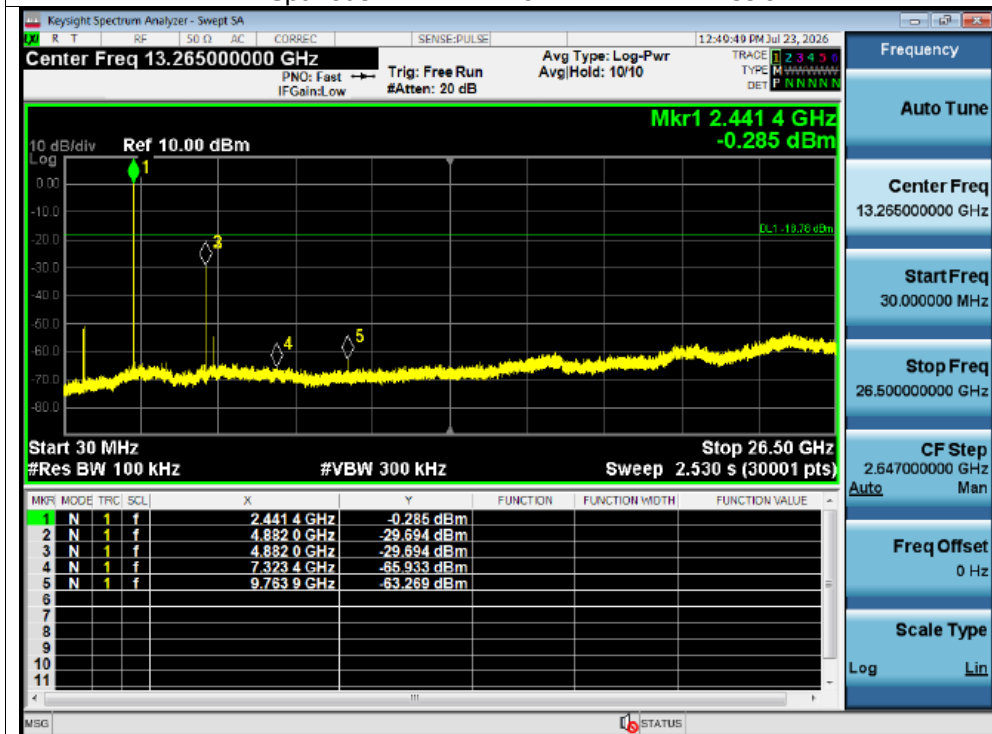
Tx. Spurious NVNT 2-DH5 2441MHz Emission
