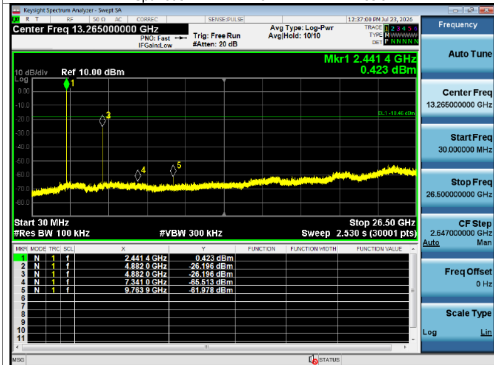
Tx. Spurious NVNT 1-DH5 2441MHz Emission
