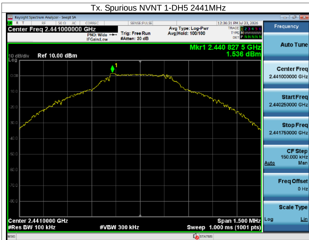
Tx. Spurious NVNT 1-DH5 2441MHz Emission
