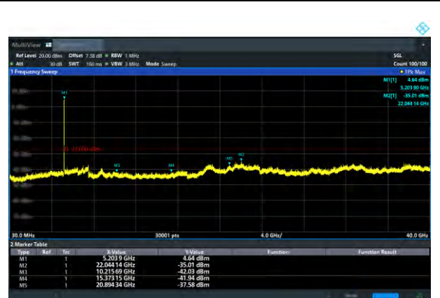
11ax (HT40) CH38
