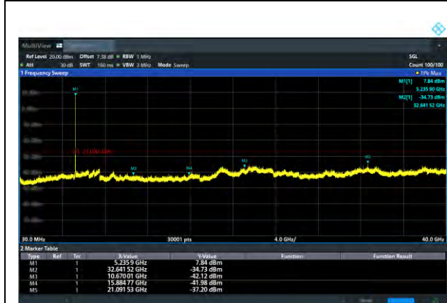
11ax (HT20) CH48
