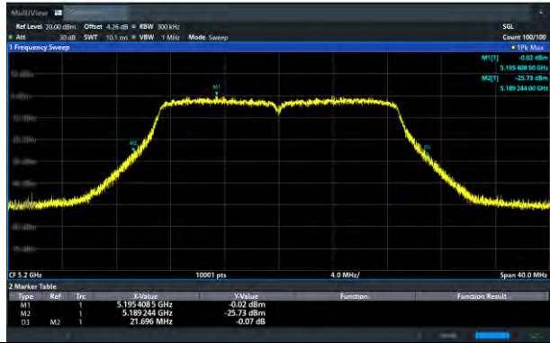
11n (HT20) CH40_26dB
