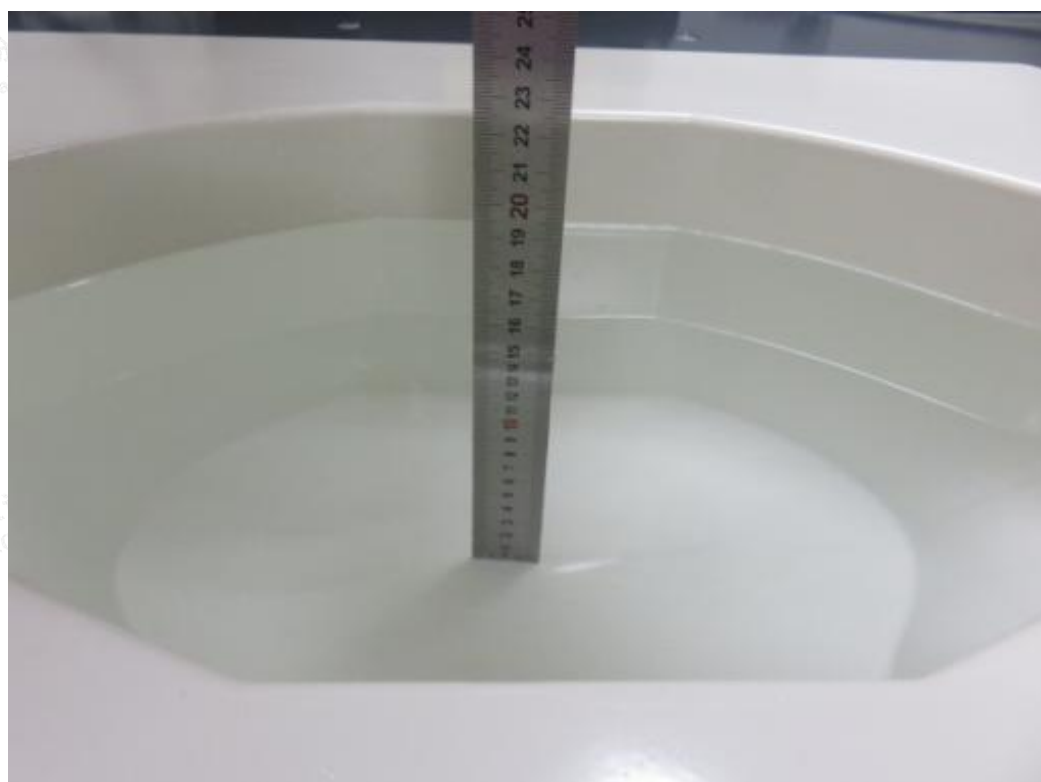
Photograph of the depth in the Body Phantom (5300MHz, 16.1cm depth)
