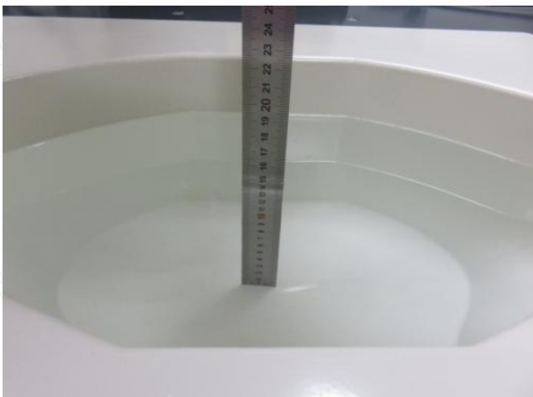
Photograph of the depth in the Body Phantom (5800MHz, 16.1cm depth)
