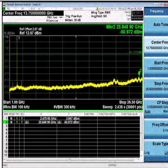
3DH5-Ant1-2480-1000~26500-PASS
