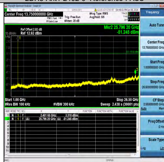
2DH5-Ant1-2402-1000~26500-PASS
