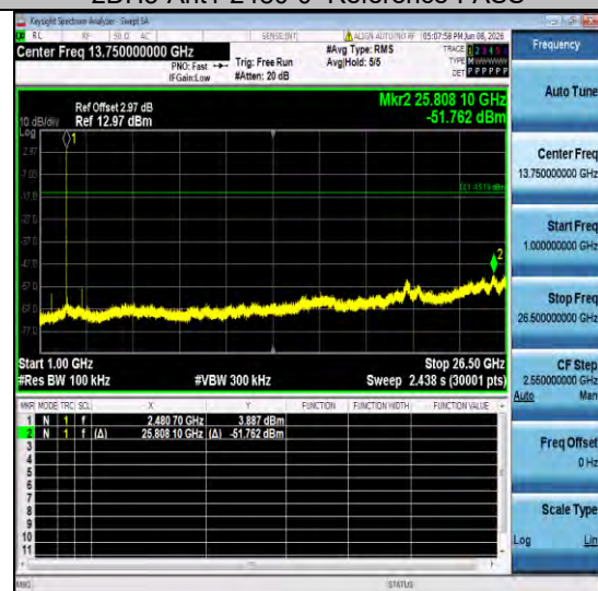
2DH5-Ant1-2480-1000~26500-PASS
