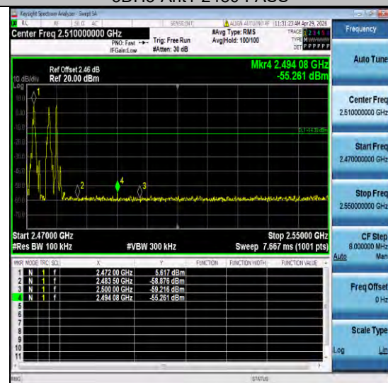
3D5-Ant1-Hop 2480-PASS
