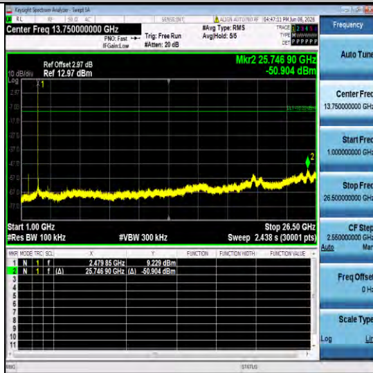
DH5-Ant1-2480-1000~26500-PASS
