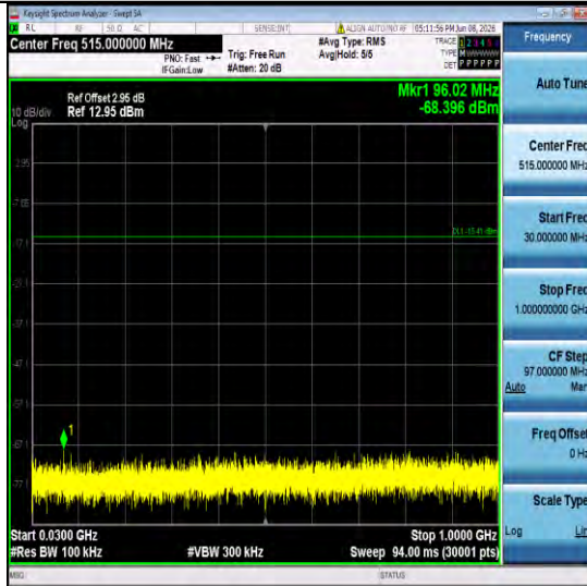
3DH5-Ant1-2441-30~1000-PASS
