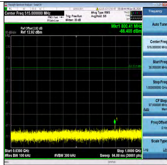
3DH5-Ant1-2402-30~1000-PASS
