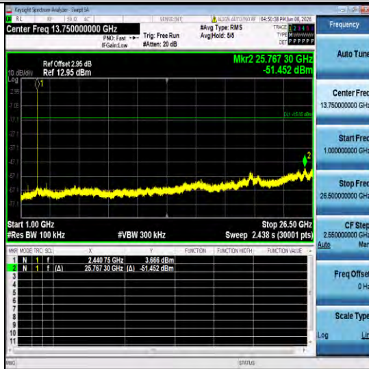
2DH5-Ant1-2441-1000~26500-PASS
