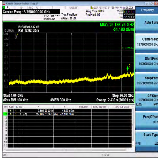
3DH5-Ant1-2402-1000~26500-PASS
