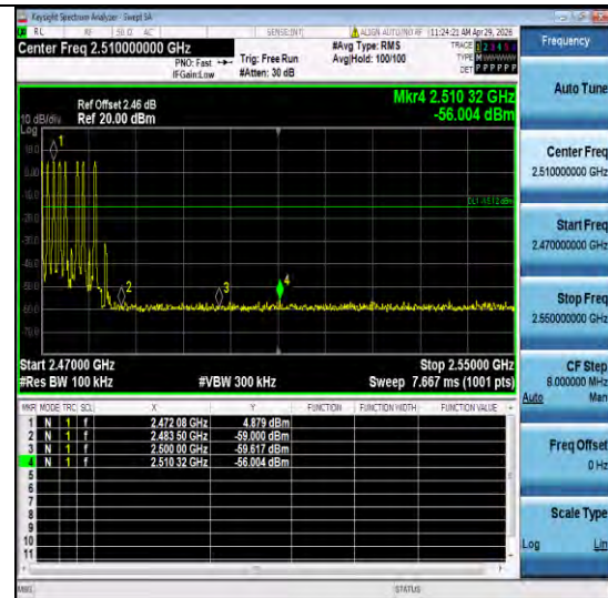
2D5-Hop 2480-PASS
