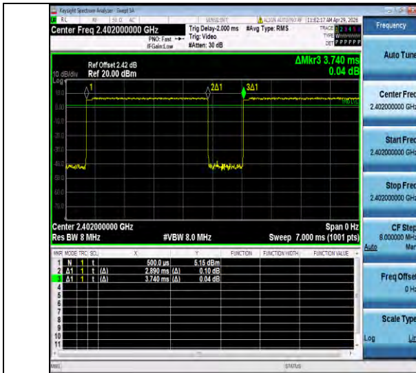
NTNV-3DH5-Ant1-2402
