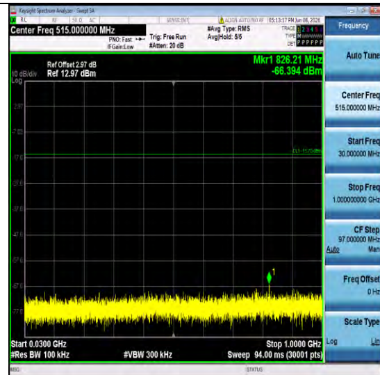
3DH5-Ant1-2480-30~1000-PASS
