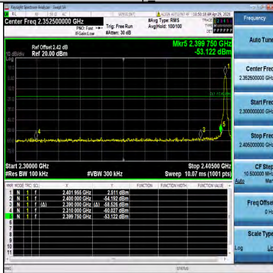
3D5-Ant1-2402-PASS
