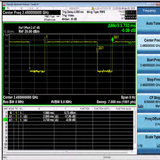
NTNV-3DH5-Ant1-2480
