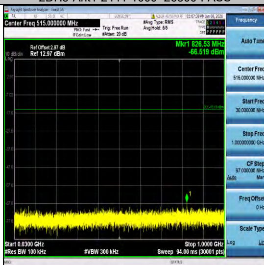
2DH5-Ant1-2480-30~1000-PASS
