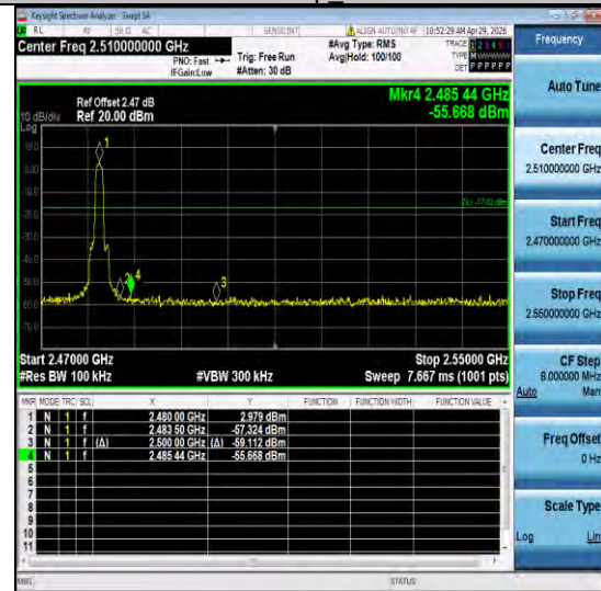
3D5-Ant1-2480-PASS
