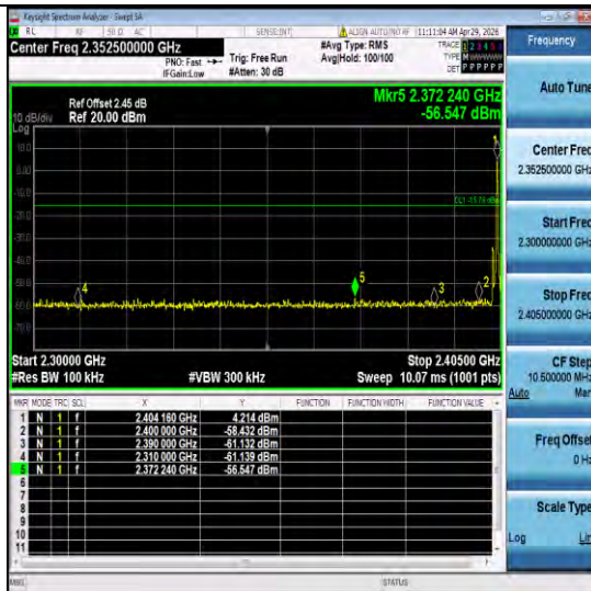
2D5-Hop 2402-PASS
