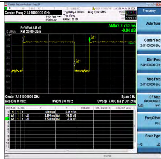
NTNV-3DH5-Ant1-2441
