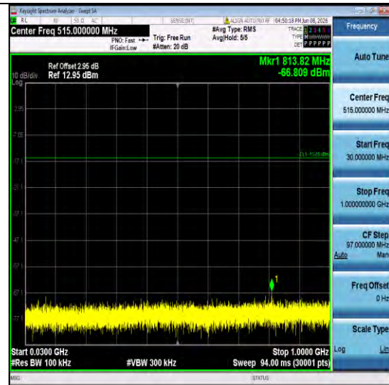
2DH5-Ant1-2441-30~1000-PASS
