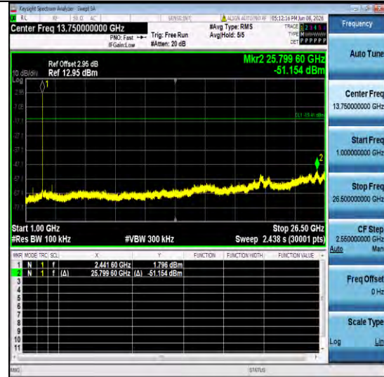
3DH5-Ant1-2441-1000~26500-PASS
