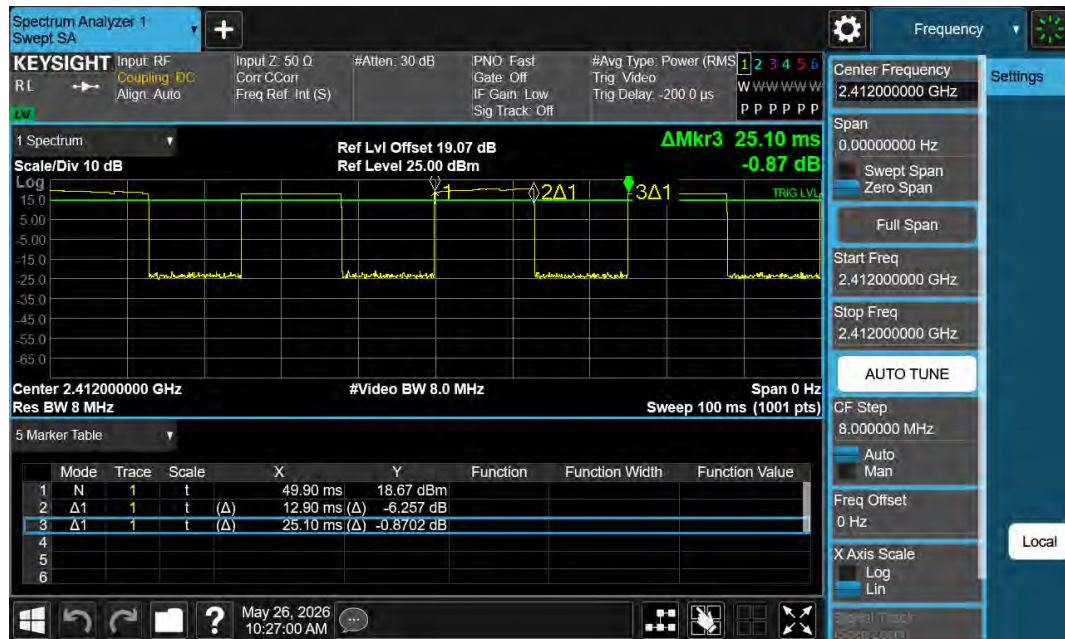
NTNV-11B-Ant2-2412
