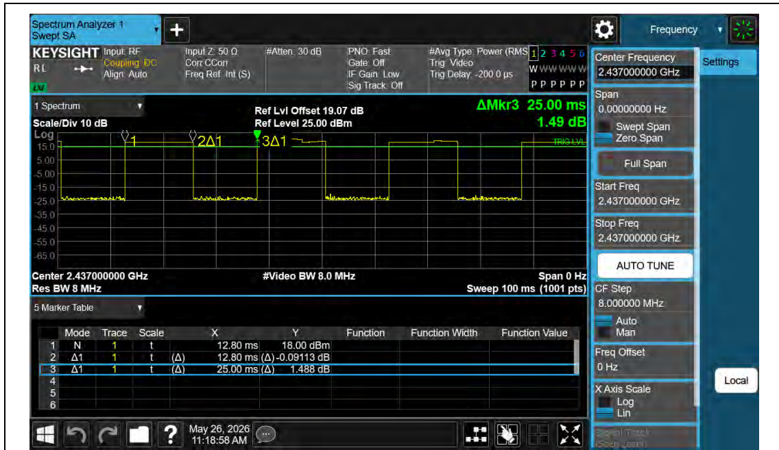
NTNV-11B-Ant2-2437
