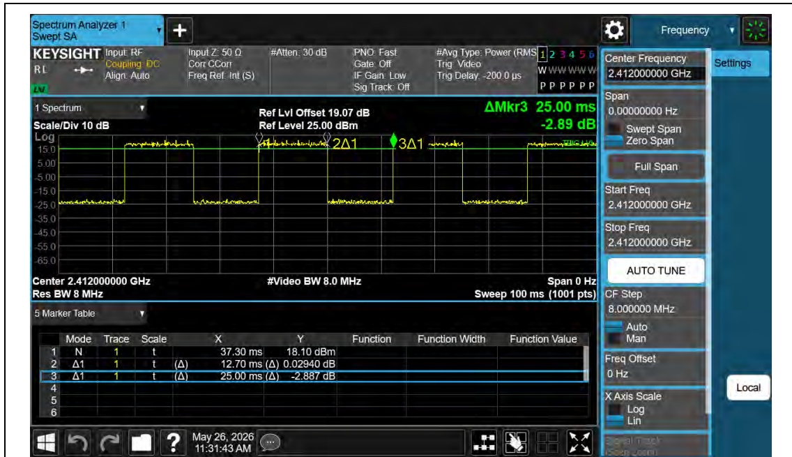
NTNV-11G-Ant2-2412
