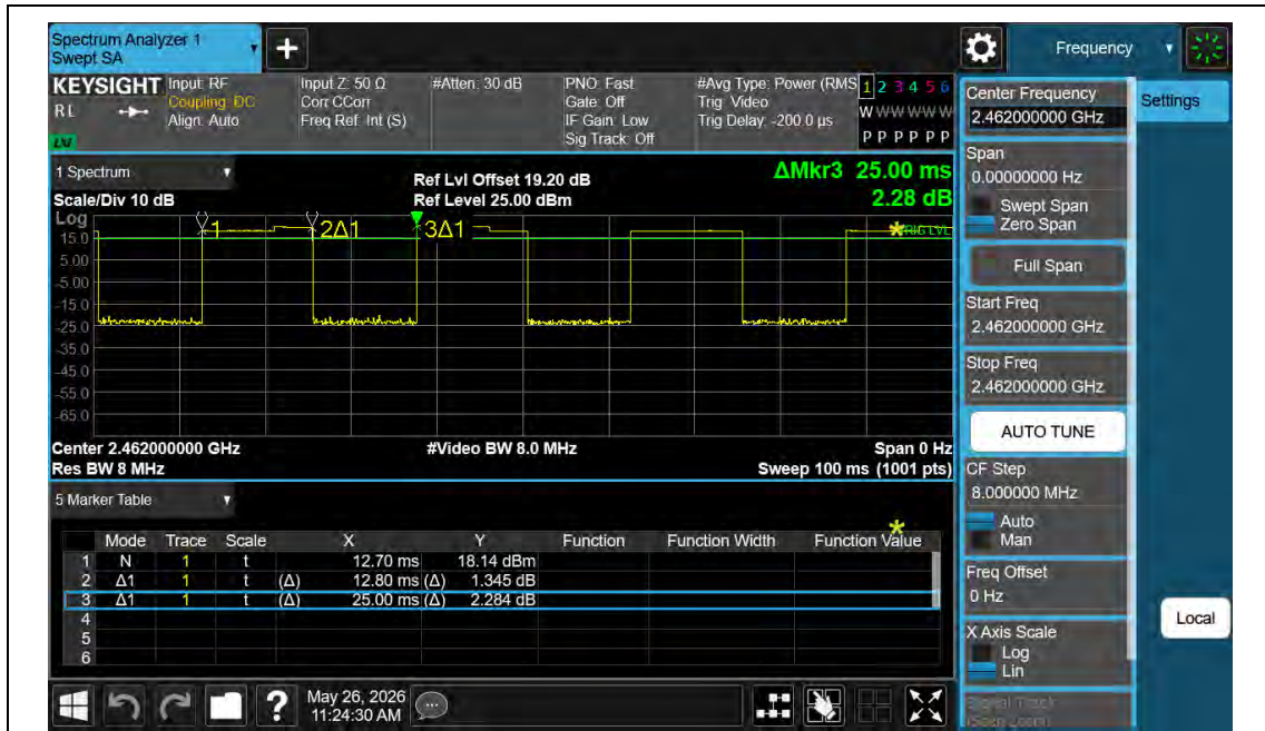
NTNV-11B-Ant2-2462
