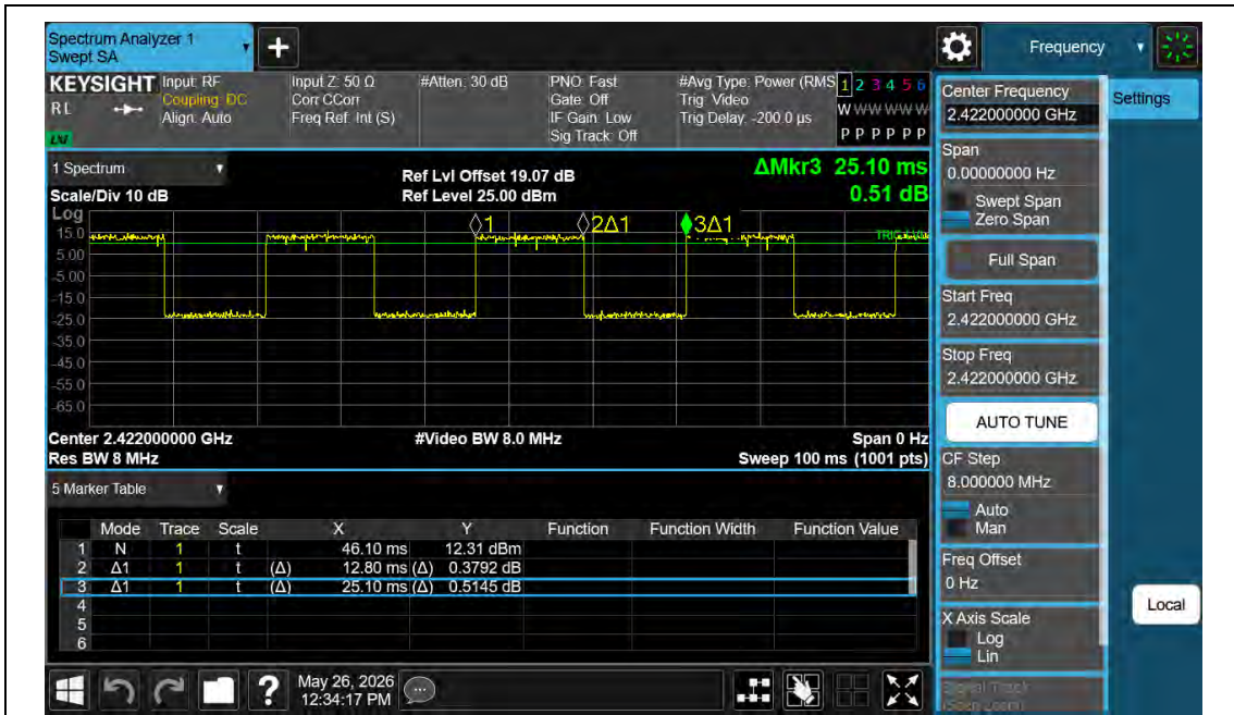
NTNV-11N40MIMO-Ant2-2422
