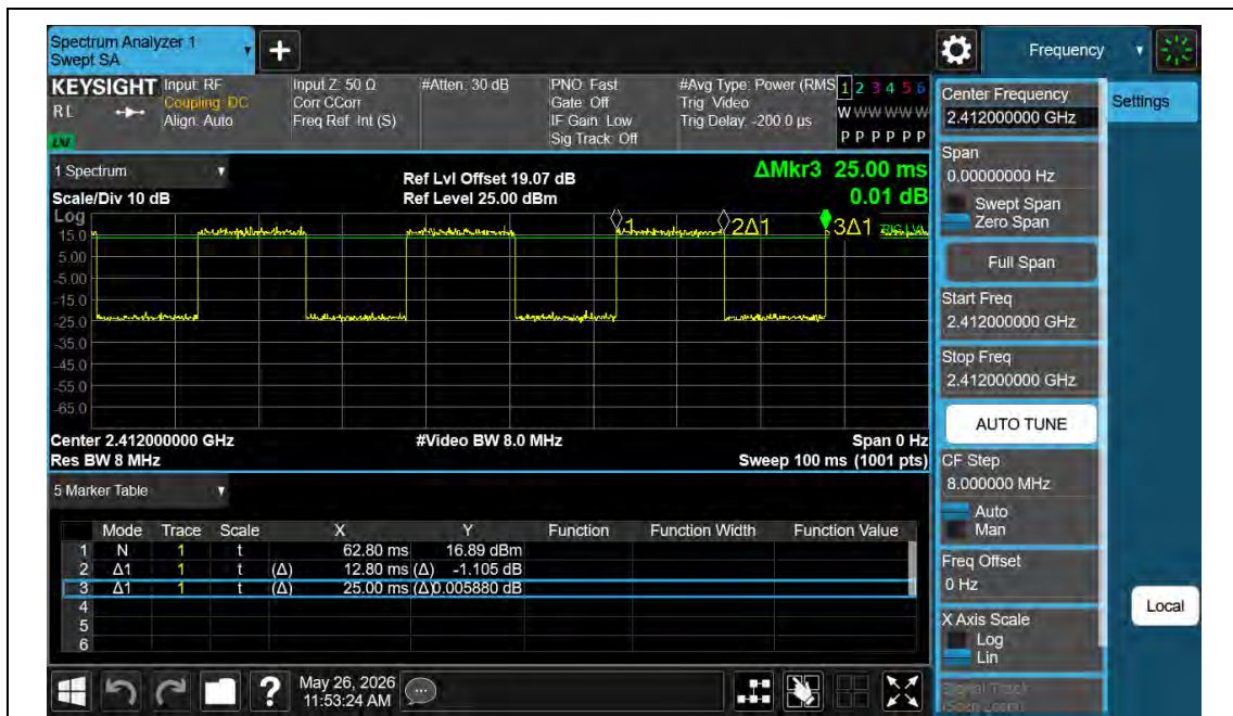
NTNV-11N20MIMO-Ant2-2412
