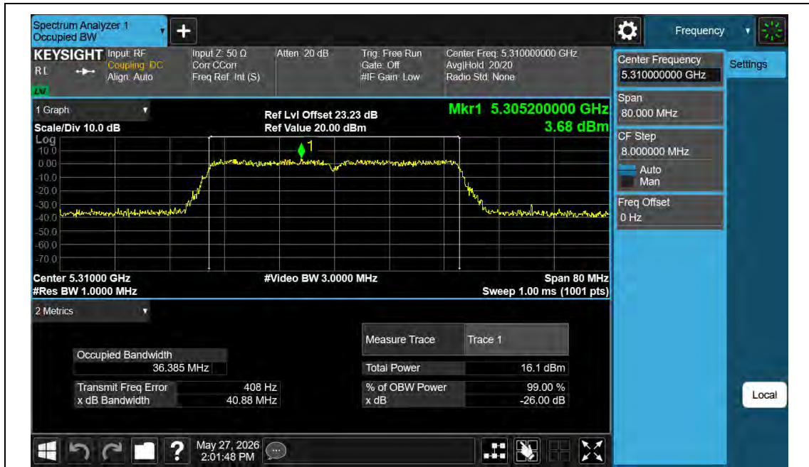
11N40MIMO-Ant2-5310
