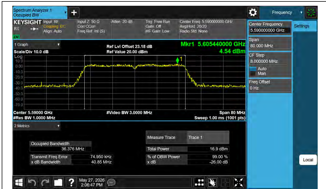
11N40MIMO-Ant2-5590
