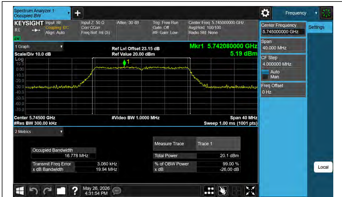
11A-Ant2-5745
