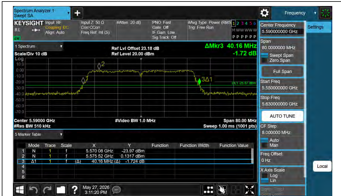
11AC40MIMO-Ant2-5590
