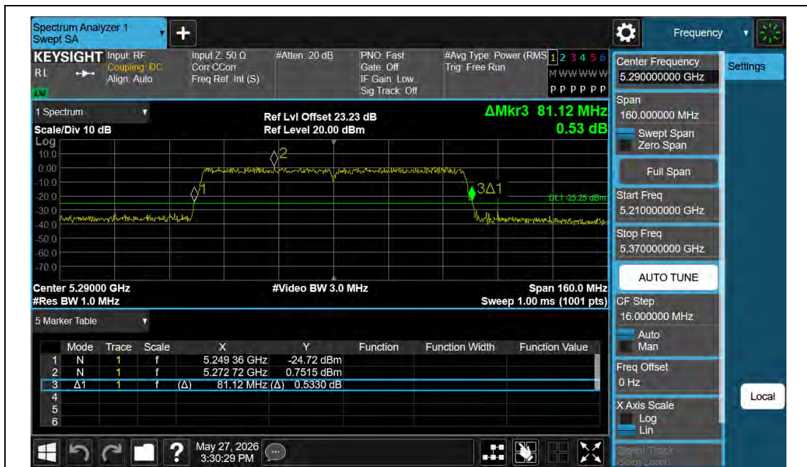
11AC80MIMO-Ant2-5290
