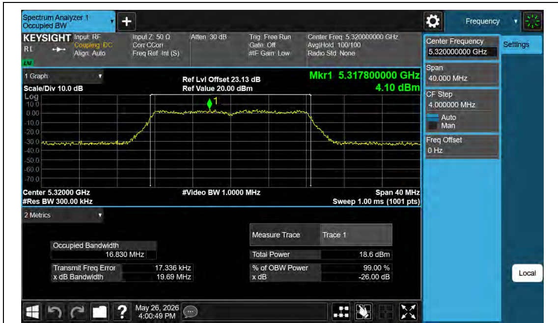
11A-Ant2-5320
