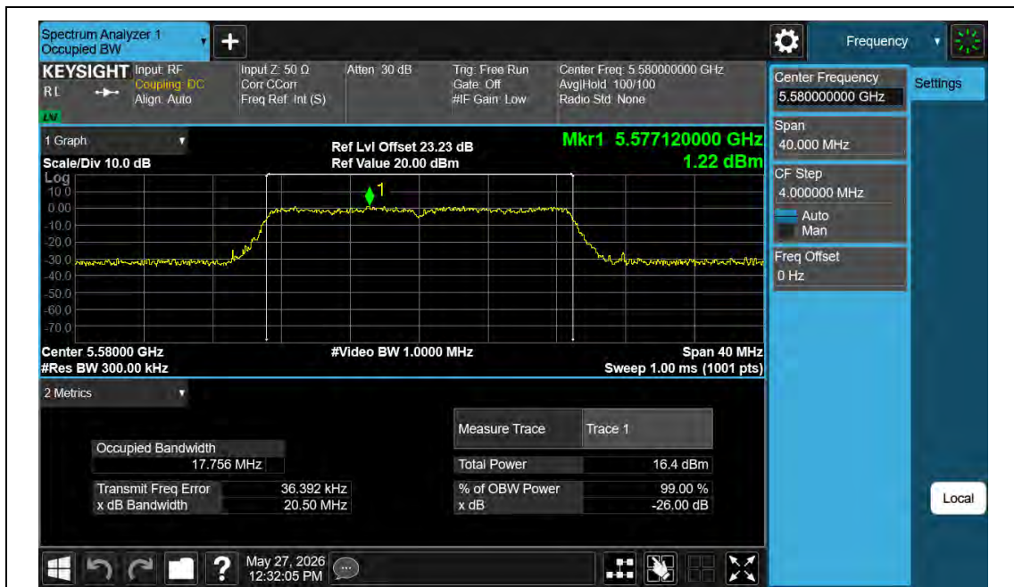
11N20MIMO-Ant2-5580
