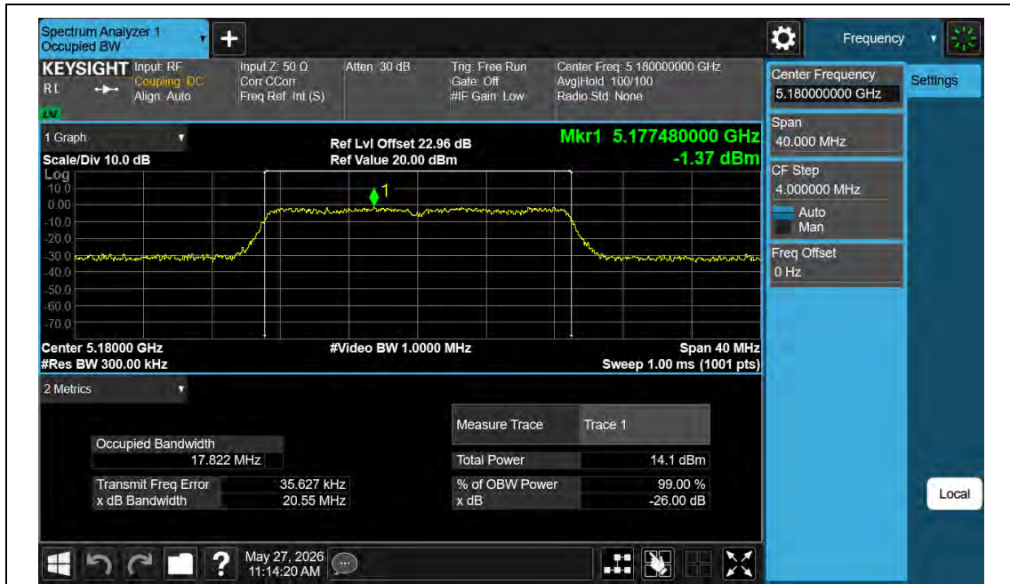
11N20MIMO-Ant2-5180
