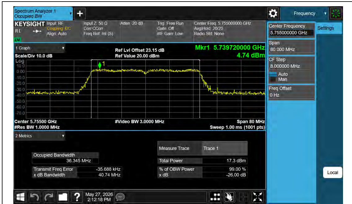
11N40MIMO-Ant2-5755
