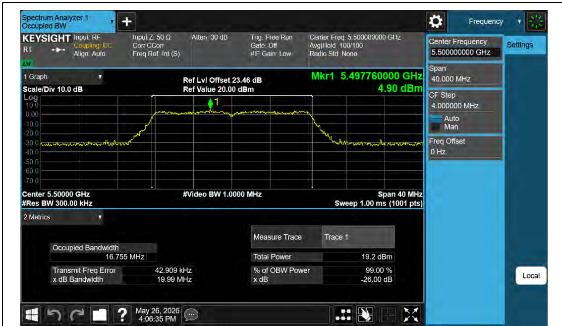
11A-Ant2-5500
