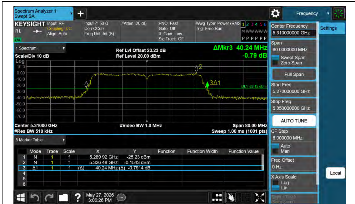
11AC40MIMO-Ant2-5310
