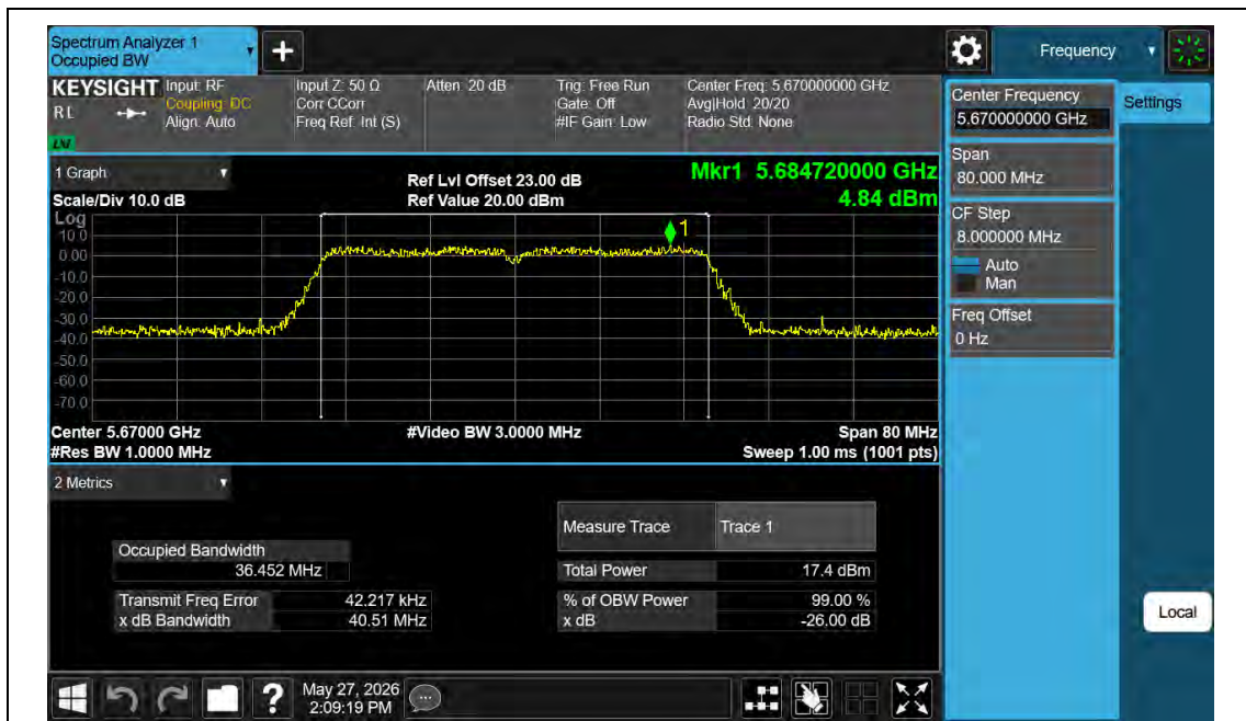
11N40MIMO-Ant2-5670
