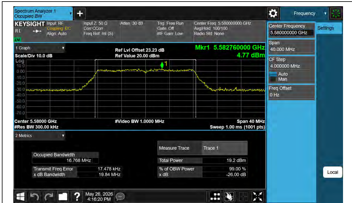
11A-Ant2-5580
