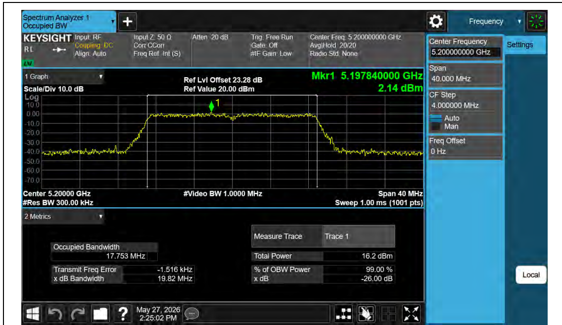
11AC20MIMO-Ant2-5200
