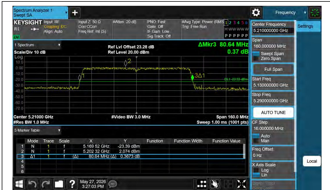
11AC80MIMO-Ant2-5210
