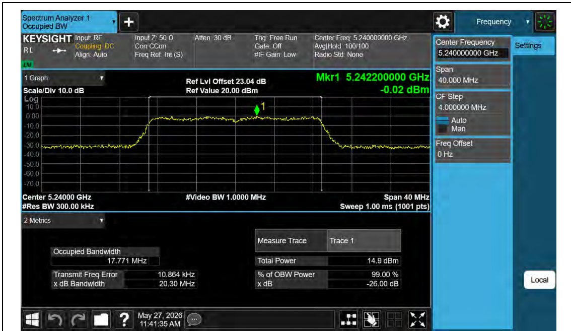
11N20MIMO-Ant2-5240
