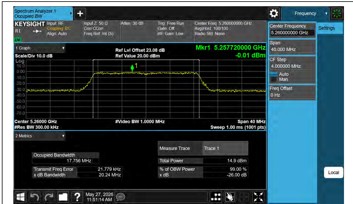
11N20MIMO-Ant2-5260
