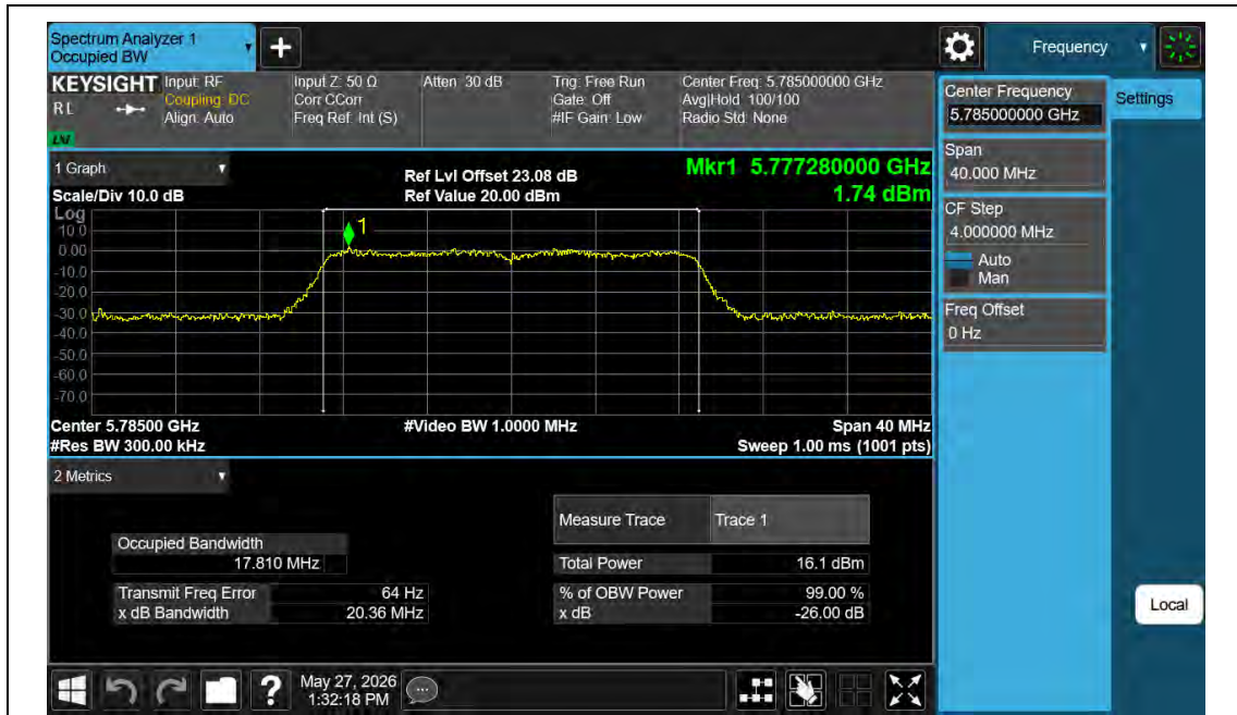
11N20MIMO-Ant2-5785
