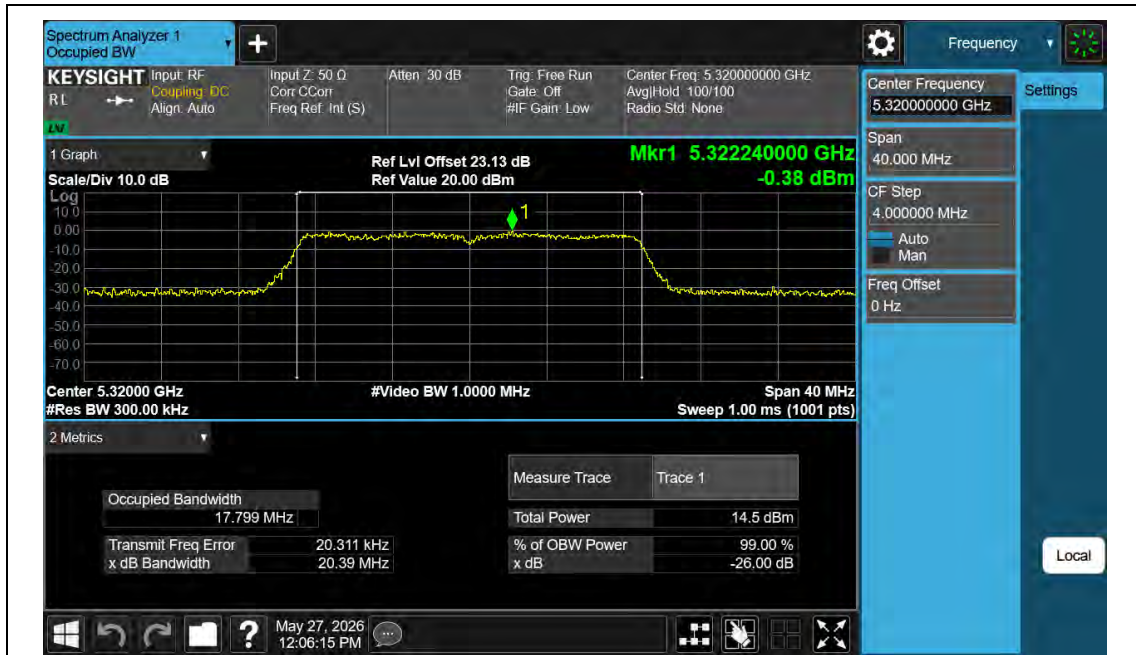
11N20MIMO-Ant2-5320
