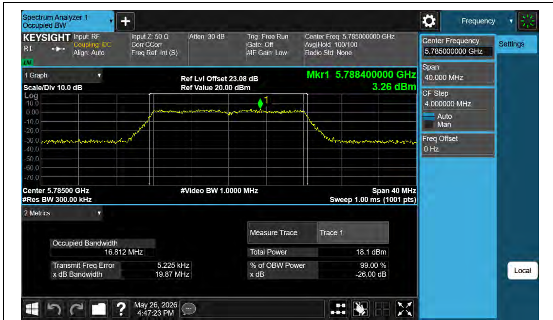
11A-Ant2-5785
