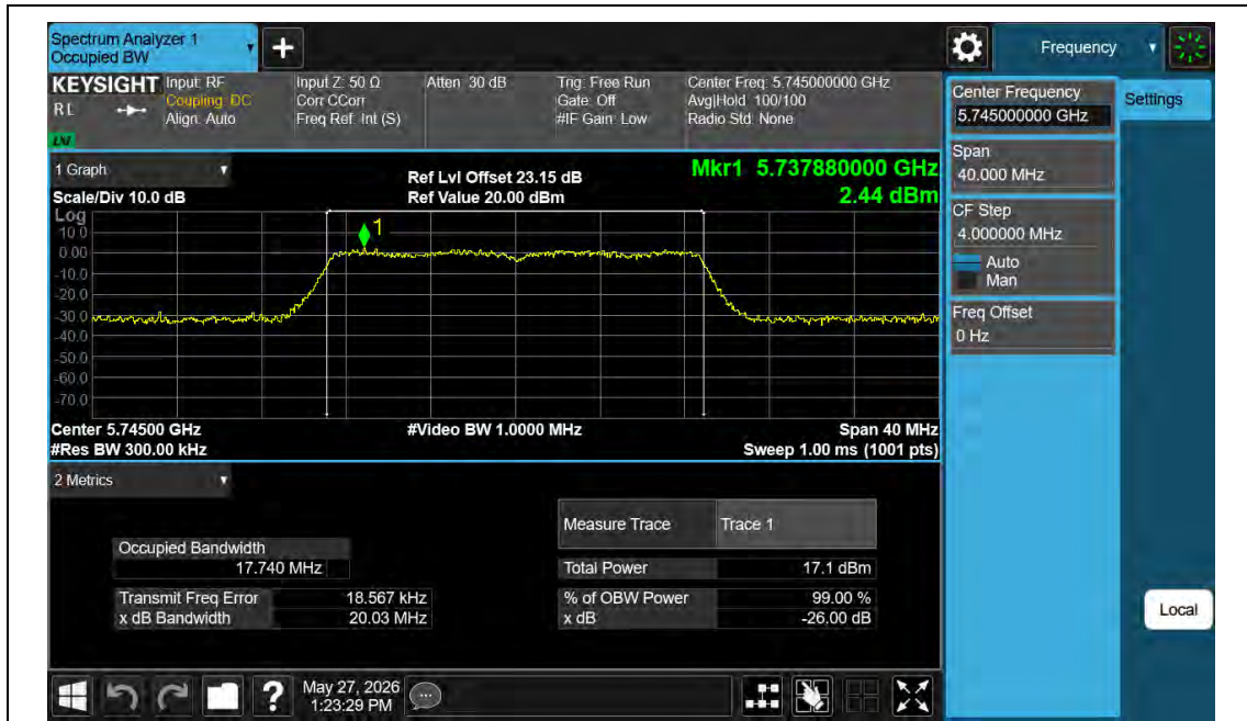
11N20MIMO-Ant2-5745
