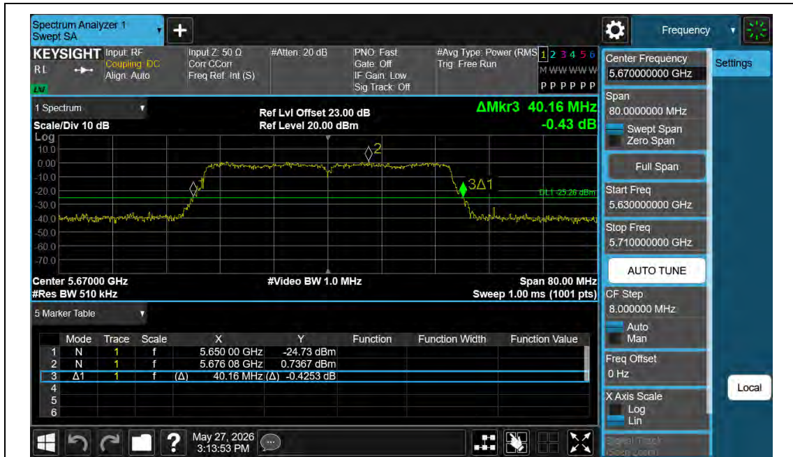
11AC40MIMO-Ant2-5670
