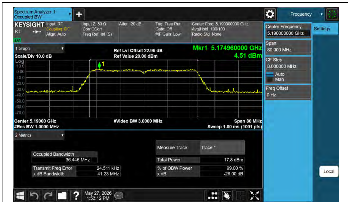
11N40MIMO-Ant2-5190
