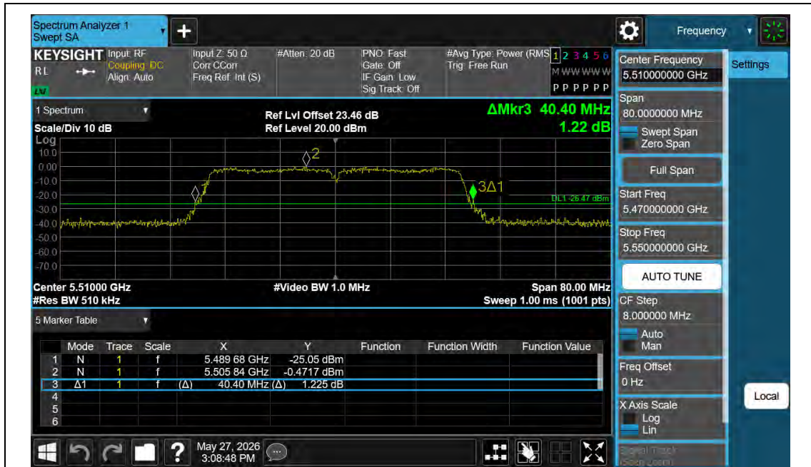
11AC40MIMO-Ant2-5510
