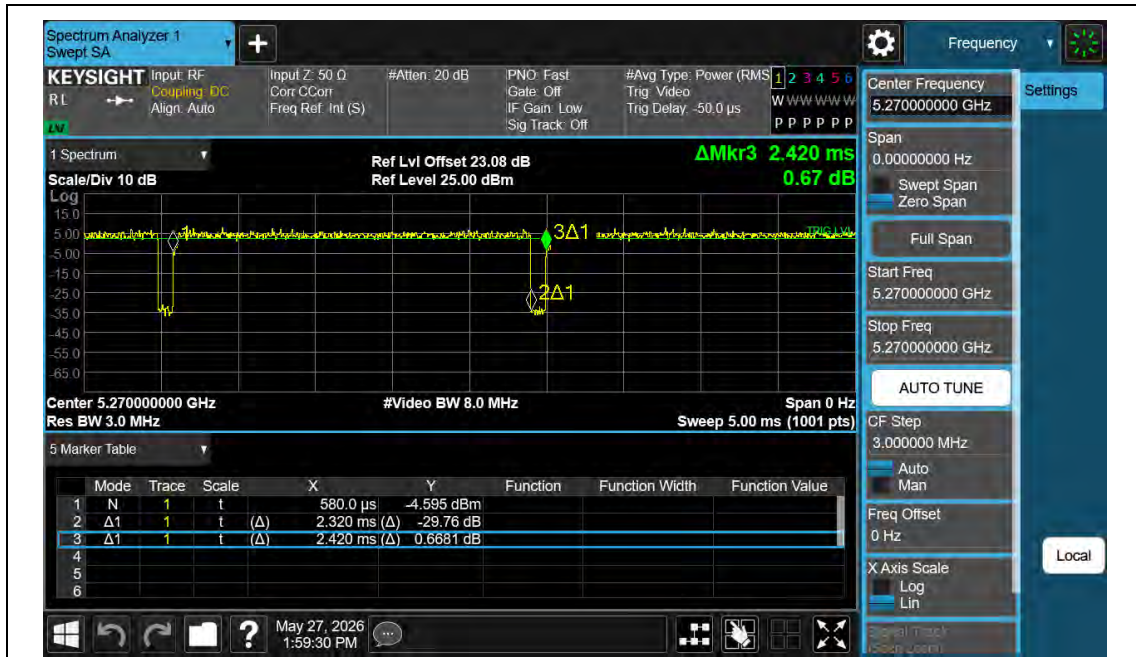
NTNV-11N40MIMO-Ant2-5270
