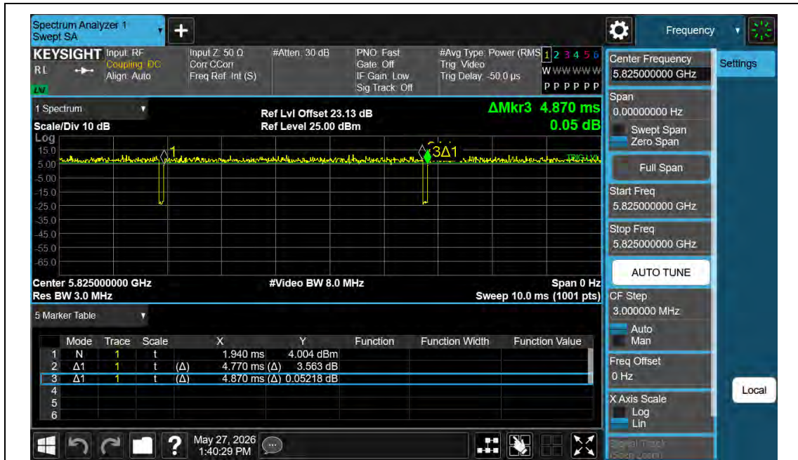
NTNV-11N20MIMO-Ant2-5825
