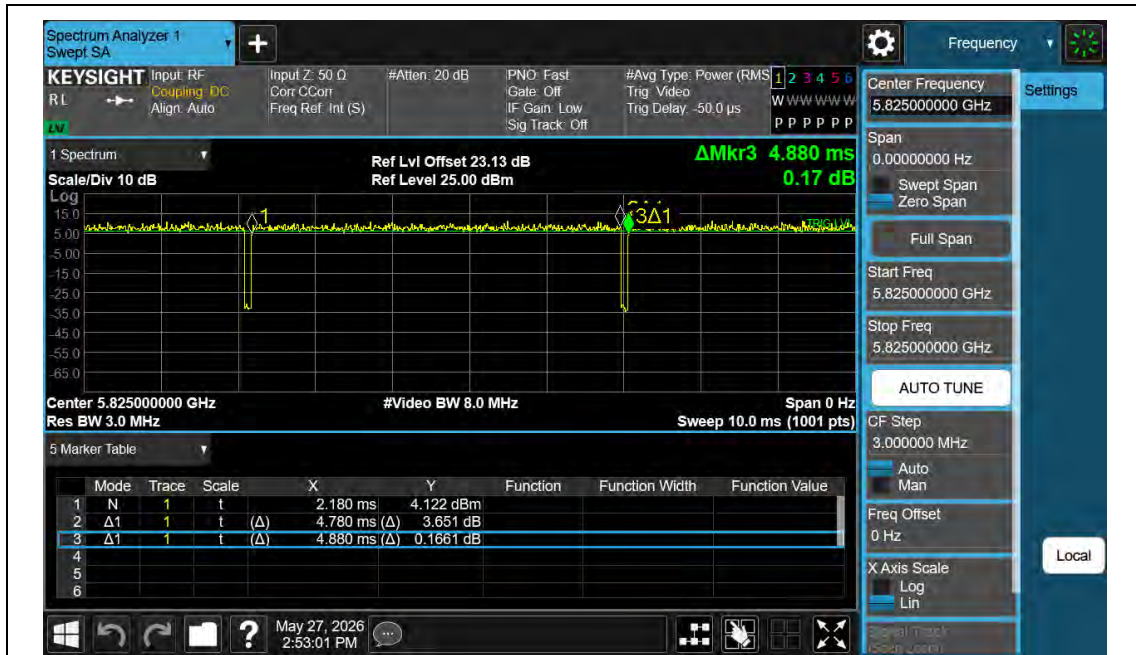
NTNV-11AC20MIMO-Ant2-5825
