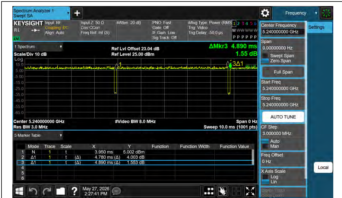
NTNV-11AC20MIMO-Ant2-5240
