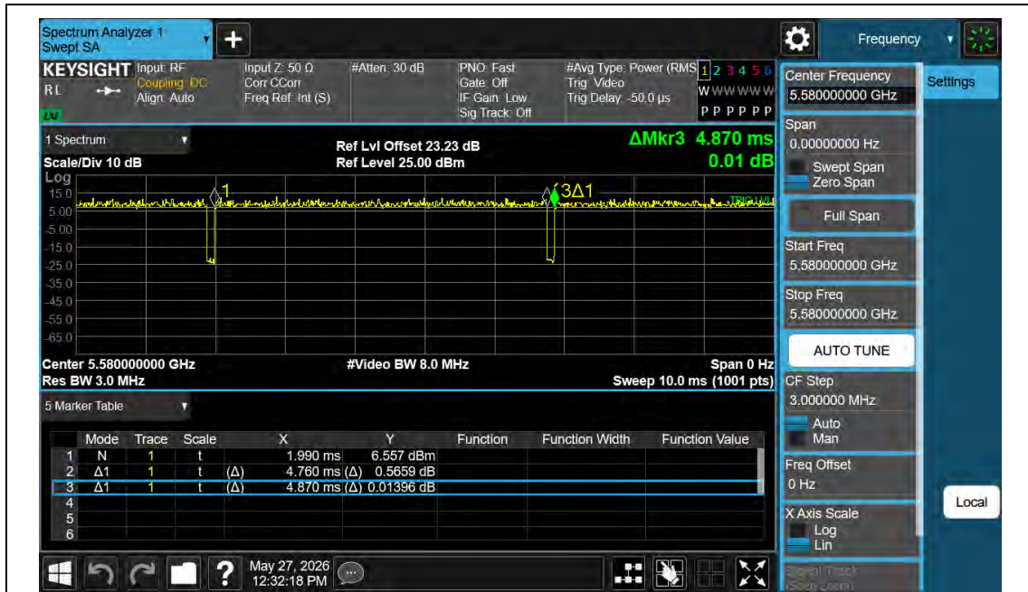
NTNV-11N20MIMO-Ant2-5580
