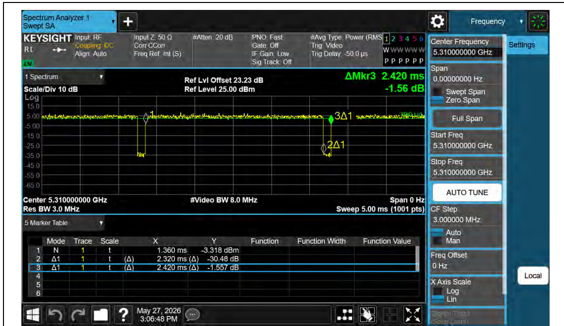
NTNV-11AC40MIMO-Ant2-5310
