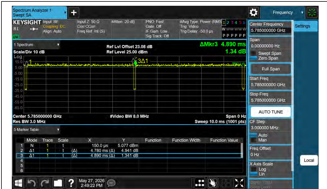
NTNV-11AC20MIMO-Ant2-5785
