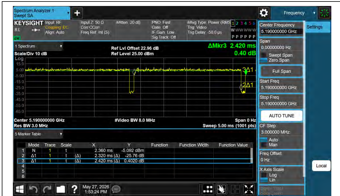
NTNV-11N40MIMO-Ant2-5190
