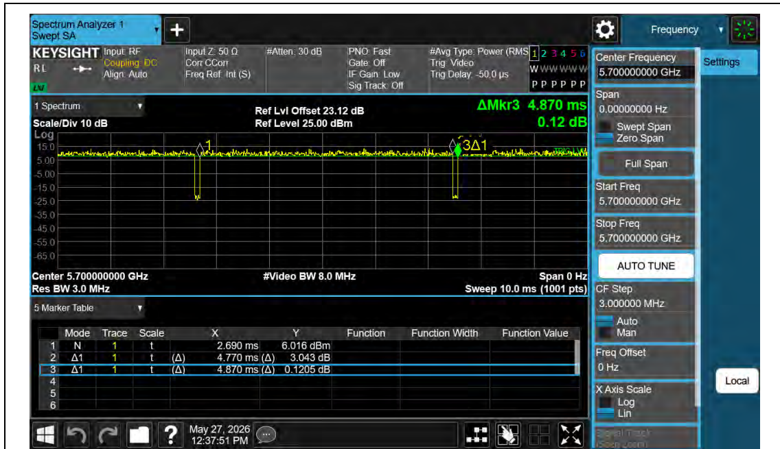
NTNV-11N20MIMO-Ant2-5700
