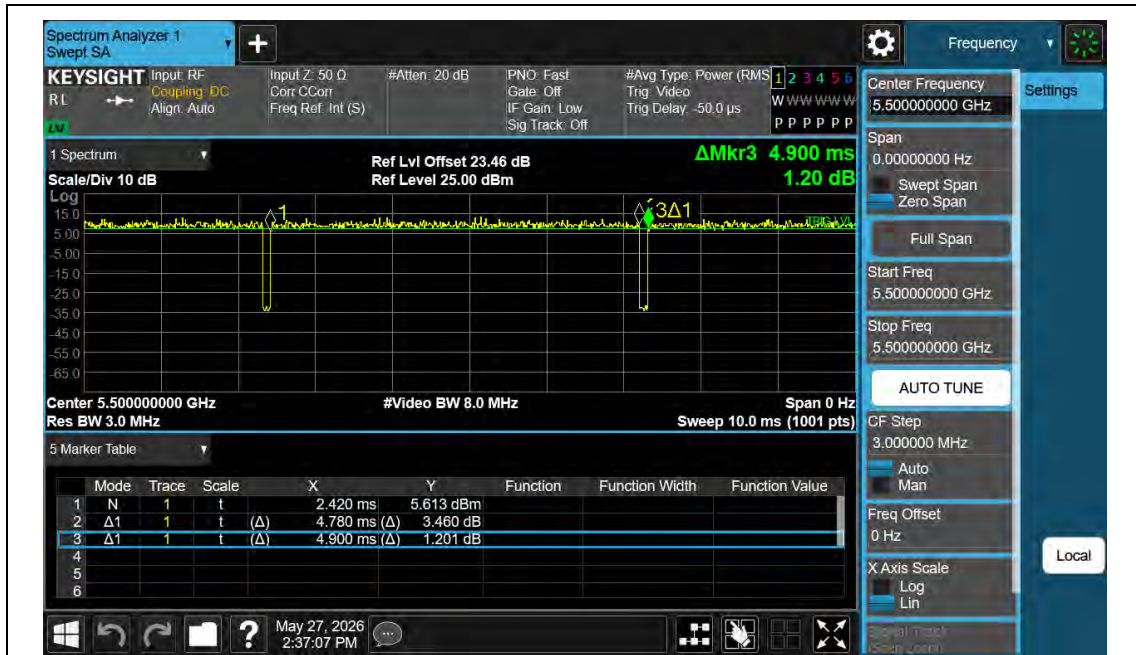
NTNV-11AC20MIMO-Ant2-5500
