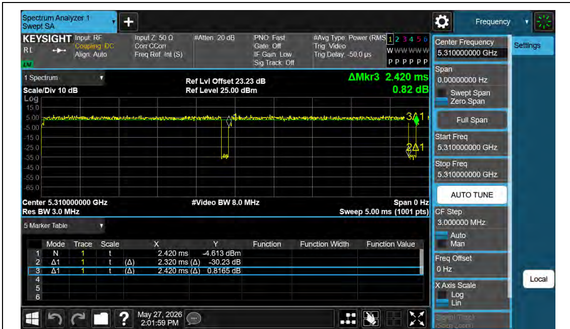
NTNV-11N40MIMO-Ant2-5310
