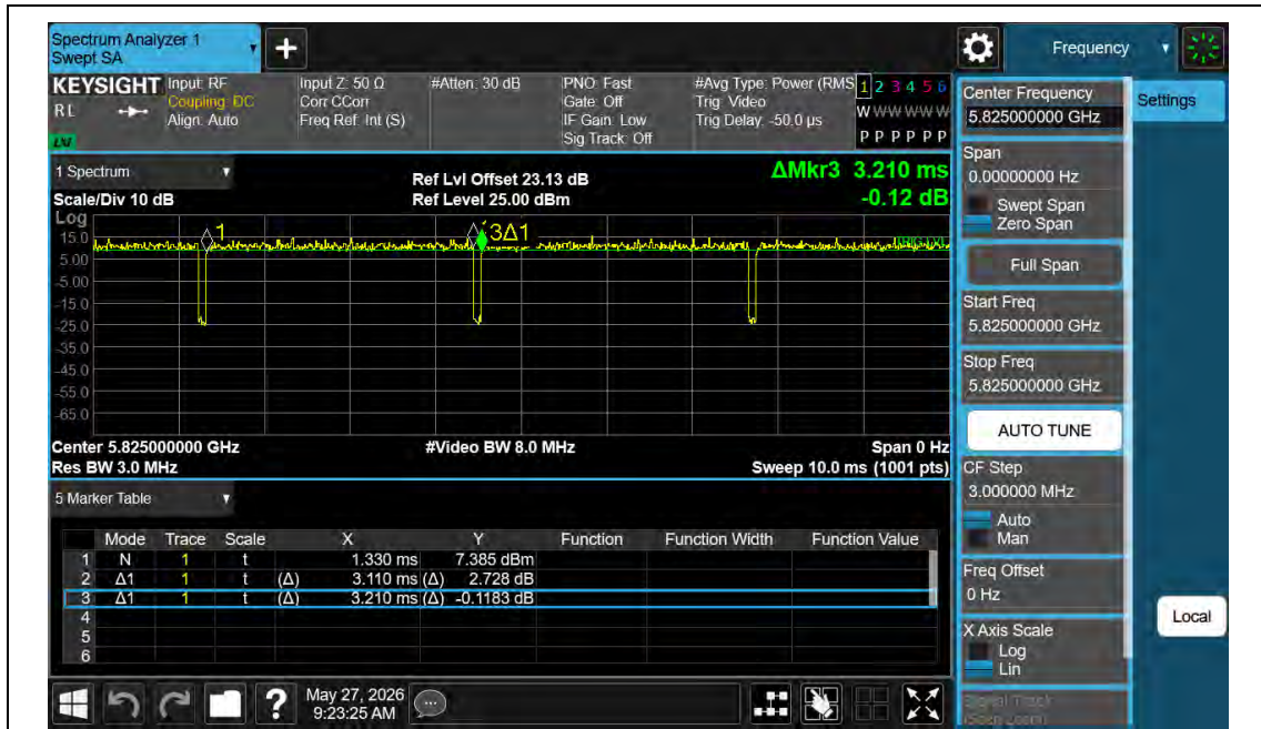
NTNV-11A-Ant2-5825
