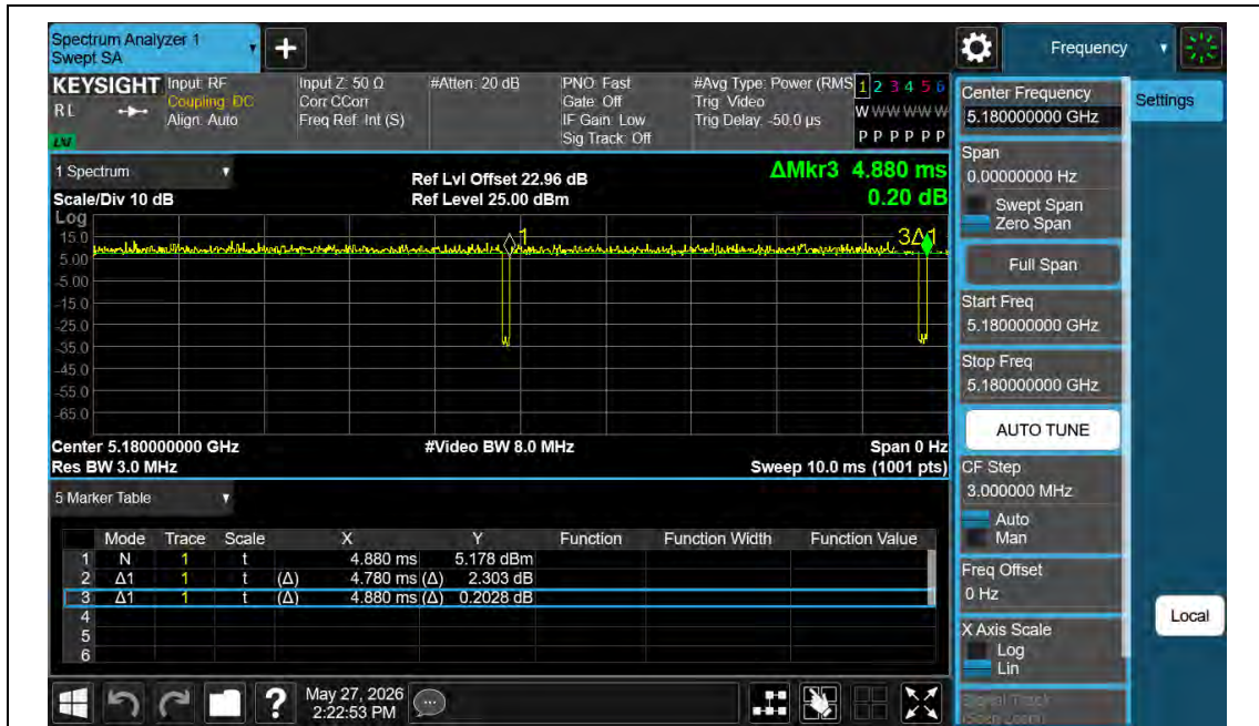
NTNV-11AC20MIMO-Ant2-5180
