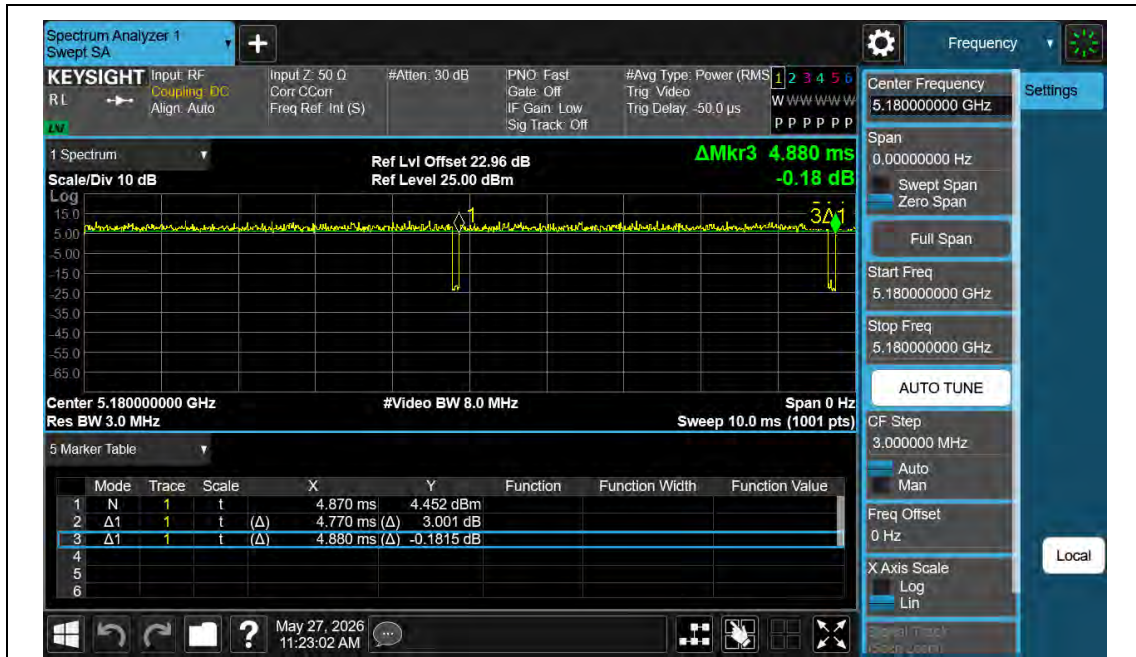
NTNV-11N20MIMO-Ant2-5180
