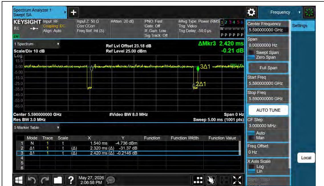
NTNV-11N40MIMO-Ant2-5590
