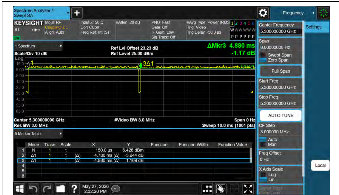
NTNV-11AC20MIMO-Ant2-5300
