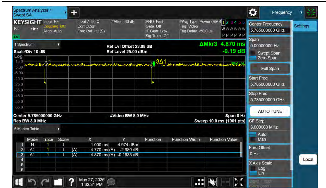
NTNV-11N20MIMO-Ant2-5785
