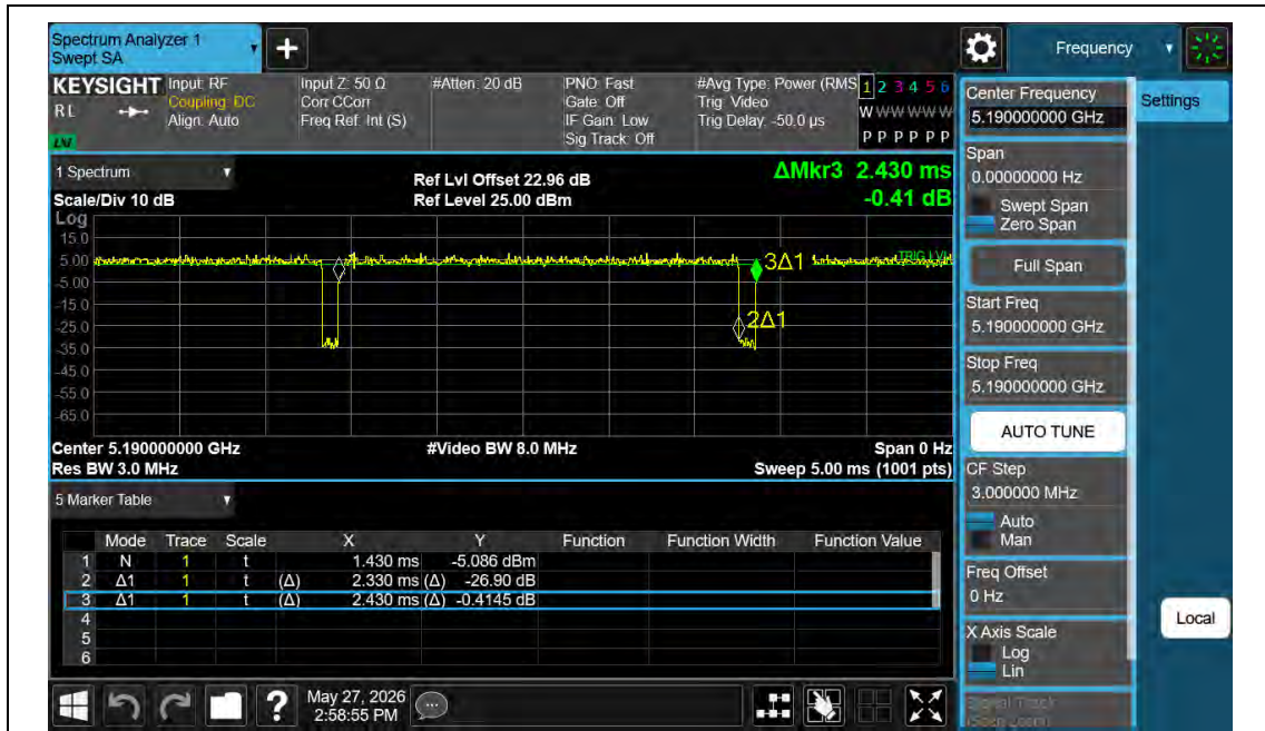
NTNV-11AC40MIMO-Ant2-5190
