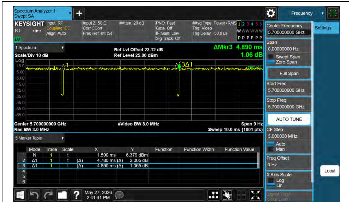
NTNV-11AC20MIMO-Ant2-5700
