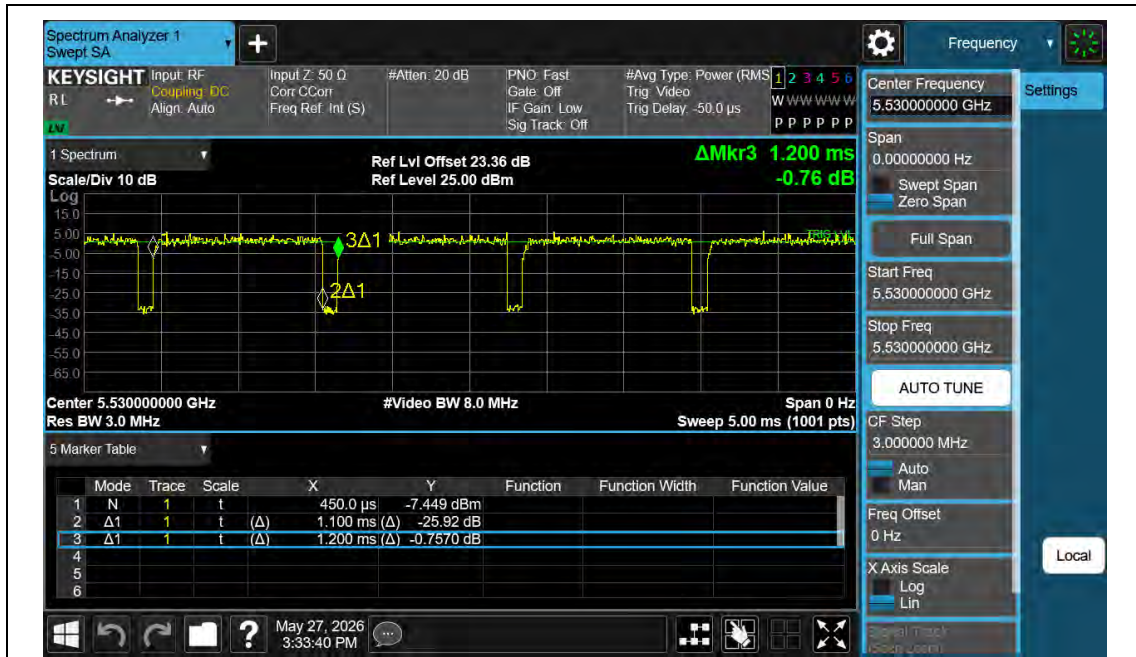
NTNV-11AC80MIMO-Ant2-5530
