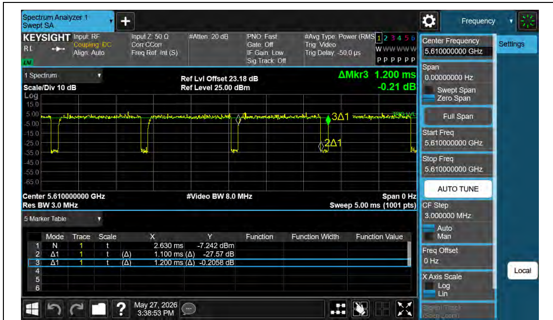
NTNV-11AC80MIMO-Ant2-5610
