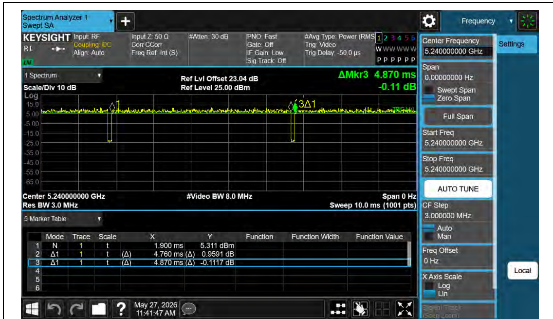
NTNV-11N20MIMO-Ant2-5240
