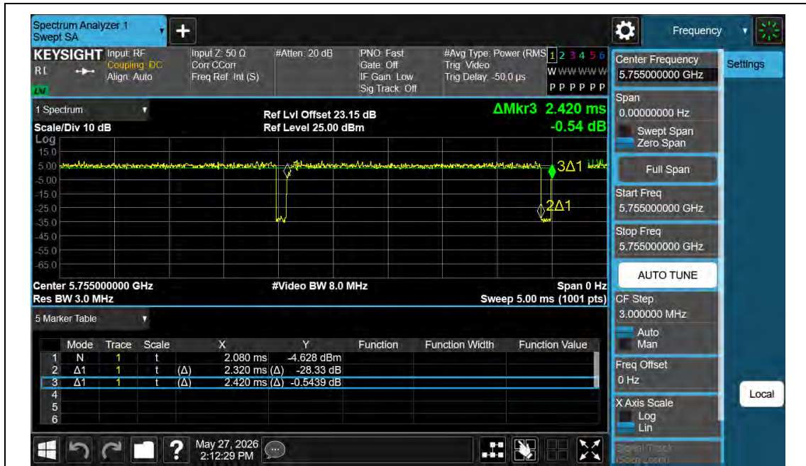
NTNV-11N40MIMO-Ant2-5755
