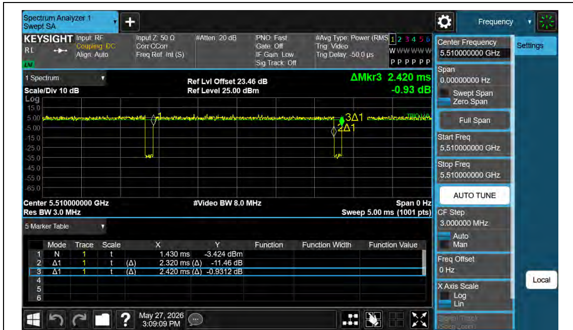
NTNV-11AC40MIMO-Ant2-5510
