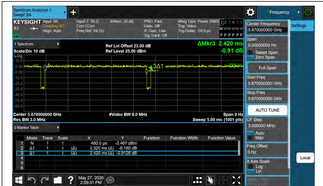
NTNV-11N40MIMO-Ant2-5670
