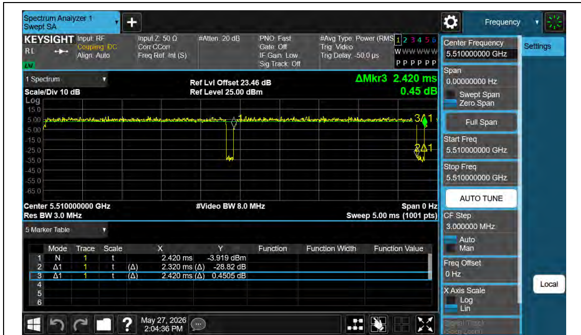
NTNV-11N40MIMO-Ant2-5510
