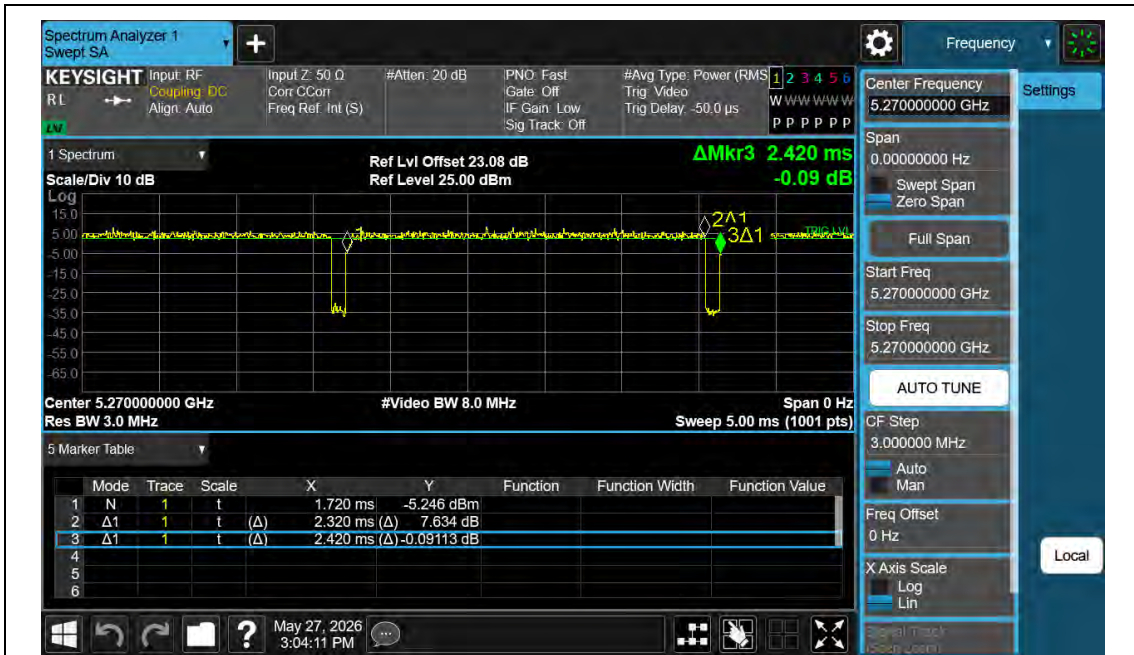
NTNV-11AC40MIMO-Ant2-5270
