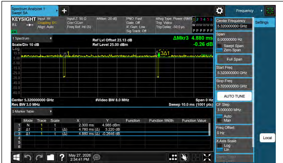
NTNV-11AC20MIMO-Ant2-5320
