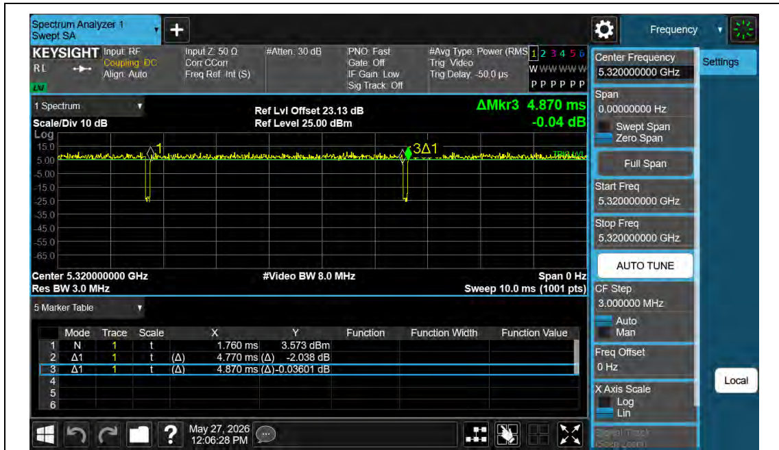
NTNV-11N20MIMO-Ant2-5320
