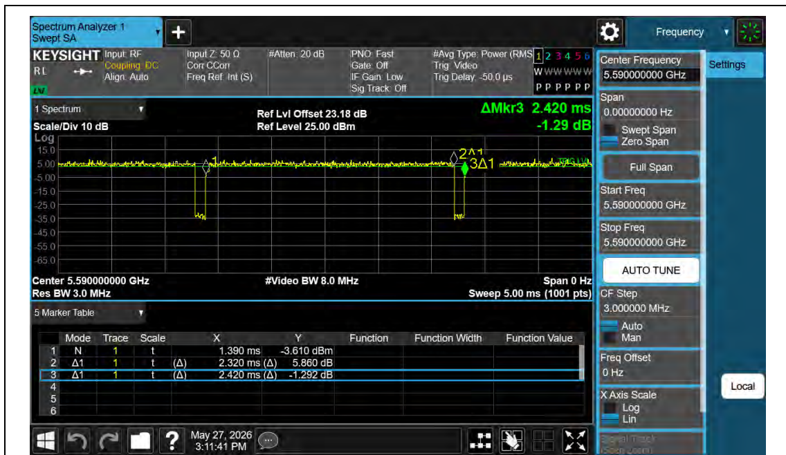
NTNV-11AC40MIMO-Ant2-5590
