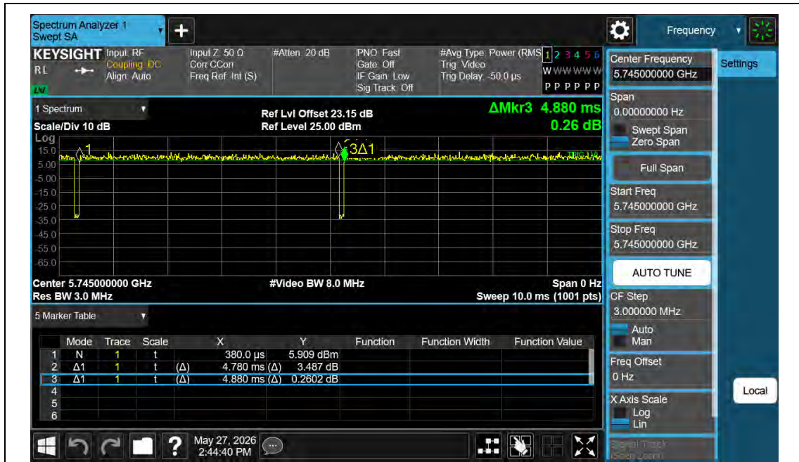
NTNV-11AC20MIMO-Ant2-5745
