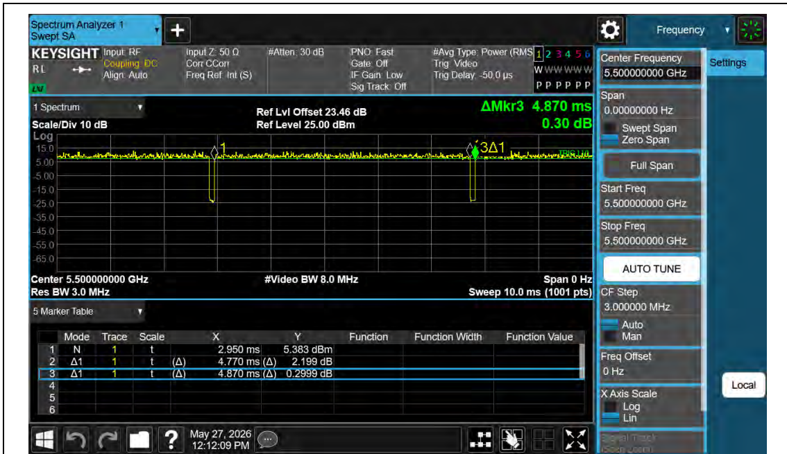
NTNV-11N20MIMO-Ant2-5500
