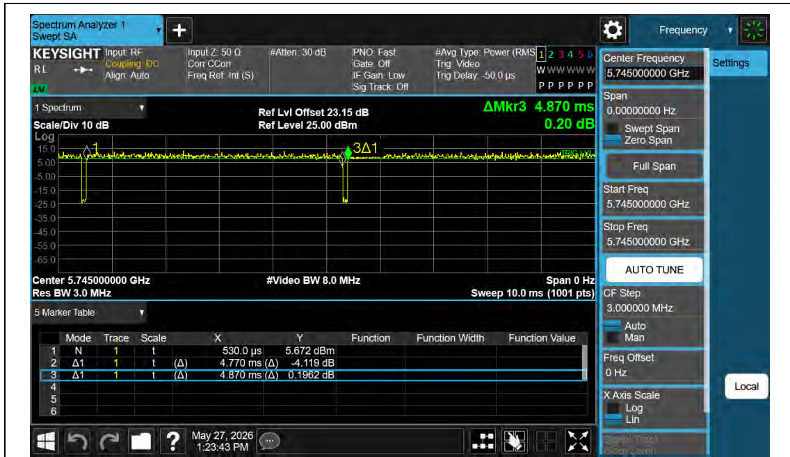
NTNV-11N20MIMO-Ant2-5745
