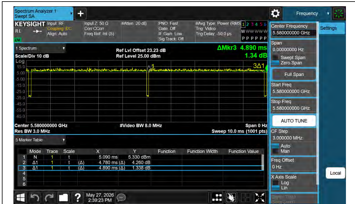
NTNV-11AC20MIMO-Ant2-5580
