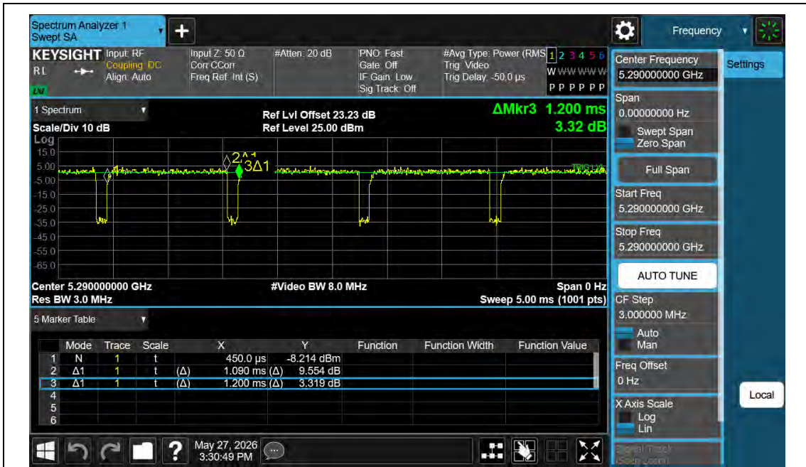
NTNV-11AC80MIMO-Ant2-5290
