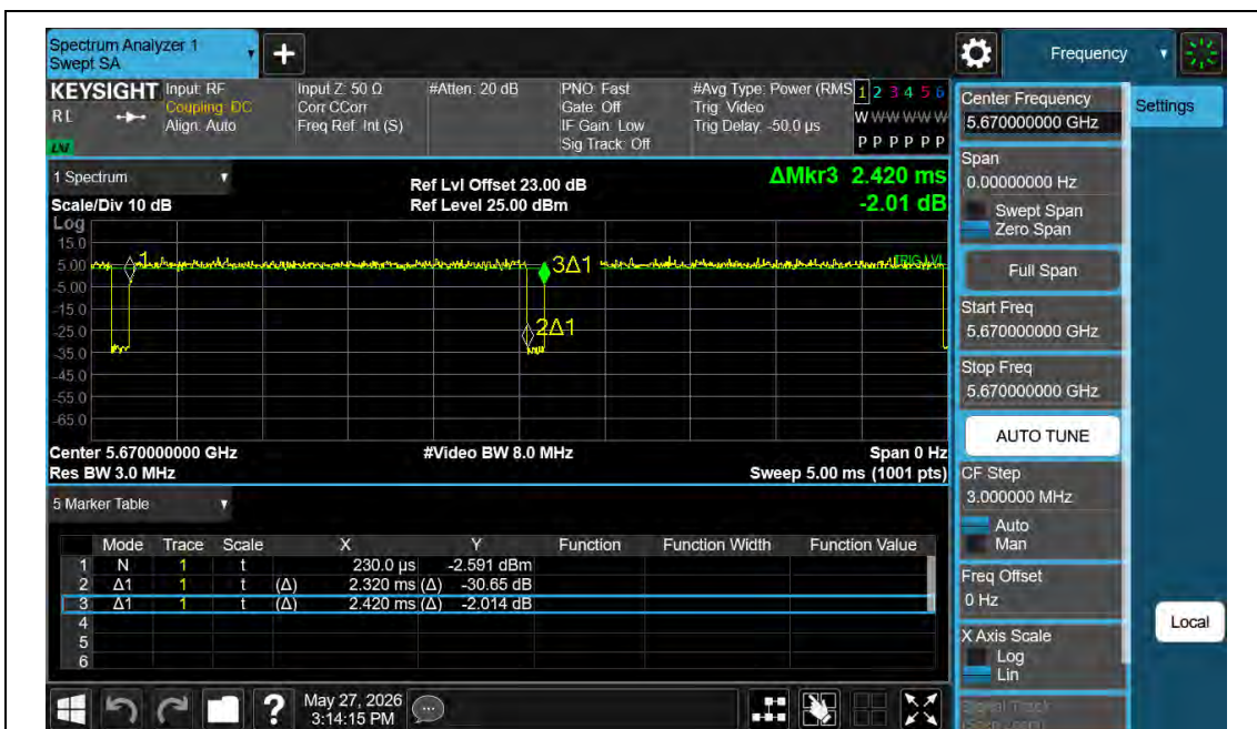
NTNV-11AC40MIMO-Ant2-5670
