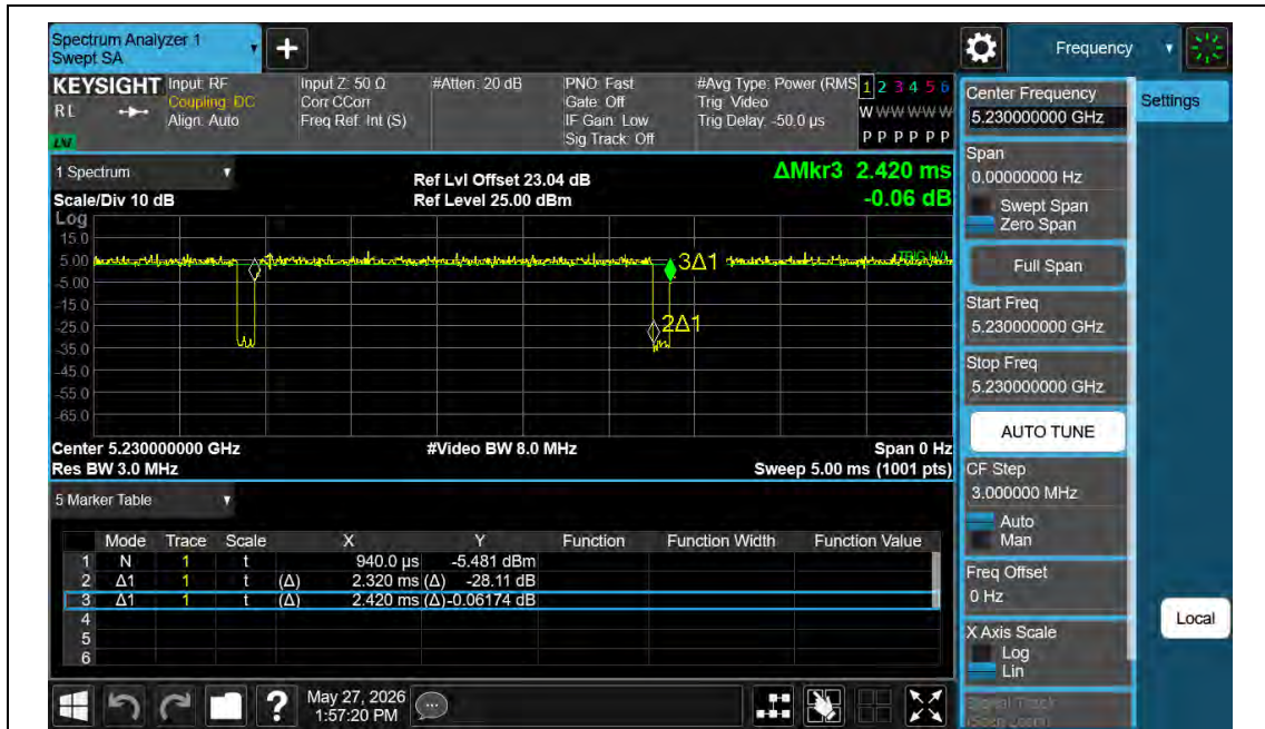
NTNV-11N40MIMO-Ant2-5230
