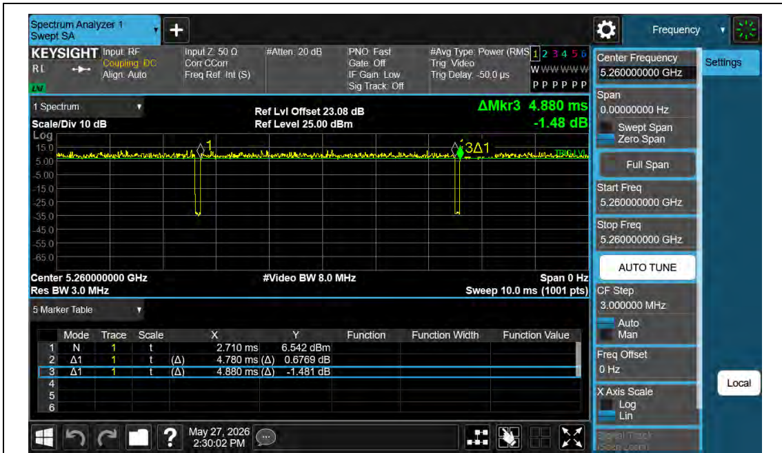
NTNV-11AC20MIMO-Ant2-5260
