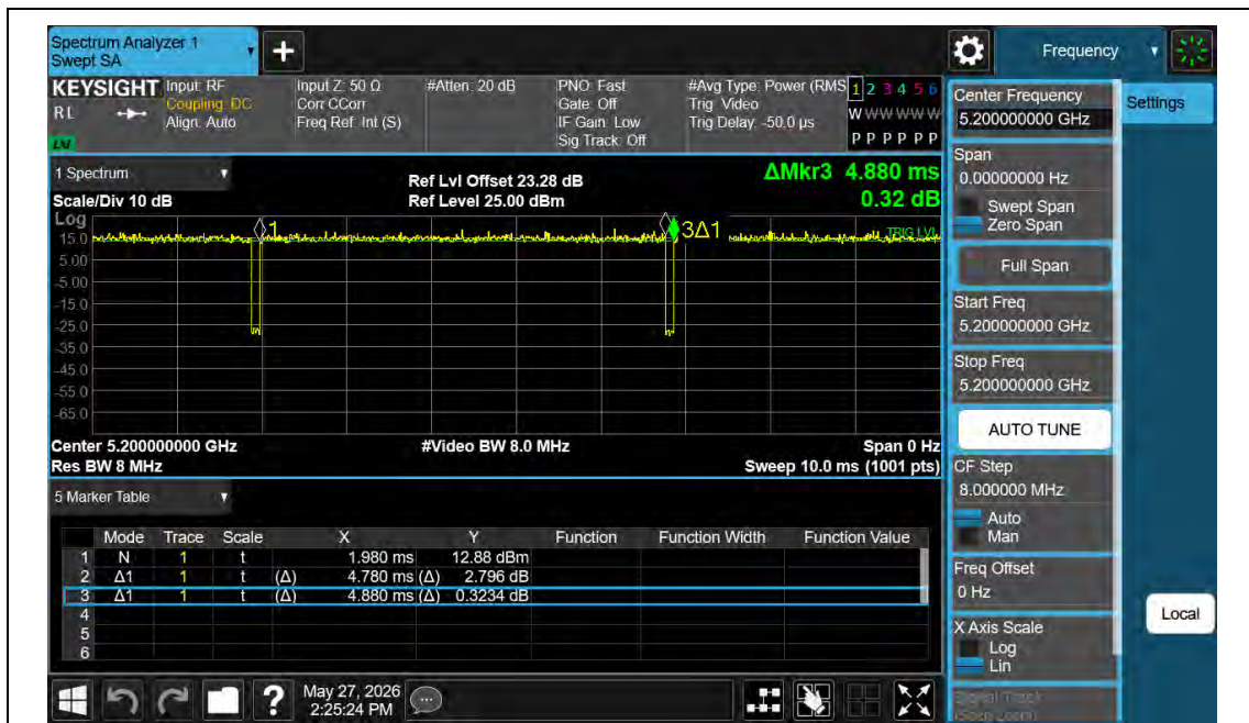
NTNV-11AC20MIMO-Ant2-5200
