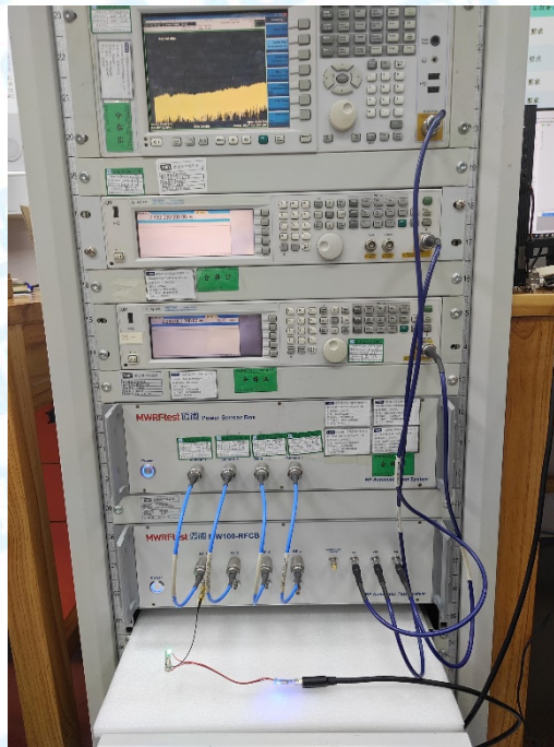
Photo of Setup for Conducted Measurement ----Left
