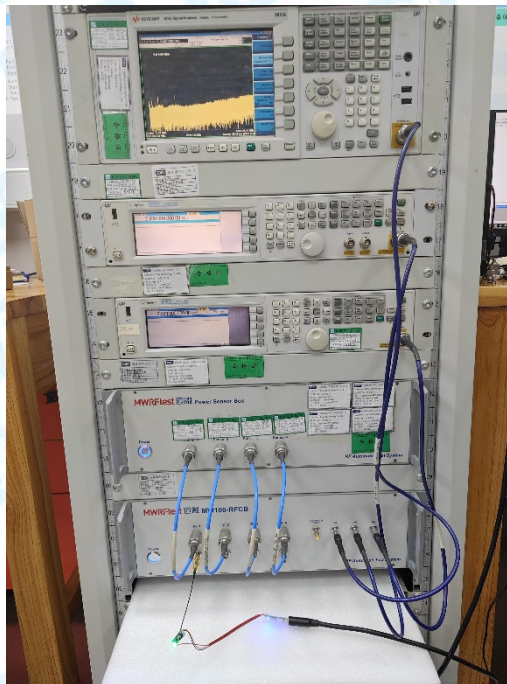
Photo of Setup for Conducted Measurement ----Right
