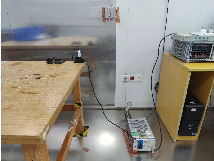
Photo of Setup for Conducted Measurement ----Left
