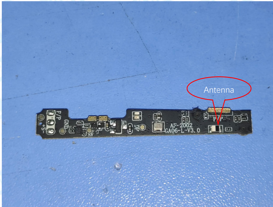
Photo 14 Appearance of PCB ----Left
